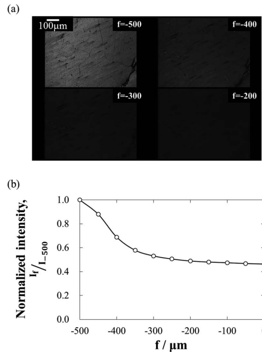
Fig. B4 (a) The laser micrographs of pure Ag under various focal positions and (b) normalized intensity of experimentally observed images as a function of focal positions “ f ” estimated by ImageJ software.
