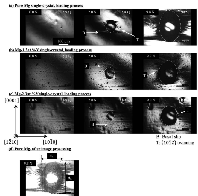
Fig. 2 The in-situ images of (a) pure Mg, (b) Mg-1.3 at.% Y and (c) Mg-2.3 at.% Y single-crystals during loading process with n_r/n_t=0.85 . (d) An in-situ image processed to measure the major and the minor diameters of the indent on pure Mg single-crystal at 9.8 N.
