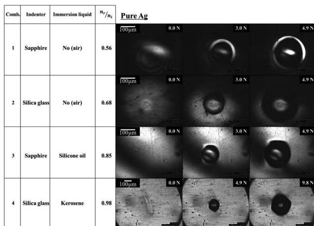
Fig. B2 The in-situ images of various combinations of the indenter and the immersion liquid on pure Ag.
