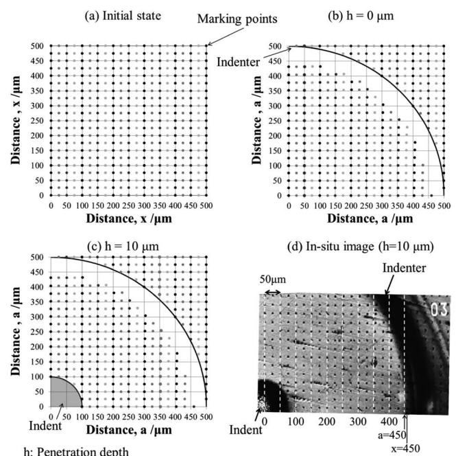
Fig. B3 The theoretical images of (a) initial state, (b) h=0 and (c) h=10 , and (d) the experimental in-situ image of pure Ag with n_r/n_i=0.98 . The marking points were plotted every 25\text{ }\mu\text{m} .
