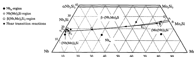
Fig. 1 The proposed liquidus surface projection of Nb–Mo-rich zone of the Nb–Mo–Si ternary system. The various marks in this diagram represent the alloy compositions investigated in this study.
