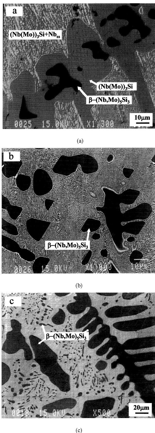
Fig. 3 BEI micrographs for compositions lying on \beta\text{-(Nb, Mo)}_5\text{Si}_3 -rich side, showing typical microstructures of (a) \text{L} + \beta\text{-(Nb, Mo)}_5\text{Si}_3 \rightarrow (\text{Nb}(\text{Mo}))_3\text{Si} peritectic reaction (Nb-20Si-1Mo), (b) (\text{Nb}(\text{Mo}))_3\text{Si}\text{--Nb}_{\text{ss}} eutectic reaction (Nb-20Si-30Mo), and (c) \beta\text{-(Nb, Mo)}_5\text{Si}_3\text{--}(\text{Mo}(\text{Nb}))_3\text{Si} eutectic reaction valley (Nb-30Si-69Mo).
