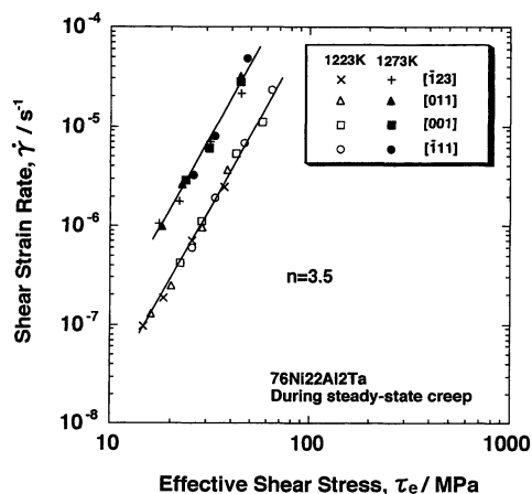
Fig. 5 Steady-state shear strain rate versus effective shear stress relations in the full logarithmic scale.
