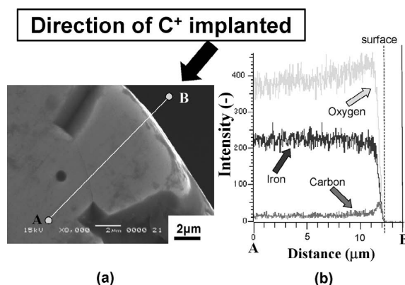
Fig. 6. Results of EDS analysis on the cross section of hematite (Imp-1). (a) SEM image (b) line analysis from the point A to B.
