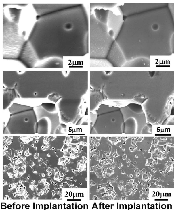
Fig. 3. Result of SEM observation of hematite surface before and after implantation (Imp-1).
