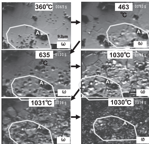
Fig. 15. In situ observation of the heating up experiment under argon atmosphere by laser microscope (Imp-1).
