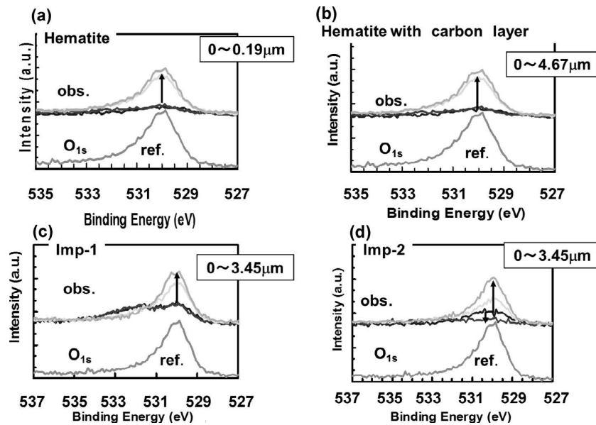
Fig. 10. Variation of peak profiles of O 1s .
