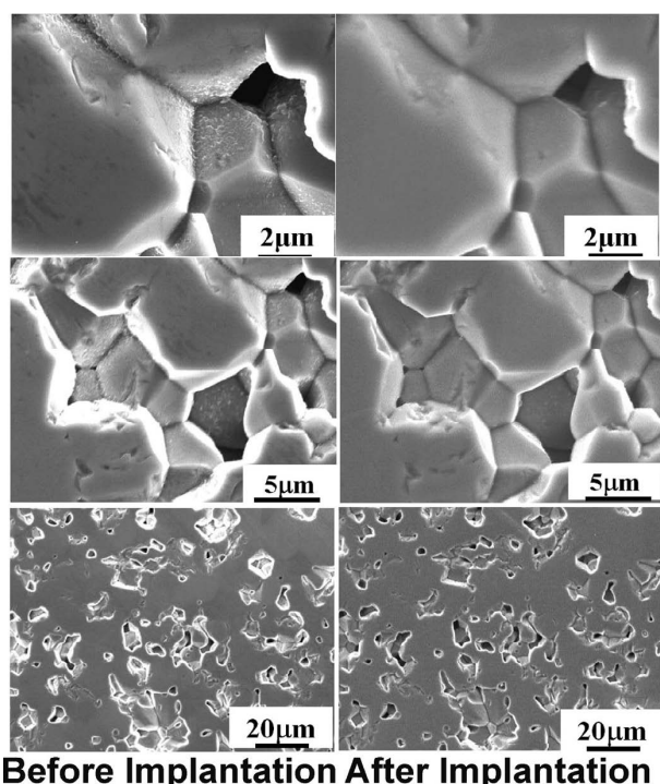
Fig. 4. Result of SEM observation of hematite surface before and after implantation (Imp-2).
