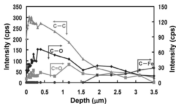
Fig. 14. Variation of intensities for the C-C , C-O , C=O and C-Fe bond in C_{1s} as a function of the depth from surface (Imp-2).
