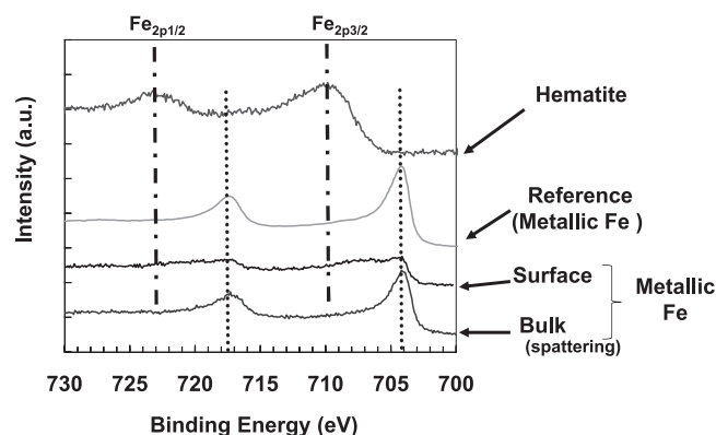
Fig. 8. Comparison of peak profiles of \text{Fe}_{2p1/2} and \text{Fe}_{2p3/2} in Hematite and Metallic iron.
