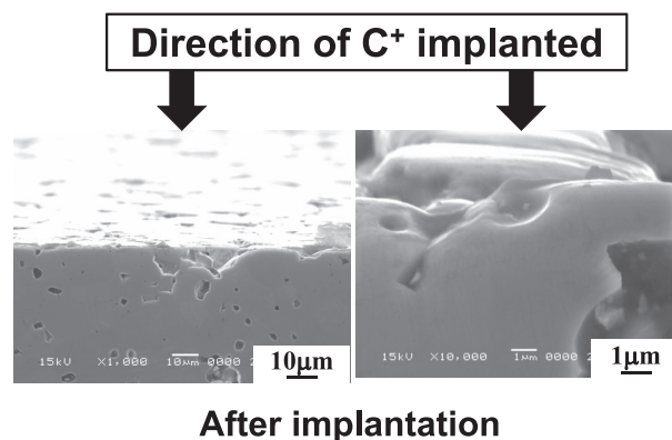
Fig. 5. SEM image of cross section of hematite (Imp-1).
