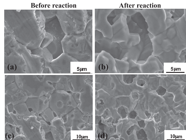
Fig. 16. Microstructure of the surface of Imp-1 before and after heating up experiment.
