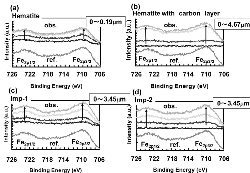
Fig. 9. Variation of peak profiles of \text{Fe}_{2p1/2} and \text{Fe}_{2p3/2} peaks.
