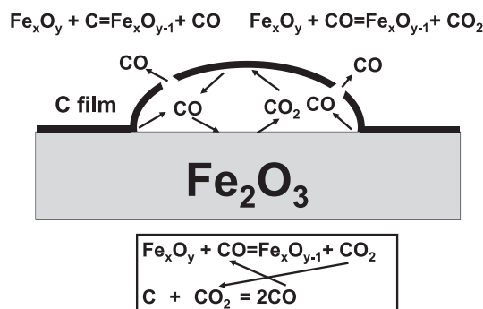
Fig. 17. Illustration of the mechanism of reaction between \text{Fe}_2\text{O}_3 and carbon film. 5)
