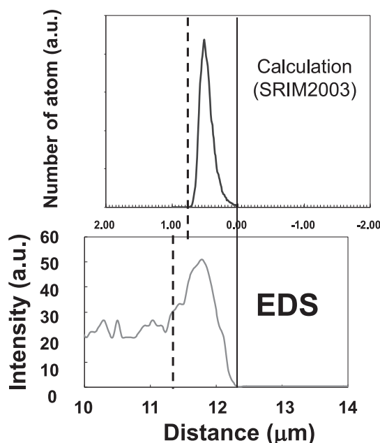
Fig. 7. Comparison of the implanted carbon distribution in hematite between experiment and calculation (SRIM2003).
