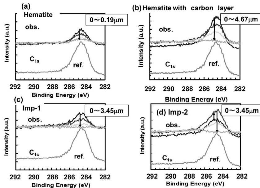
Fig. 11. Variation of peak profiles of C 1s .
