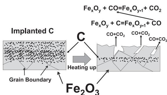
Fig. 18. Illustration of the mechanism of reaction of \text{Fe}_2\text{O}_3 and carbon implanted.
