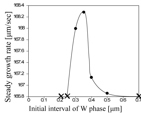
Fig. 8. The size dependency of growth rate of the W phase (●: stable lamellar growth, ×: unstable lamellar growth, —: fitted curve). The W phase grows stable with cooperative larger than 0.30 \mu\text{m} . The W phase with initial interval less than 0.30 \mu\text{m} grows resulting interval of 0.33 \mu\text{m} for stable growth.
