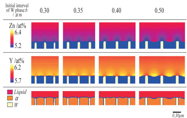
Fig. 9. The stable lamellar growth at 0.050 s. In case that the initial interval length of the W phase, b , is larger than 0.3 μm, the lamellar spacings keep the initial interval length.
