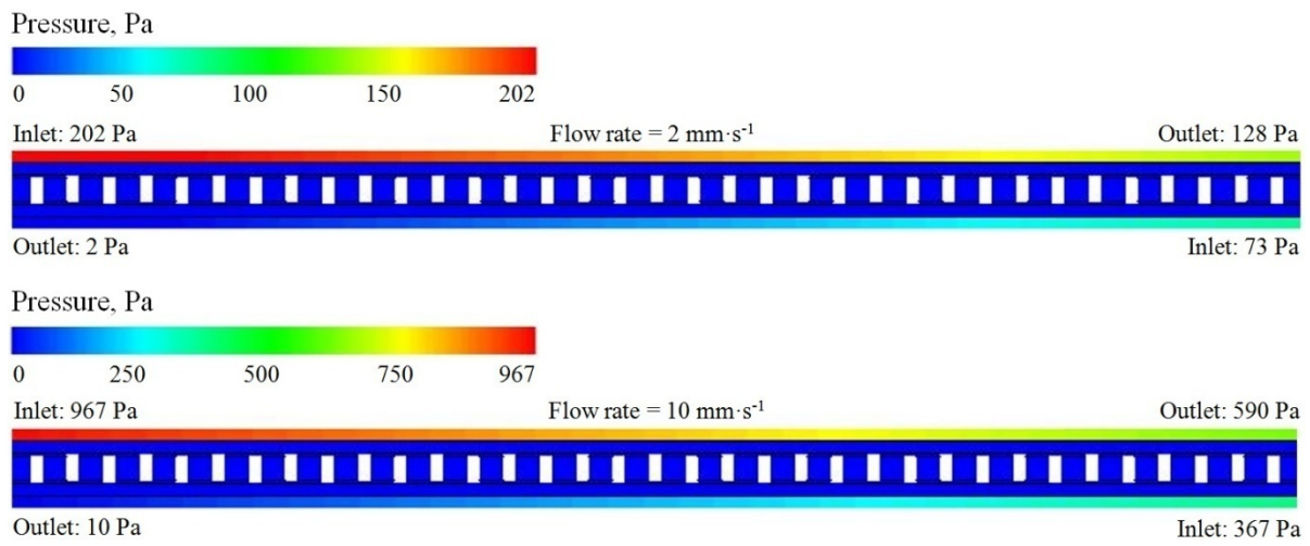
Figure 7 Pressure in channels of TE module.
