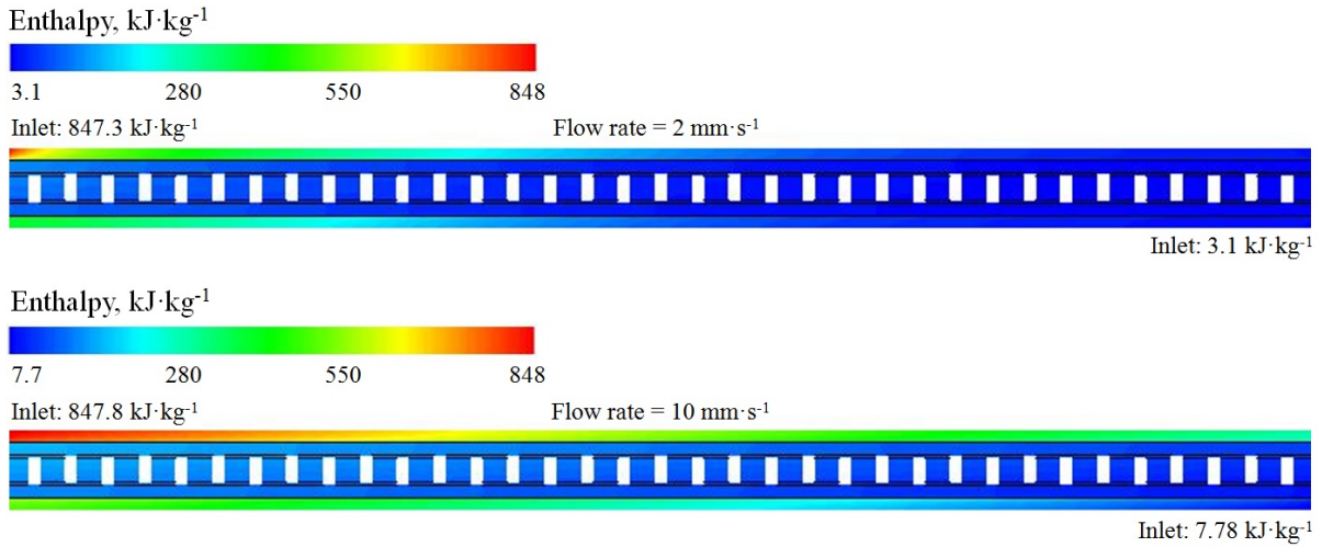
Figure 9 Enthalpy on TE module.
