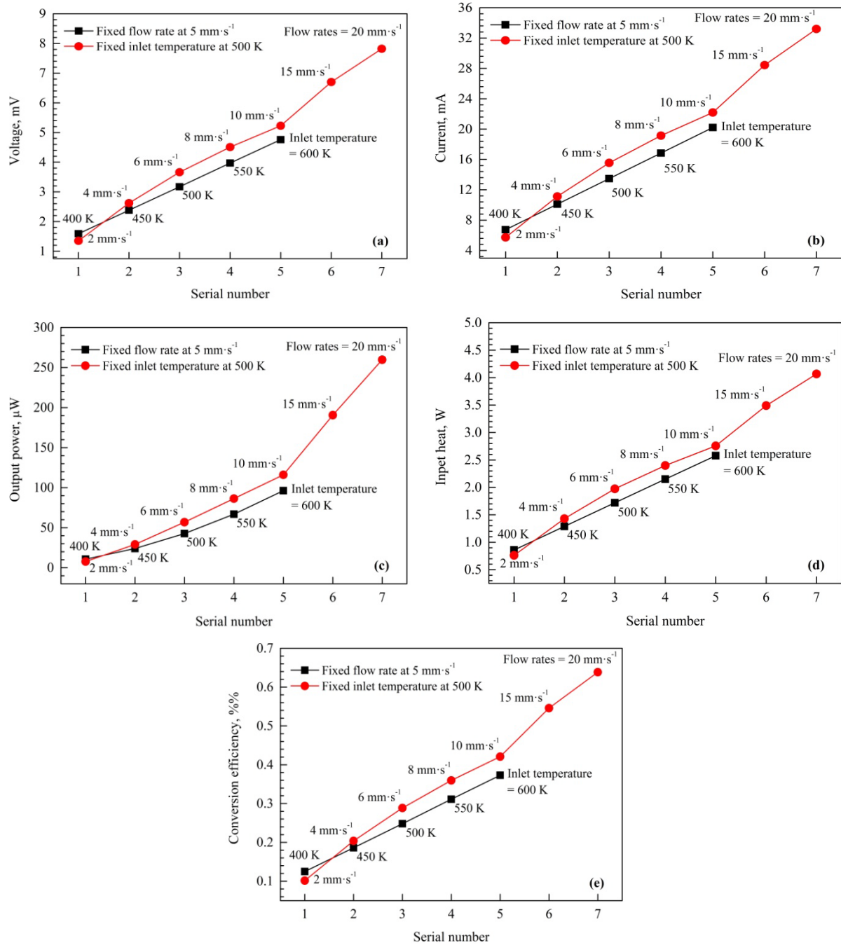
Figure 4 Stable performance comparison of TE module: (a) voltage, (b) current, (c) output power, (d) input heat, and (e) conversion efficiency.
