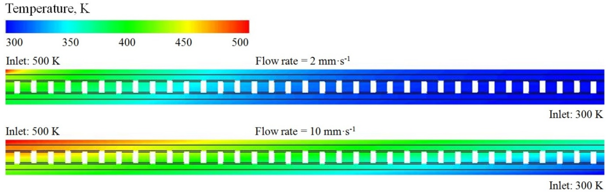
Figure 5 Distribution of temperature on TE module.
