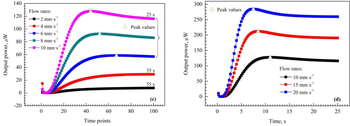
Figure 3 Transient performance of TE module:
