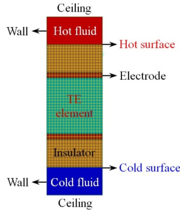
Figure 2 Cross-section design of TE module for finite-element analysis.
