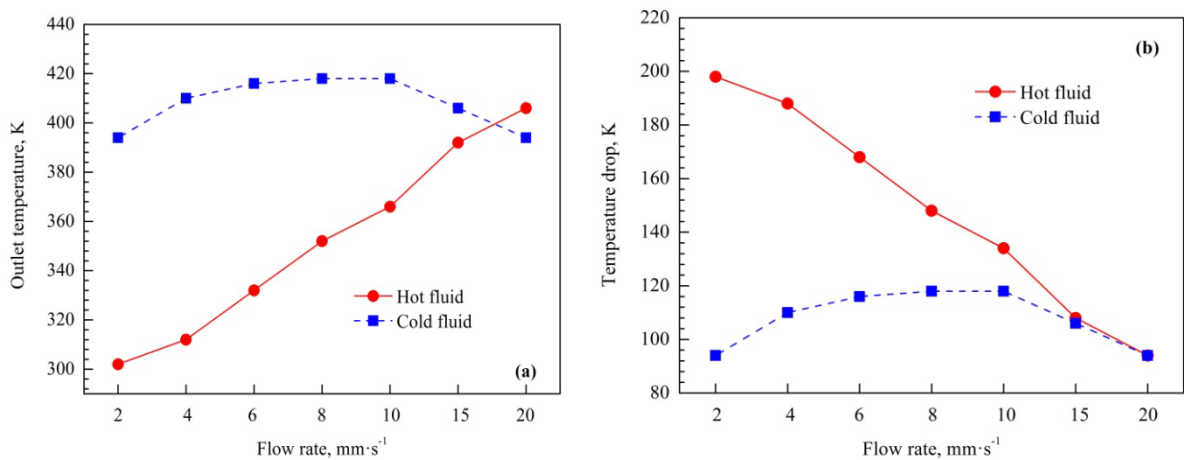
Figure 6 Temperature of thermal fluids in channel: (a) outlet temperature and (b) temperature drop from inlet to outlet.
