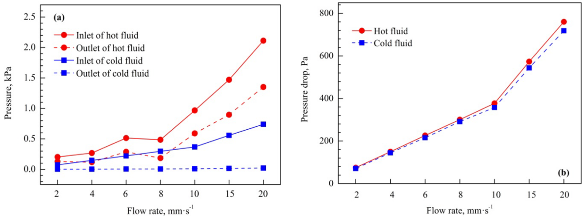
Figure 8 Pressure of thermal fluids in channel:
