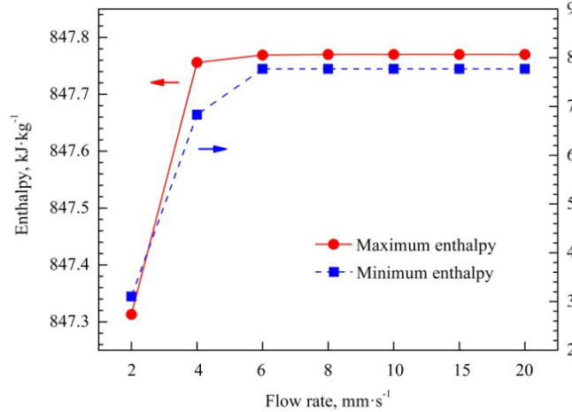
Figure 10 Enthalpy extrema of TE module.
