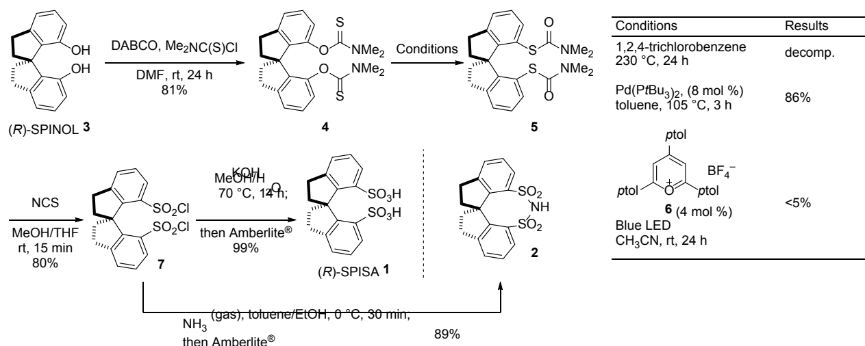
Scheme 1. Synthesis of ( R )-SPISA 1 and disulfonimide 2 from ( R )-SPINOL 3 .
