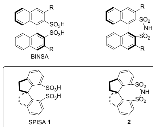
Figure 1. Structures of BINSA (1,1'-binaphthyl-2,2'-disulfonic acid), SPISA (1,1'-spirobiindane-7,7'-disulfonic acid), and their disulfonimide derivatives
