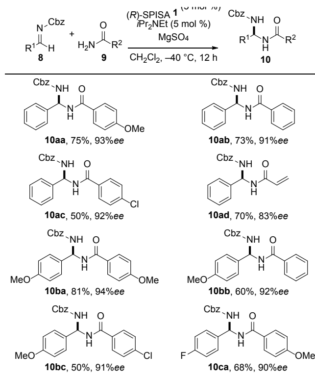
Scheme 2. Substrate scope of (R)-SPISA 1 -catalyzed asymmetric aminalization.
