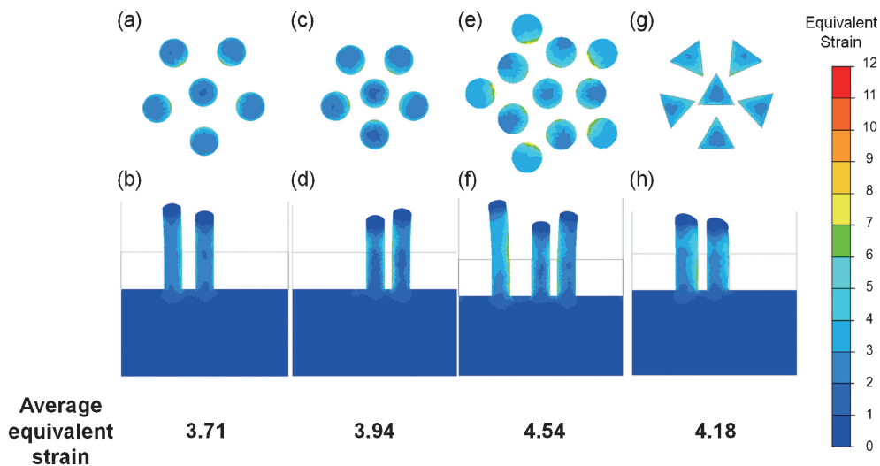
Fig. 13 The distributions of equivalent strain after extrusion of 10 mm with (a) and (b) 6-hole die, (c) and (d) 6-centered-hole die, (e) and (f) 11-hole die and (g) and (h) triangle-hole die. Figures (a), (c), (e) and (g) show the cross section of the extrudates directly above the die, and figures (b), (d), (f) and (h) show the longitudinal section of the extrudates, which passes through the center of the die. The average equivalent strains were measured on the observed cross sectional plane.
