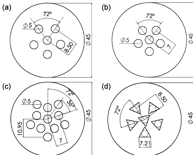
Fig. 12 Die designs for the simulations; (a) 6-hole die, (b) 6-centered-hole die, (c) 11-hole die and (d) triangle-hole die, (All dimensions are in mm).
