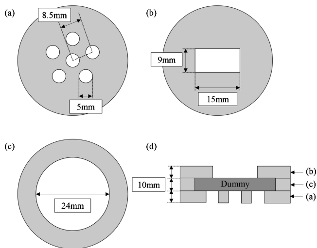
Fig. 2 Schematic image of dies: (a) a strain-giving die, (b) a shape-giving die, (c) a spacer and (d) a heteromorphic die, (The diameter and height of all dies are 45 mm and 10 mm, respectively).
