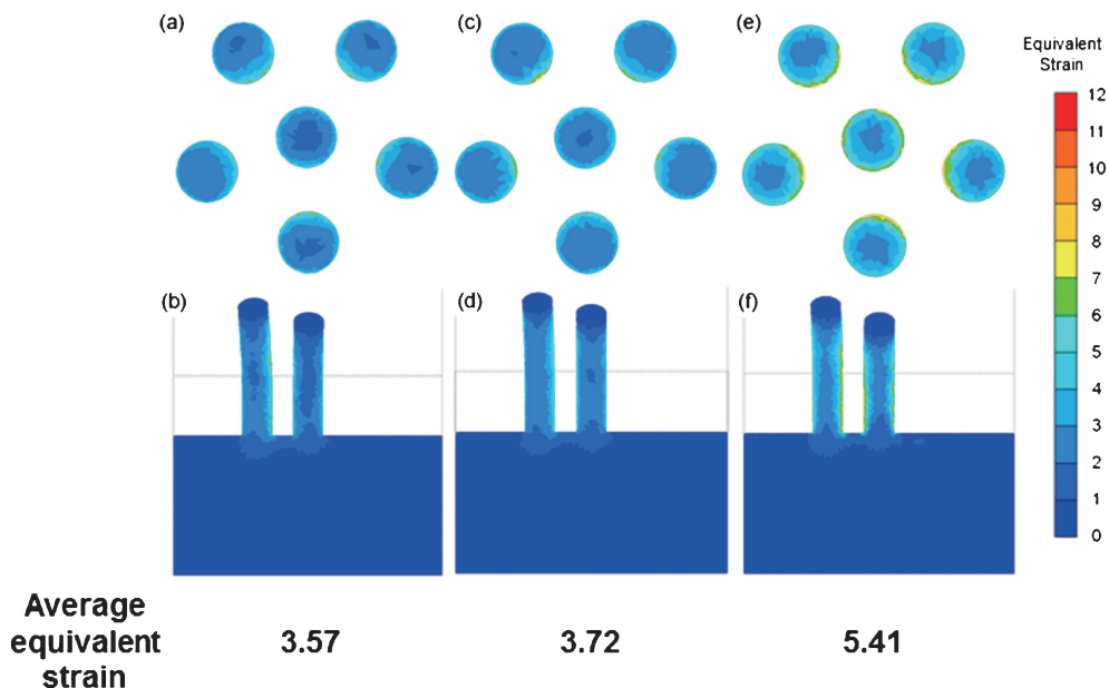
Fig. 14 The distributions of equivalent strain after extrusion of 10 mm with various friction conditions at the interface between the metal and the die; (a) and (b) low friction, (c) and (d) medium friction and (e) and (f) high friction conditions. Figures (a), (c) and (e) show the cross section of the extrudates directly above the die, and figures (b), (d) and (f) show the longitudinal section of the extrudates, which passes through the center of the die. The average equivalent strains were measured on the observed cross sectional plane.
