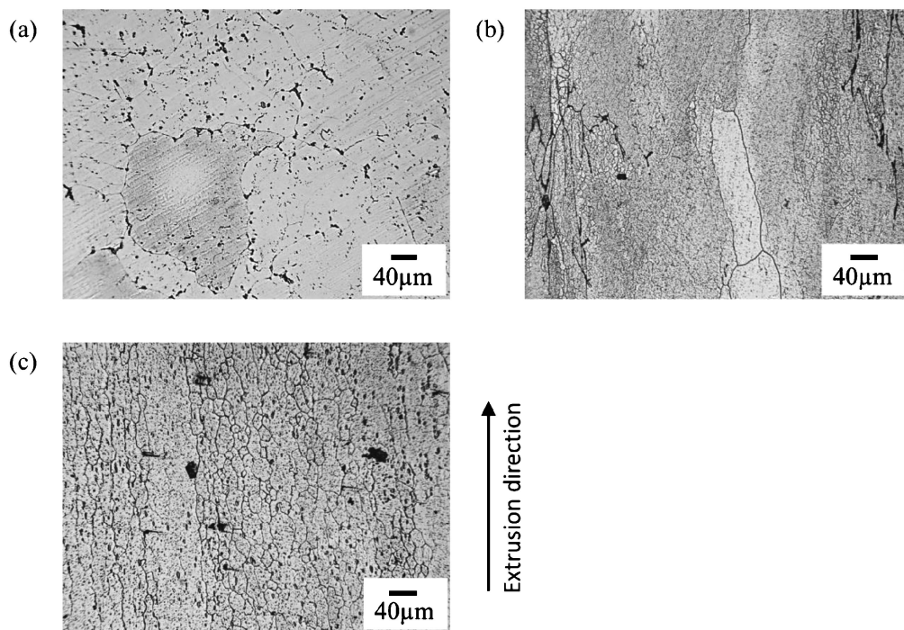
Fig. 4 Microstructures of Al-Cu alloy: (a) sample before extrusion, (b) sample extruded with the shape-giving die, (c) sample extruded with the heteromorphic die.
