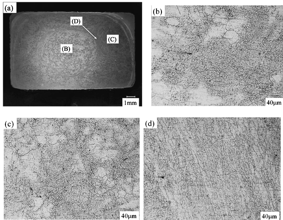
Fig. 3 Microstructures observed on a cross section of the rectangular bar extruded using a heteromorphic die. (a) Full picture of the cross section at a low magnification. (b), (c) and (d) High magnification pictures showing points (B), (C) and (D) indicated in Fig. 3 (a), respectively.
