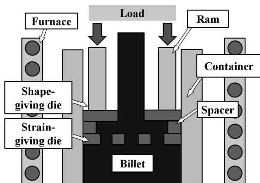
Fig. 1 Schematic illustration of hot extrusion equipment.
