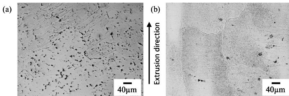
Fig. 6 Microstructures of Al-Cu alloy: (a) annealed billet, (b) annealed extruded sample with the shape-giving die.
