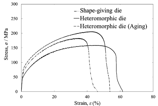
Fig. 9 Results of tensile tests at room temperature for aging-treated extruded sample with heteromorphic die and as-extruded samples.
