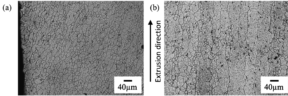
Fig. 10 Microstructures of Al-Cu alloy: (a) near the wall of the die hole, (b) center of the die hole.
