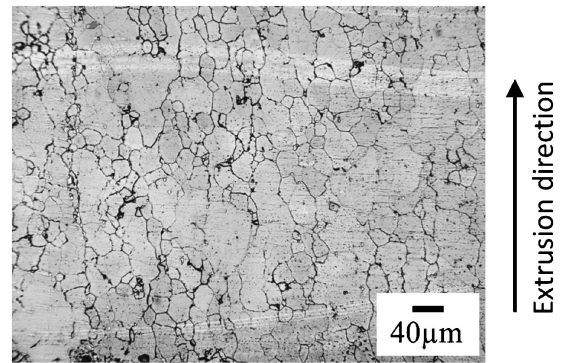
Fig. 8 A microstructure of the aging-treated extruded sample with a heteromorphic die.
