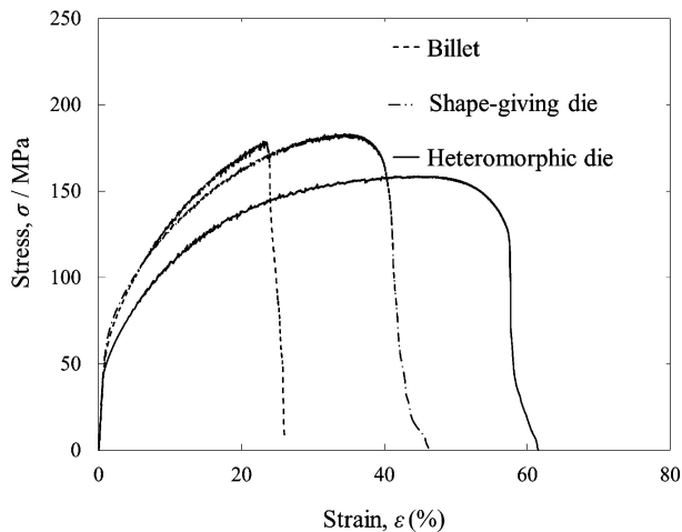
Fig. 7 Results of tensile tests at room temperature for annealed samples and extruded sample with a heteromorphic die.
