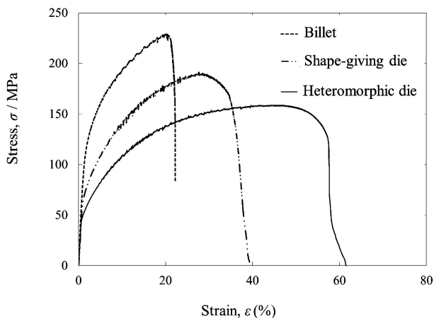
Fig. 5 Results of tensile tests at room temperature for the billet and as-extruded samples.
