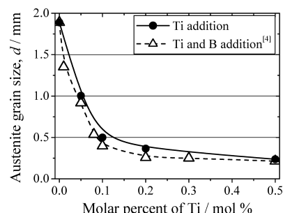
Fig. 2. Effects of Ti addition on \gamma grain size. The dashed line represents the results of Ti and B additions reported in the previous paper. 4)
