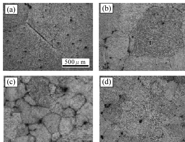
Fig. 1. \gamma grain structures (a) without Ti addition, (b) with addition of 0.05 mol% Ti, (c) with addition of 0.1 mol% Ti, and (d) with addition of 0.5 mol% Ti.
