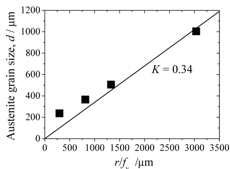
Fig. 11. Relation between r/f_v of Ti(C,N) and \gamma grain size.
