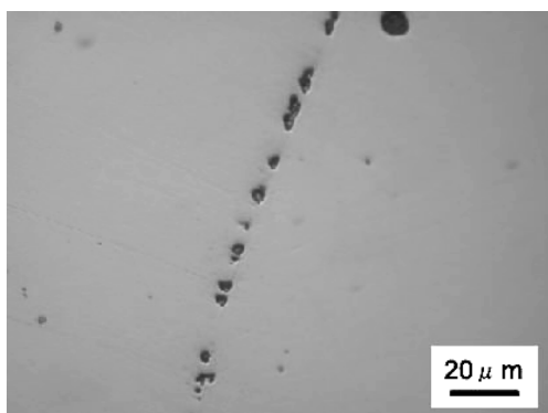
Fig. 5. Ti(C,N) particles existing at \gamma grain boundary.
