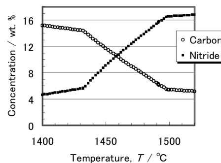
Fig. 7. Temperature dependence of C and N compositions in Ti(C,N) phase calculated by CALPHAD method for the sample with 0.45 wt% C, 0.0037 wt% N and 0.2 mol% Ti.
