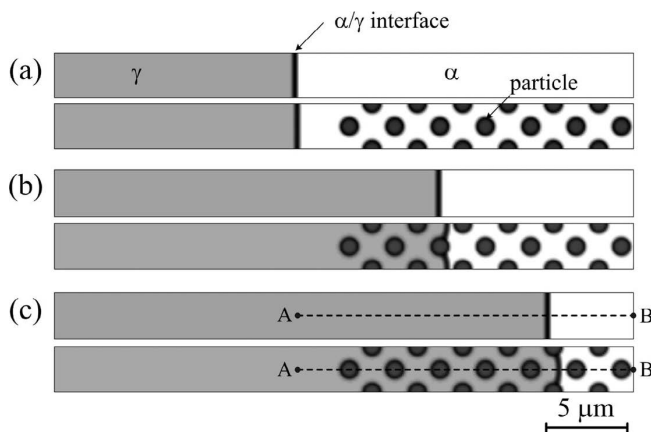
Fig. 7. Migration behavior of \alpha/\gamma interface compared in samples without and with particles ( r=0.5 \mu\text{m} , f_v=0.20 ) at different time steps of (a) t=0 , (b) t=22.5 \text{ s} and (c) t=56.0 \text{ s} . Grey area, bright area and black circular area correspond to \gamma , \alpha phases and particles, respectively. (The dashed lines AB in (c) will be used to discuss the carbon concentration along them later.)
