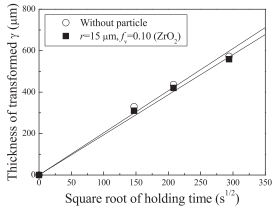
Fig. 4. Thickness of newly transformed \gamma phase with varied holding time at 1133 K in samples without and with \text{ZrO}_2 particles with r=15\ \mu\text{m} , f_v=0.10 .
