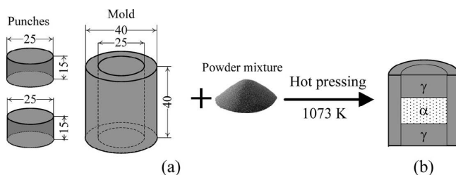
Fig. 1. Schematic drawing of (a) mold and punches produced from S45C steel rod and mixture of iron powder and insoluble particles and (b) longitudinal section of \gamma/\alpha diffusion couple sample after hot-pressing (unit: mm).
