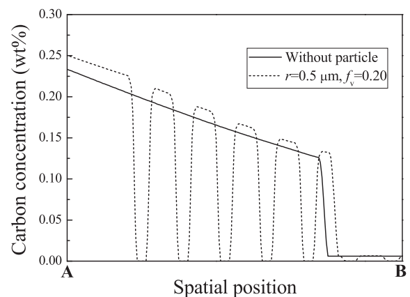
Fig. 9. Carbon concentration profile in samples without particle and having particles with r=0.5 \mu\text{m} and f_v=0.20 at time step of 56.0 s along the dashed lines shown in Fig. 7(c).
