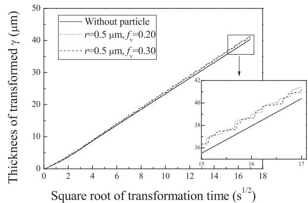
Fig. 8. Time dependences of thickness of newly transformed \gamma phase in samples without and with particles obtained from simulation ( \sigma_{\alpha/\gamma}/\sigma_{\alpha/\beta}/\sigma_{\gamma/\beta}=1.0/1.0/1.0 \text{ J/m}^2 ). The enlarged figure corresponds to the indicated rectangle area.
