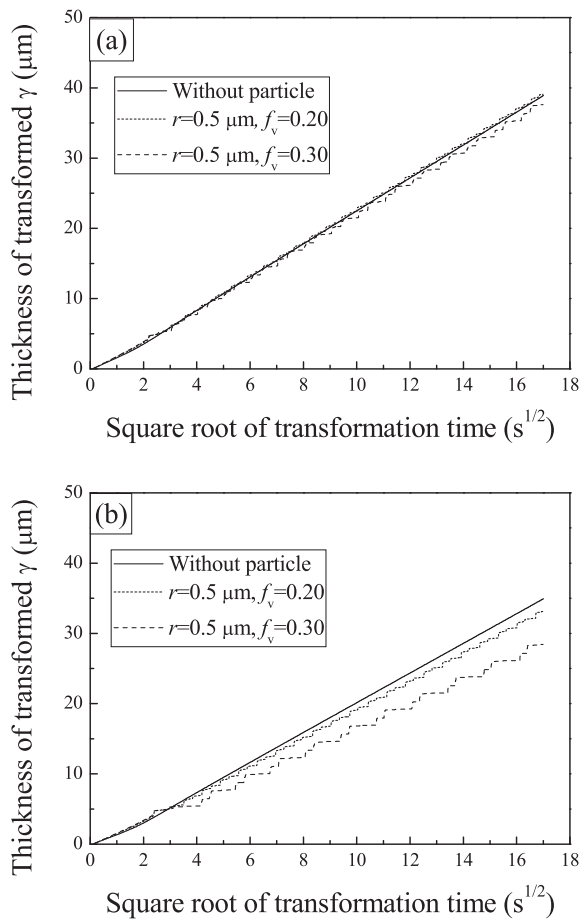
Fig. 10. Time dependences of thickness of transformed \gamma phase obtained from simulation using higher interfacial energy, \sigma_{\alpha/\gamma} . (a) \sigma_{\alpha/\gamma}/\sigma_{\alpha/p}/\sigma_{\gamma/p}=1.8/1.0/1.0 J/m 2 (b) \sigma_{\alpha/\gamma}/\sigma_{\alpha/p}/\sigma_{\gamma/p}=4.0/1.0/1.0 J/m 2 .
