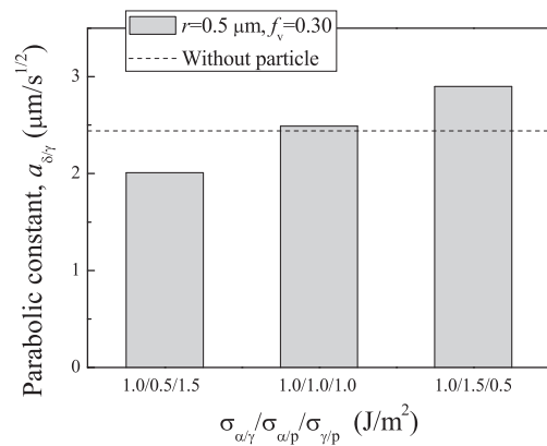
Fig. 11. Effect of unequal \sigma_{\alpha/p} and \sigma_{\gamma/p} on parabolic constants with a fixed \sigma_{\alpha/\gamma}=1.0 J/m 2 in sample having particles with r=0.5 \mu\text{m} and f_v=0.30 . The dashed line shows the case of without particle for a comparison.
