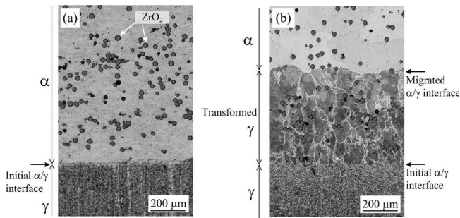
Fig. 3. Microstructures on the longitudinal section of sample having \text{ZrO}_2 particles with r=15\ \mu\text{m} and f_v=0.10 , quenched after (a) hot-pressing at 1073 K and (b) holding at 1133 K for 24 hrs.
