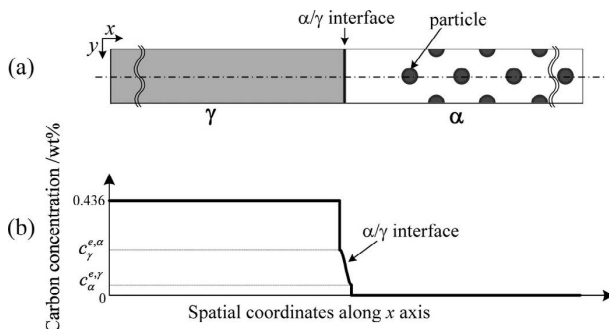
Fig. 2. Schematic drawing of (a) phase field simulation system and (b) initial carbon concentration profile along the center line indicated in (a).
