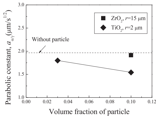
Fig. 6. Parabolic constants of \alpha/\gamma interface regressed from experimental results.
