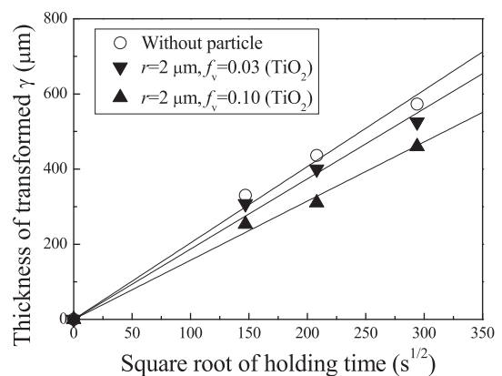
Fig. 5. Thickness of newly transformed \gamma phase with varied holding time at 1133 K in samples without and with \text{TiO}_2 particles with r=2\ \mu\text{m} , f_v=0.03 and 0.10 .
