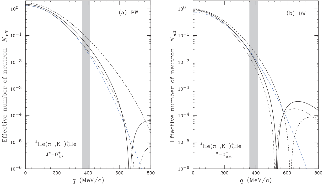
FIG. 6. Calculated effective number of nucleons N_{\text{eff}}^{0+} for 0_{\text{g.s.}}^{0+} in {}^4_\Lambda\text{He} via the {}^4\text{He}(\pi^+, K^+) reaction with (a) the plane-wave (PW) and (b) the distorted-wave (DW) approximations, as a function of the momentum transfer q . Solid, dashed, and dotted curves denote the results obtained from the Isle, SG, and HO potentials, respectively. Long-dashed curves denote the results in the eikonal-oscillator approximation with \bar{\sigma} = 30 mb. The half-tones denote the region of q = 360\text{--}410 MeV/ c corresponding to \theta_{\text{lab}} = 0^\circ\text{--}12^\circ at p_\pi = 1.05 MeV/ c .
