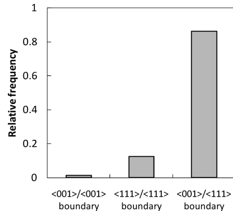
Fig. 9. Frequency of the three types of boundaries fractured in the creep test.
