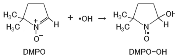
Fig. 1. DMPO-OH formation from DMPO and \cdot\text{OH} .
