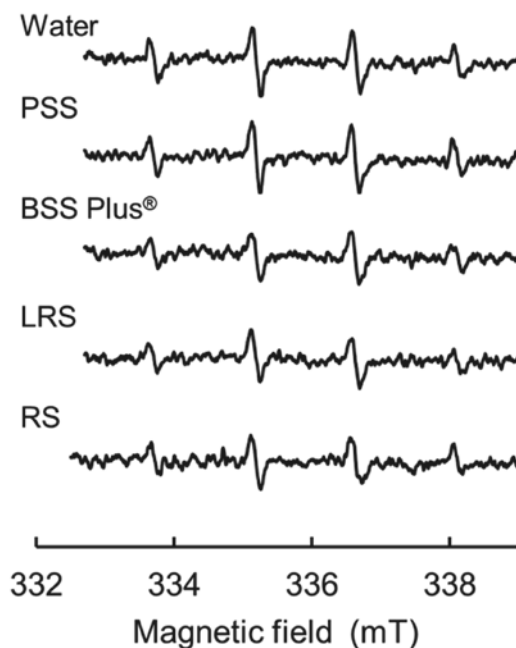
Fig. 2. Representative ESR signals consisted of four lines with a ratio of 1:2:2:1 after sonication in various solutions. The hyperfine coupling constants were estimated as a_N = a_H = 1.49 mT using computer simulation, and the spectra were assigned to DMPO-hydroxyl radical adducts (DMPO-OH).
