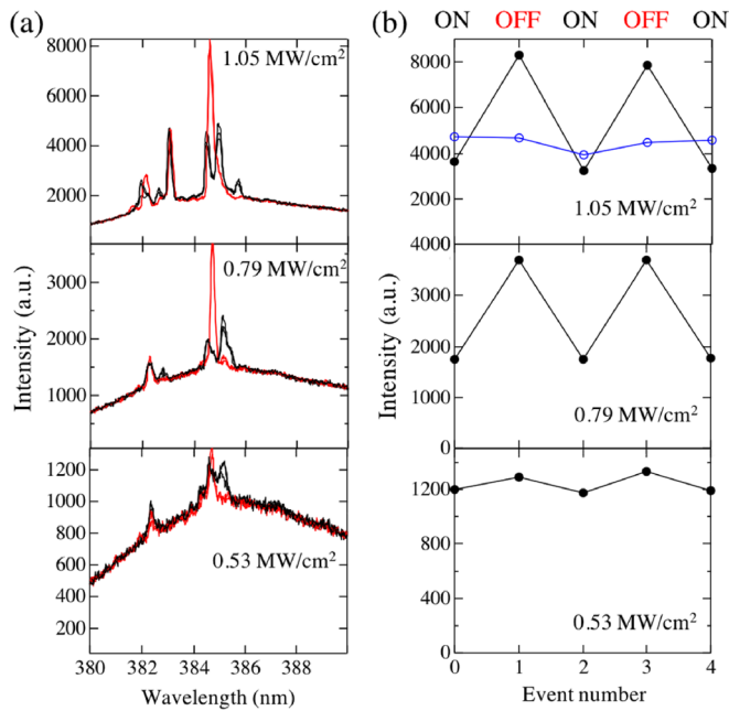
FIG. 3. Magnetic field dependence of (a) emission spectra and (b) peak intensities. The excitation intensities were fixed at 1.05, 0.79, and 0.53 MW/cm 2 . The black and red lines in (a) indicate spectra in the presence and absence of the magnetic field. These are the same data shown in Figs. 2(a) and 2(b). In (b), the black circles indicate the peak intensities at 384.7 nm and the blue circles indicate the peak intensities at 382.8 nm [marked by the circle and star in Fig. 2(a)].
