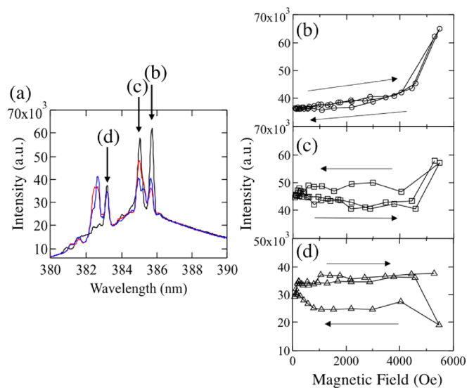
FIG. 5. Magnetic field dependence of (a) emission spectra and (b)–(d) peak intensities when the excitation intensity was fixed at 1.15 MW/cm 2 . The red, blue, and black lines in (a) indicate the emission spectra with a magnetic field of 0, 2900, and 5300 Oe, respectively. The circles, squares, and triangles in (b)–(d) denote the peak intensities indicated by arrows in (a). The arrows in (b)–(d) indicate the directions of magnetic field intensity change.
