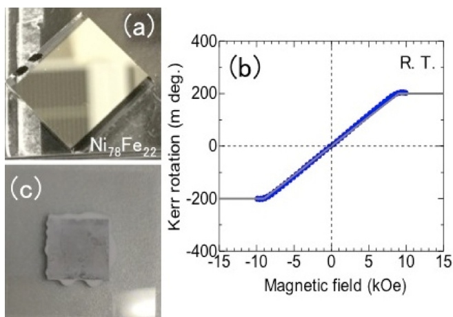
FIG. 1. (a) Image and (b) Kerr rotation of the NiFe thin film (35 nm). A magnetic field was applied perpendicular to the film plane, and Kerr rotation was detected from laser light reflection at 405 nm. (c) Image of the ZnO nanoparticle film cast on the NiFe film.
