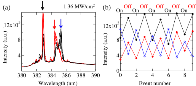
FIG. 4. Magnetic field response of (a) emission spectra and (b) peak intensities. The excitation intensity was fixed at 1.36 MW/cm 2 . The black and red lines in (a) indicate the spectra with and without the magnetic field. The black, red, and blue circles in (b) denote the peak intensities, indicated by arrows in (a).
