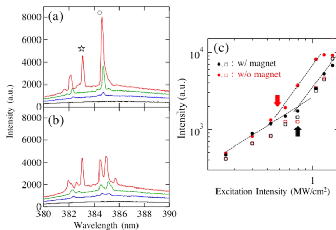
FIG. 2. Excitation intensity dependence of emission spectra in the (a) absence and (b) presence of the magnetic field. The excitation intensities were 0.26, 0.53, 0.79, and 1.05 \text{ MW/cm}^2 from bottom to top in each figure. (c) Excitation intensity dependence of emission peak intensities at 384.7 and 383.0 nm (indicated by circles and squares, respectively) with and without a magnetic field. These peaks correspond to the peaks indicated by a circle and star in Fig. 2(a).
