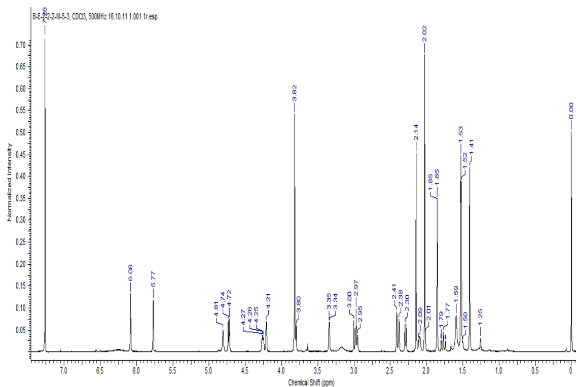
Figure 3.37 ^1\text{H} -NMR spectrum of compound 7
