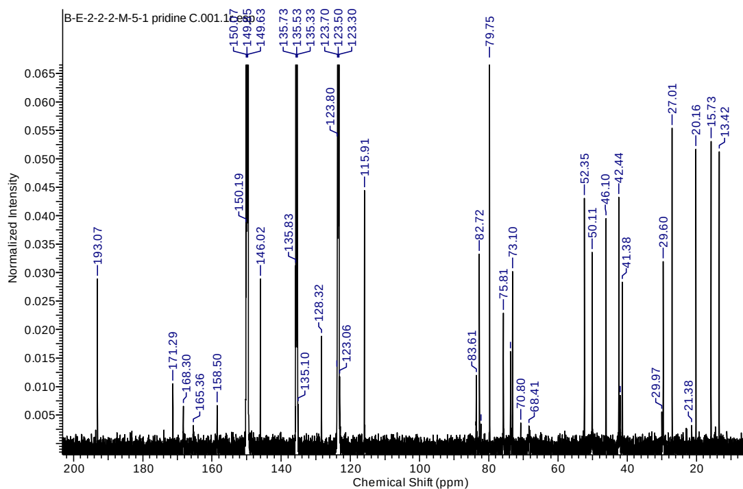
Figure 3.35 ^{13}\text{C} -NMR spectrum of compound 6
