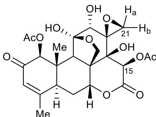
Figure 3.18 Structure of 1, 15- di-O-acetyl-13 \beta ,21-epoxyeurycomanone ( 4 )
