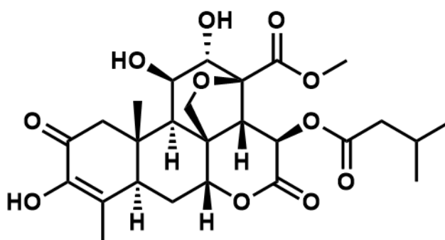
Figure 3.33 Structure of bruceine A (5)
