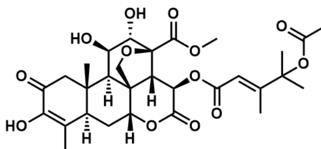
Figure 3.39 Structure of bruceantanol ( 7 )
