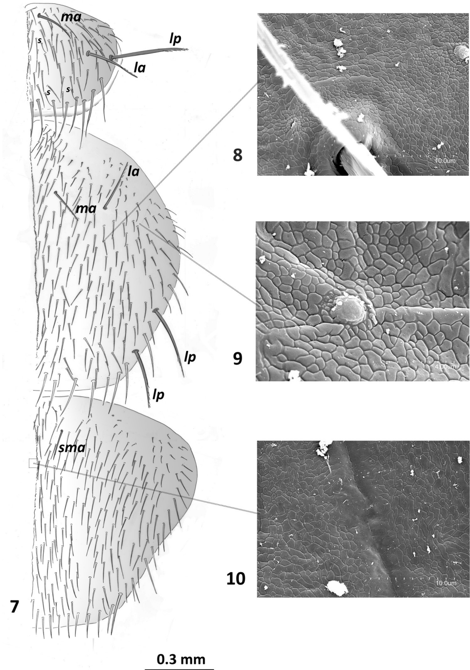
Figures 7–10. Pacificampa daidarabotchi Sendra, sp. n. 7 Pro-, meso- and metanotum, right side, holotype 8 detail epicuticle surface on mesonotum, paratype 9 detail epicuticle surface including external gland in the middle on mesonotum, paratype 10 detail epicuticle surface and the ecdysial suture on metanotum, paratype.
