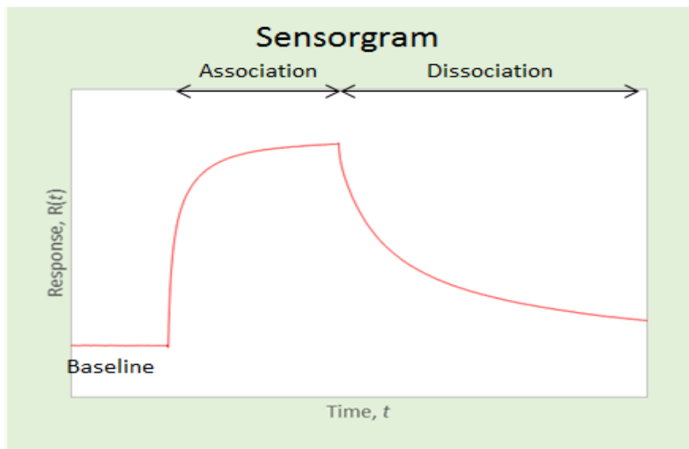
Figure 6: Surface plasmon resonance (SPR) The representative sensorgram obtained from kinetic analysis.
