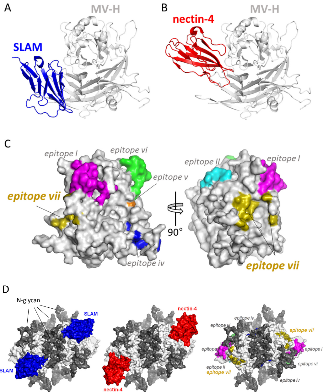
Figure 4: The complex structures of MV-H with receptors and the location of the epitopes on the MV-H protein. (A) Complex structure of MV-H and SLAM (PDB ID: 3ALZ). (B) Complex structure of MV-H and nectin-4 (PDB ID: 4GJT). (C) The location of the epitopes for neutralizing antibodies summarized in Table 1. Surface representation of the MV-H. The left panel shows a view of the same direction of A and B. The right panel shows a view rotated by 90° around a vertical axis. (D) Surface representation of the MV-H homodimer with SLAM (left), with nectin-4 (middle) and the location of the epitopes for neutralizing antibodies (right). MV-H is shown in white, potential N-linked glycan is shown in black (gray and light gray depending on the depth).
