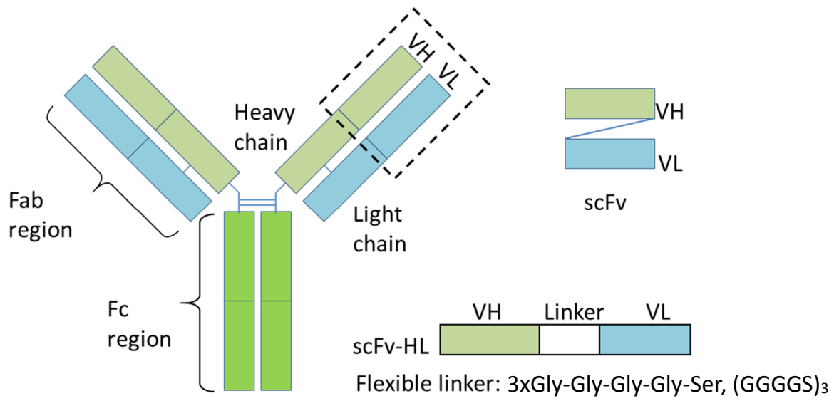
Figure 5: Schematic representation of the full length and the scFv antibodies. In the scFv, V H and V L domains are linked with the glycine-serine flexible linker (GGGGS) 3 .
