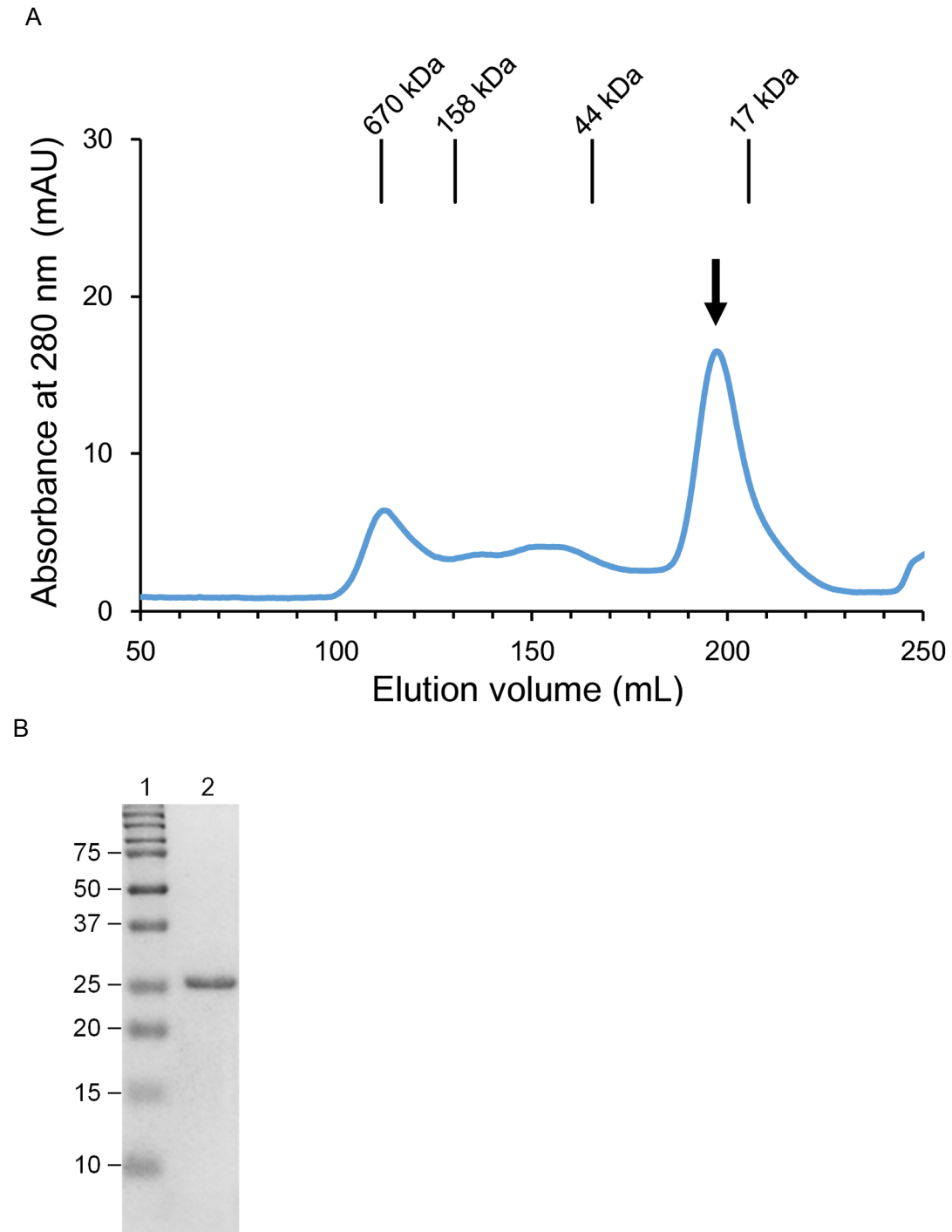
Figure 14: Purification of the recombinant 2F4-scFv protein.
