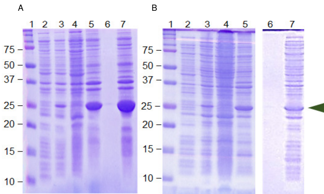
Figure 9: The SDS-PAGE for the expression and preparation of the inclusion body. Preparation of the inclusion bodies of 2F4-scFv with V_H - V_L (A) or V_L - V_H (B). Lane1, Protein size marker; lane 2, before induction; lane 3, after induction; lane 4, supernatant after cell disruption; lane 5, precipitate after cell disruption; lane 6, supernatant after wash of inclusion body; lane 7, precipitate after wash of inclusion body. Arrow indicates the corresponding size of the 2F4-scFv.
