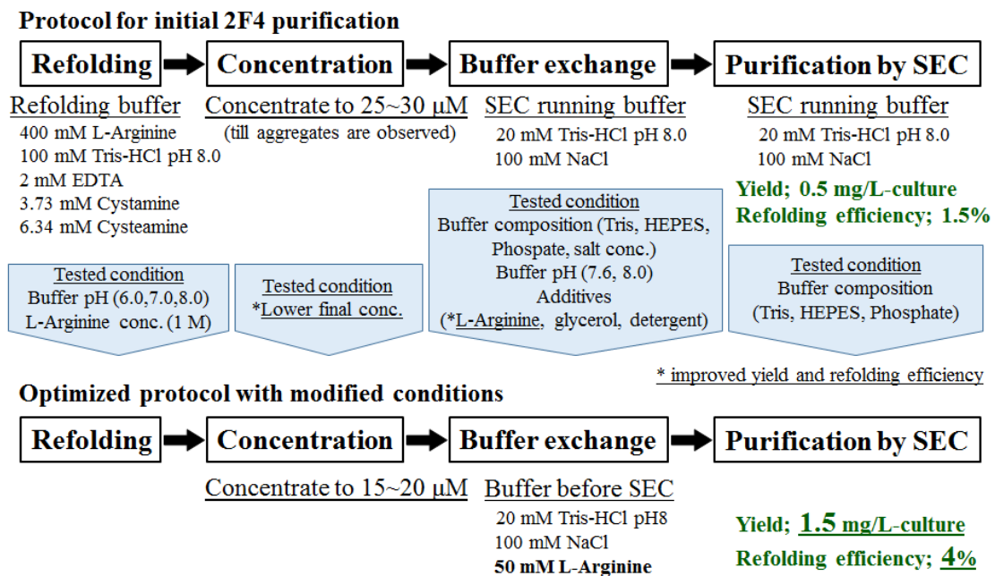
Figure 13: Summary of the examination for the purification conditions.
