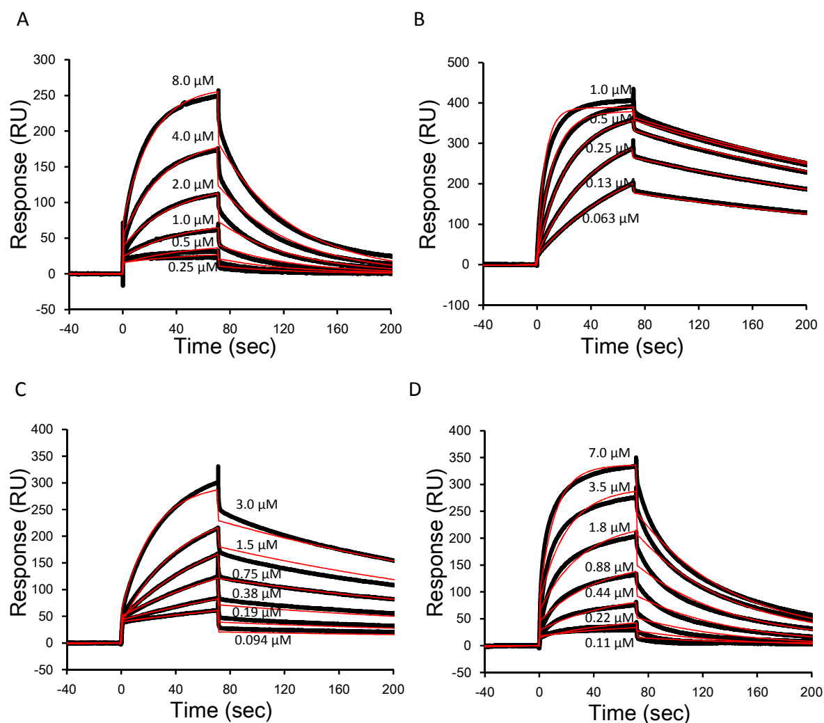
Figure 15: Kinetic analyses of 2F4-scFv, 2F4 Fab, SLAM or nectin-4 with MV-H.
