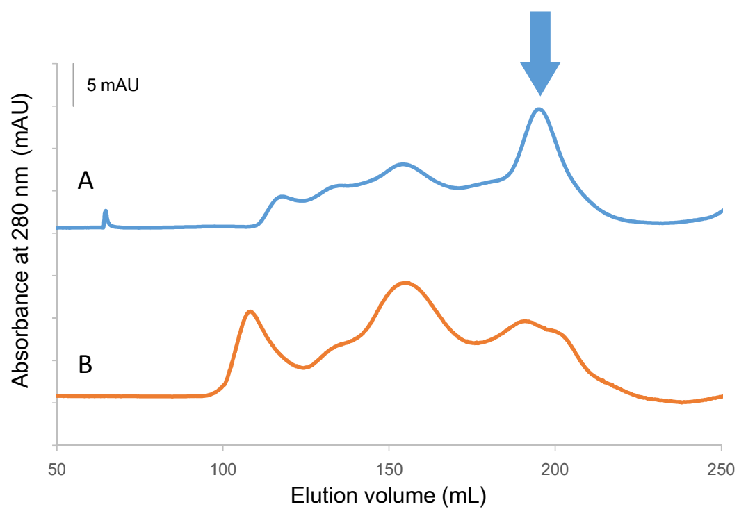
Figure 10: The chromatograms of the SEC for the 2F4-scFv-HL (A) and 2F4-scFv-LH (B). The arrow indicates the elution position of the 2F4-scFv.
