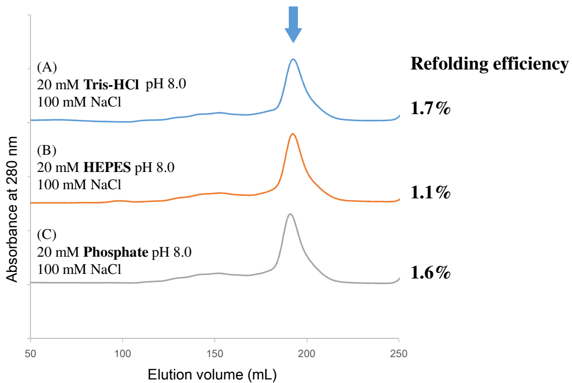
Figure 11: Examination of the buffer condition for SEC.
