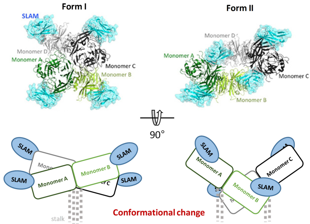
Figure 3: Different dimer of dimer (tetramer) forms of MV-H bound to SLAM.
