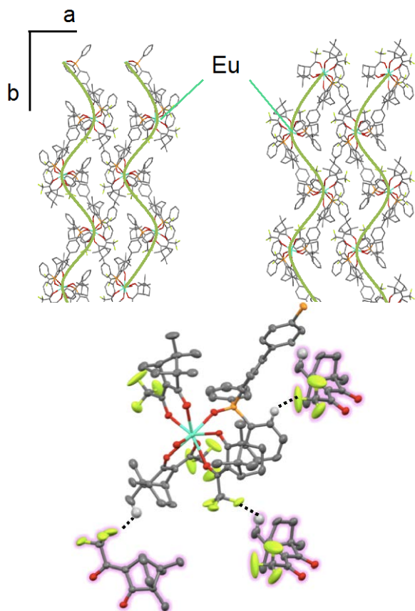
Fig. 2 Ortep views of [Eu(+/-tfc)_3(dpbp)]_n . Dot lines in ortep view shows CH/F interactions in crystal.
