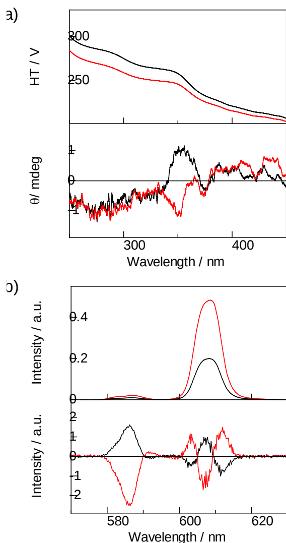
Fig. 4 a) Electronic absorption, CD, b) emission, and CPL spectra of [\text{Eu}(+\text{tfc})_3(\text{dpbp})]_n (Back line) and [\text{Eu}(-\text{tfc})_3(\text{dpbp})]_n (red line) in solid state.
