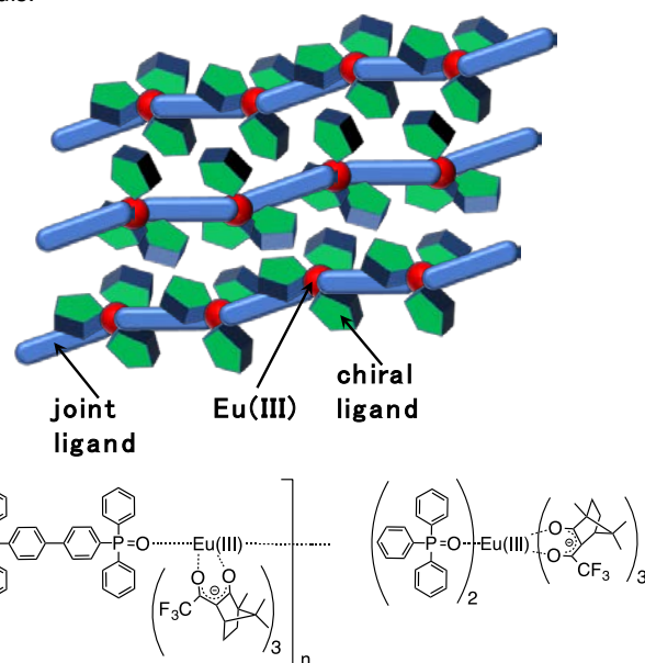
Fig. 1 a) Image and b) chemical structures of poly-nuclear [\text{Eu}(\text{+/-tfc})_3(\text{dpbb})]_n and mono-nuclear [\text{Eu}(\text{+/-tfc})_3(\text{tppo})] .
