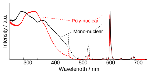
Fig. 3 Emission and excitation spectra of [Eu(+/-tfc)_3(dpbp)]_n (poly-nuclear: red line) and [Eu(+/-tfc)_3(tppo)] (mono-nuclear: black line) in solid states. Excitation wavelength for emission spectra at 380 nm. Detection wavelength for excitation spectra at 616 nm.
