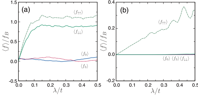
FIG. 10. The pairing functions at the center of a ferromagnet j = 25 are shown as a function of \lambda . (a) A strong ferromagnet at h = 0.5t . (b) A half-metallic ferromagnet at h = 2.5t .
