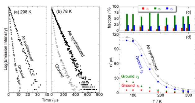
Figure 6. Emission decays of the as-synthesized (closed circles) and ground samples (open circles) of Cu-4-tpyb at (a) 298 K and (b) 78 K in the solid state ( \lambda_{\text{ex}} = 337 \text{ nm} ). Temperature dependence of (c) the fraction and (d) lifetime of each emission component (red, green, and blue symbols represent the emission components with short ( \tau_1 ), middle ( \tau_2 ), and long ( \tau_3 ) lifetimes) observed for the ground sample of Cu-4-tpyb . Data of the as-synthesized Cu-4-tpyb is also shown in (d).
