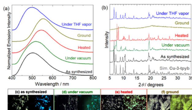
Figure 7. Changes in the (a) emission spectrum ( \lambda_{\text{ex}} = 350 \text{ nm} ) and (b) PXRD pattern of Cu-3-tpyb by (green) drying under vacuum, and subsequent (red) heating, (orange) manual grinding, and (blue) exposure to THF vapor at room temperature. Black curves show the spectrum and pattern of the as-synthesized sample. Gray curve at the bottom in (b) shows the simulation pattern calculated from the crystal structure of Cu-3-tpyb . Photographs in (left) bright field and (right) under UV light of the (c) as-synthesized, (d) vacuum-dried, (e) heat-dried, and (f) ground Cu-3-tpyb are shown.
