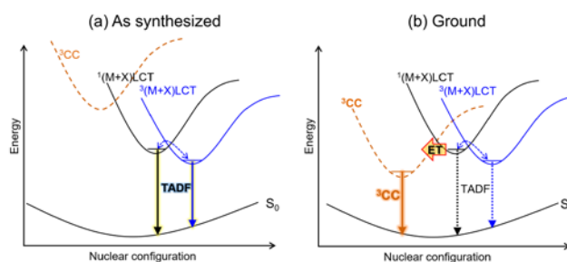
Scheme 2. Schematic energy diagrams of the (a) as-synthesized and (b) ground samples of Cu-4-tpyb .
