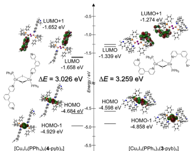
Figure 4. Schematic molecular orbital diagrams for the model dinuclear complexes, (left) [Cu 2 I 2 (PPh 3 ) 2 (4-pyb) 2 ] and (right) [Cu 2 I 2 (PPh 3 ) 2 (3-pyb) 2 ]. The energy gap between HOMO and LUMO is also shown.
