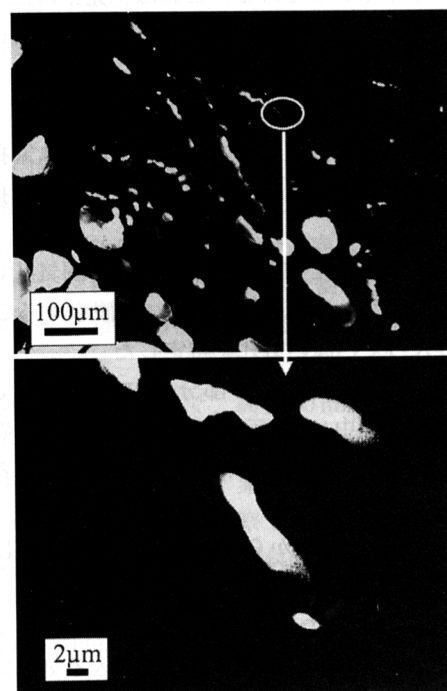
Fig. 8. Minimum size of pore, which can be observed in this experiment by microscope.
