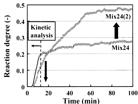
Fig. 13. Effect of water keeping method of catalyst on the reaction curve (Mix: hematite + graphite).
