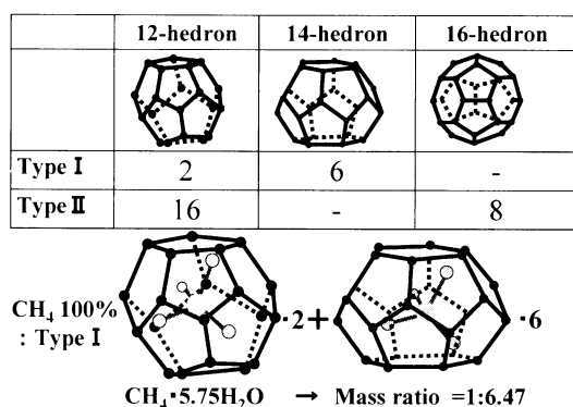
Fig. 1. Structures of methane hydrate.
