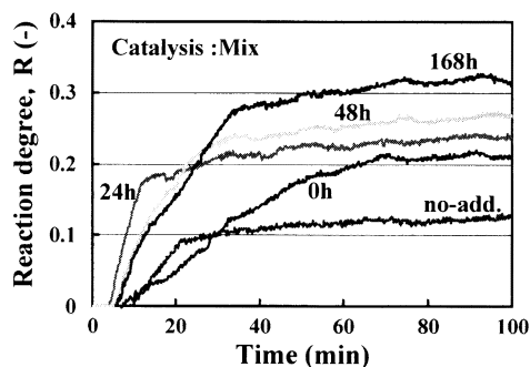
Fig. 8. Effect of milling time and catalyst "Mix" on the variation of reaction degree of methane hydrate formation.
