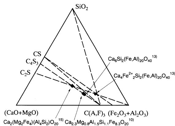
Fig. 5. Chemical compositions of reported SFCA single crystals.
