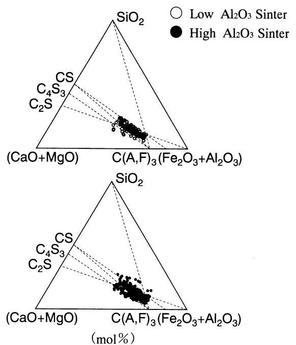
Fig. 2. Chemical composition domain of calcium ferrite.
