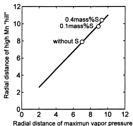
Fig. 12. Relationship between position of maximum metal vapor pressure and high Mn "hill" in Fe-Mn alloy with different S content.
