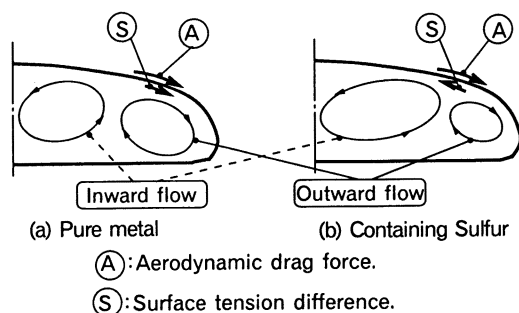
Fig. 11. The effects of aerodynamic drag force and surface tension difference on the size of outward flow.
