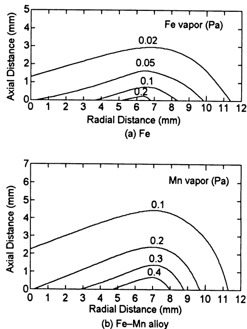
Fig. 2. Distributions of metallic vapor pressure in plasma melting of Fe and Fe-Mn alloy.
