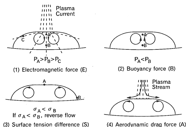
Fig. 7. Driving forces of melt flow in plasma button melting.
