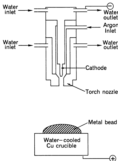
Fig. 1. Schematic diagram of torch and crucible.
