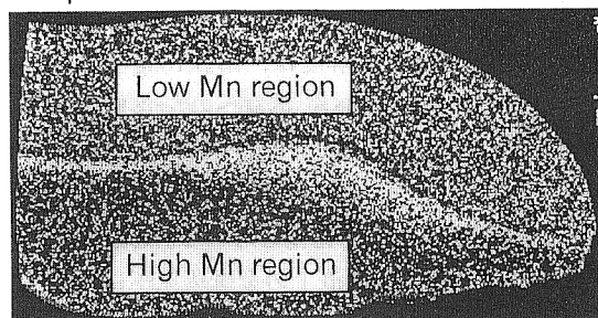
Fig. 6. Distribution of Mn concentration in cross section of Fe-Mn alloy sample after 30 minutes melting.
