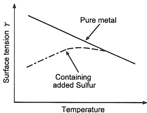
Fig. 9. Schematic surface tension-temperature behavior for iron.
