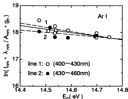
Fig. 5. Ar Boltzmann plot obtained by Wiese's Ar transition probabilities.
