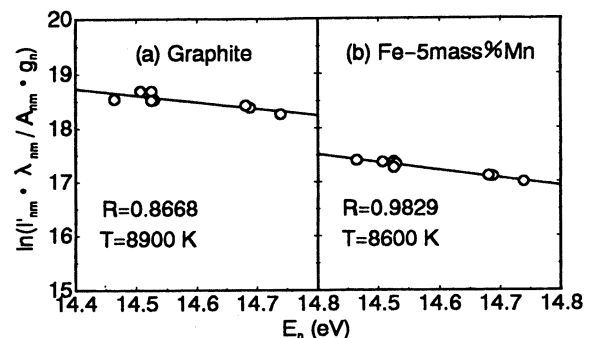
Fig. 9. Effect of metallic vapor on Boltzmann plot.
