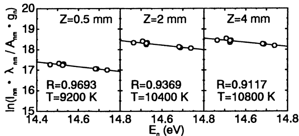
Fig. 6. Effect of temperature on the Boltzmann plot by new transition probabilities shown in Table 1.
