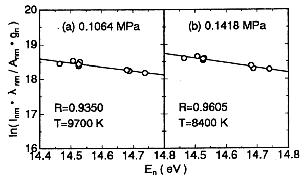
Fig. 8. Effect of plasma pressure on Boltzmann plot.
