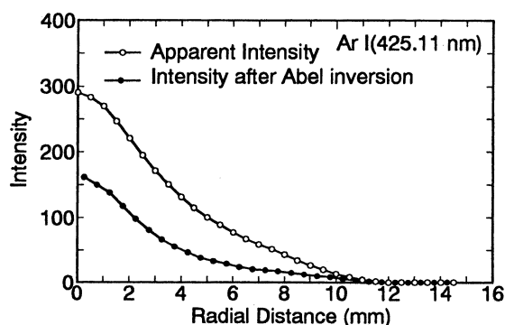
Fig. 4. Radial distribution of spectrum intensity.
