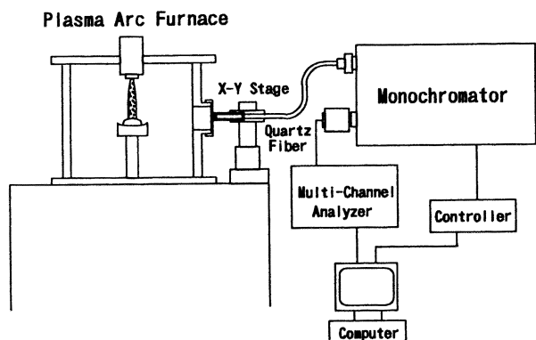
Fig. 2. Scheme of experimental apparatus.
