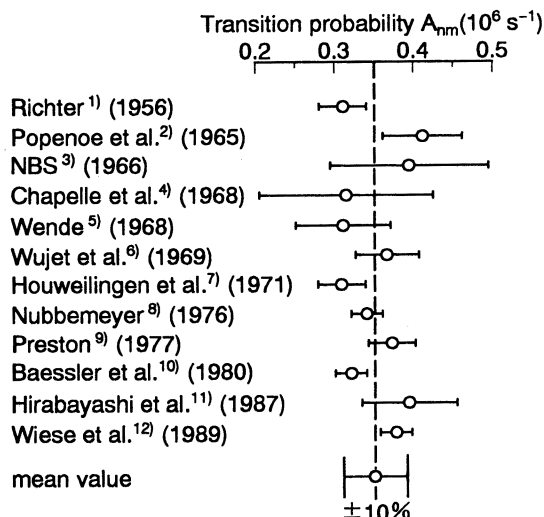
Fig. 1. Reported transition probabilities of Ar I line at 430.01nm.
