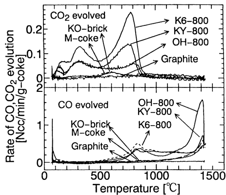
Fig. 2. Rate of CO, CO 2 evolution from coke in Ar atmosphere.
