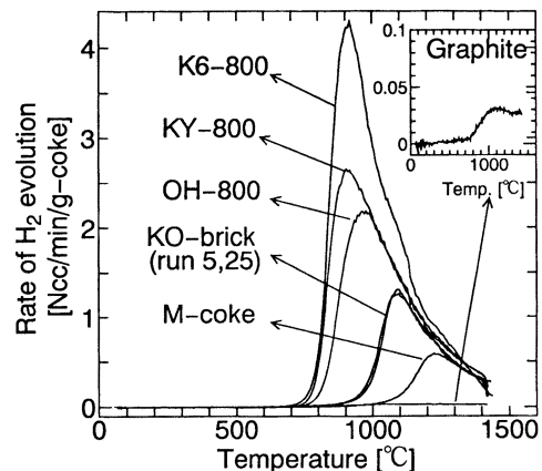
Fig. 1. Rate of H 2 evolution from coke in Ar atmosphere.
