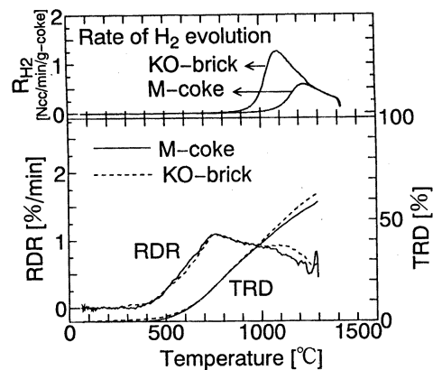
Fig. 4. Comparison of RDR and TRD between M-coke and KO-brick (MTCC).
