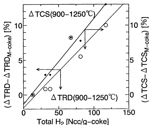
Fig. 10. Difference of TRD and TCS between M-coke and MTCC or LTCC from 900°C to 1250°C.
