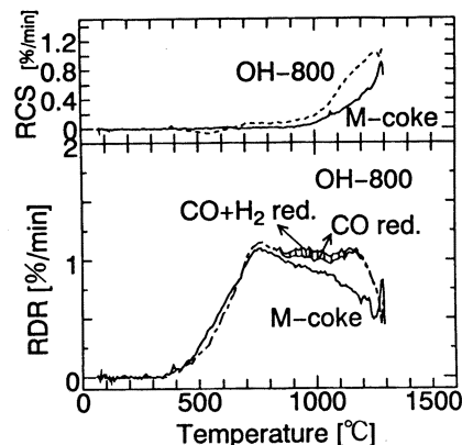
Fig. 7. Comparison of RDR and RCS between M-coke and OH-800(LTCC).
