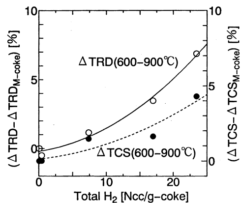
Fig. 9. Difference of TRD and TCS between M-coke and MTCC or LTCC from 600℃ to 900℃.
