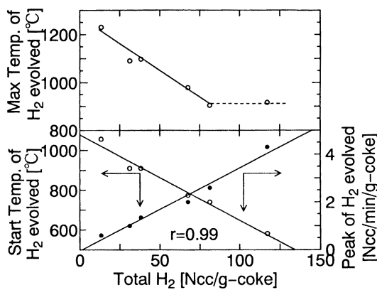
Fig. 3. Relationships between total amount and evolution curve of H 2 .
