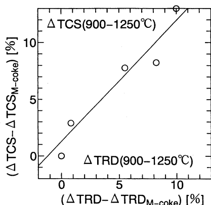
Fig. 11. Relationship between \Delta\text{TRD} and \Delta\text{TCS} from 900°C to 1250°C.
