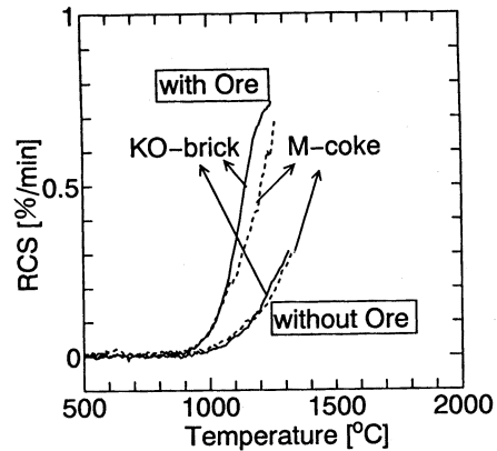
Fig. 8. Increase of gasification rate (RCS) when coke reacts with sinter in mixed bed.
