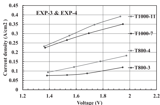
Fig. 12. Relationship between voltage and current density for EXP-3 and EXP-4.
