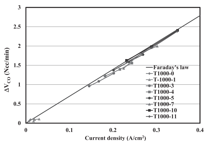
Fig. 13. Comparison of current densities with Faraday's law.
