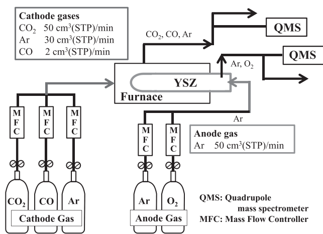
Fig. 5. Schematics of experimental apparatus.
