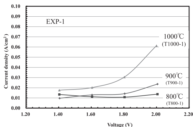
Fig. 10. Variation of IR drop at each applied voltages in 1000°C.
