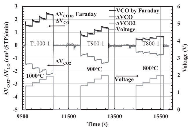
Fig. 7. Typical experimental results of 1 000°C, 900°C and 800°C.
