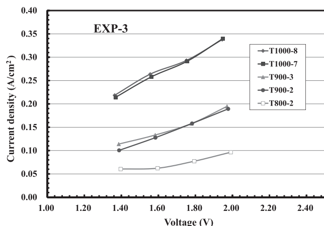
Fig. 11. Relationship between voltage and current density for EXP-3.
