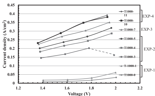
Fig. 8. Relationship between voltage and current density in 1000^\circ\text{C} .
