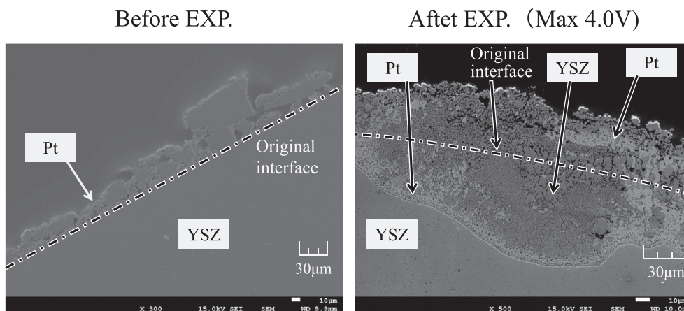
Fig. 14. Cross sectional image of interface between YSZ and Pt electrode before and after experiment.
