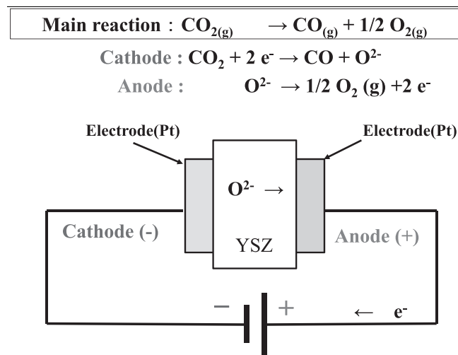
Fig. 2. Reaction system in the present study.
