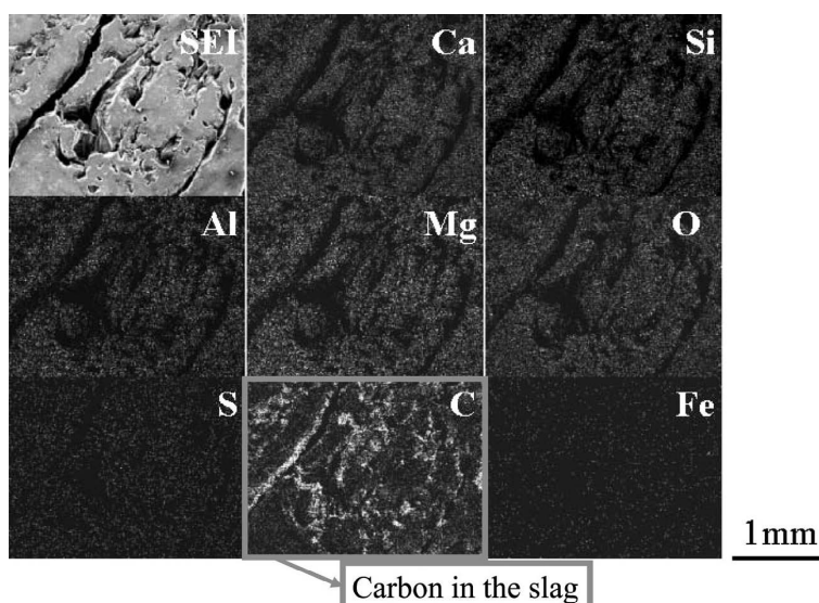
Fig. 4. Result of EDS analysis for the foamed slag.
