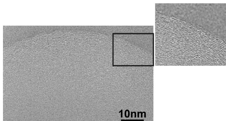
Fig. 7. High resolution TEM observation of onion type carbon particle.
