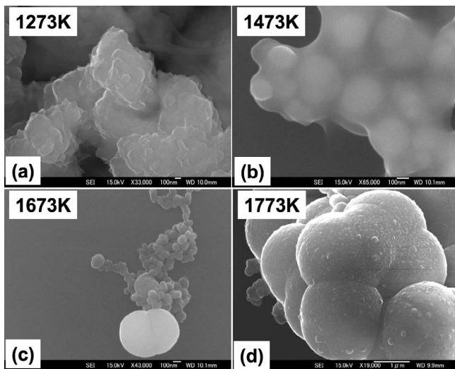
Fig. 5. Results of SEM observation of the soot type carbon particles precipitated at different temperatures.
