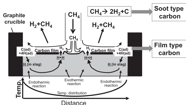
Fig. 8. Reaction mechanism for forming of the carbon film in cooperation with slag melt and soot type carbon formation in gas phase.
