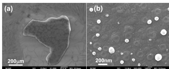
Fig. 9. SEM observation of carbon film. (a) Fragment of carbon film, (b) High magnification of surface of carbon film with carbon particles.
