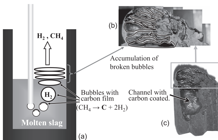
Fig. 2. Phenomena during CH 4 injection into molten slag.
