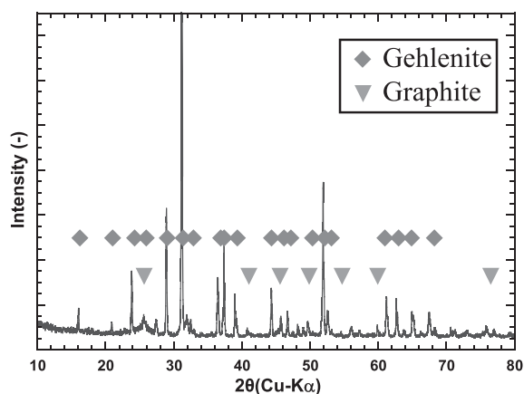
Fig. 3. Result of XRD of bubbles accumulating.
