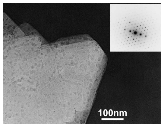
Fig. 10. TEM image and SAD pattern of carbon film.
