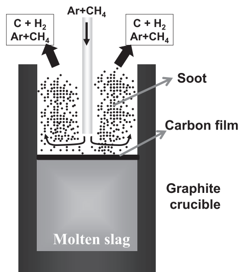
Fig. 1. Types of carbons formed during the blowing to the slag surface.
