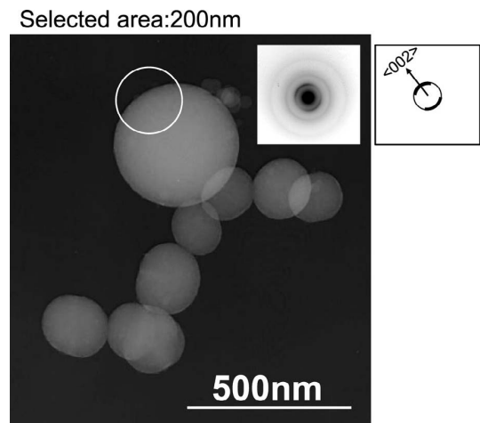
Fig. 6. TEM image and SAD pattern of the spherical carbon particle precipitated at 1773 K.
