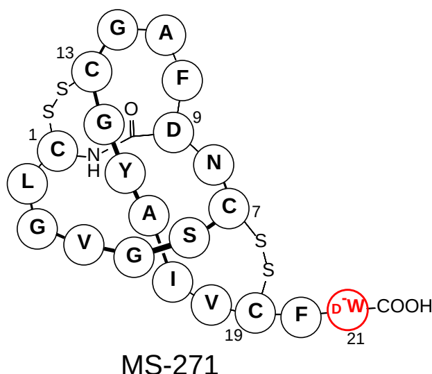
Figure 1. Structure of MS-271.
