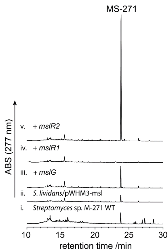
Figure 3. LC-MS analysis of products accumulated in the cultures. i) Streptomyces sp. M-271 wild type, ii) S. lividans /pWHM3-msl, iii) S. lividans:mslG /pWHM3-msl, iv) S.
