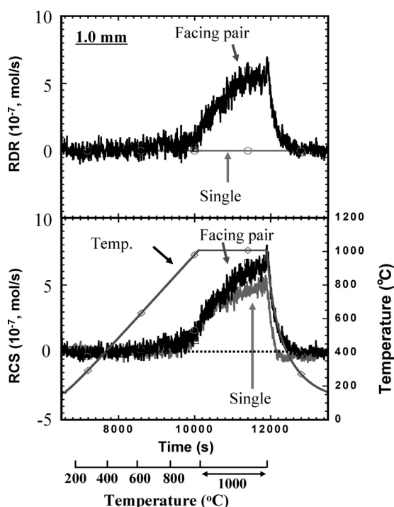
Fig. 10. Variations of RDR and RCS with time. (Ar-30% \text{CO}_2 : 10 cm/s, 1.0 mm, facing pair: hematite-graphite pair, single: graphite-alumina pair)
