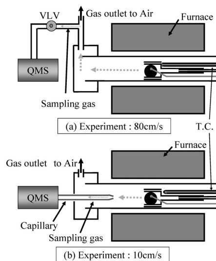
Fig. 3. Improvement of gas sampling method. VLV: variable leak valve, QMS: quadrupole mass spectrometer.
