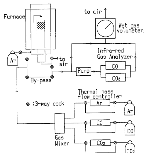
Fig. 11. Schematic diagram of experimental apparatus.
