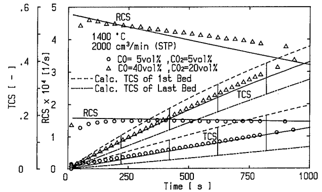
Fig. 16. Comparison between calculated results and observed data (RCS=RCS e at 1 400°C).
