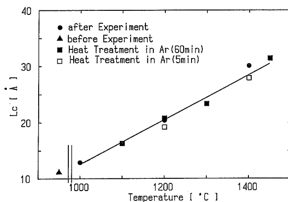
Fig. 5. Relationship between L_c and temperature.
