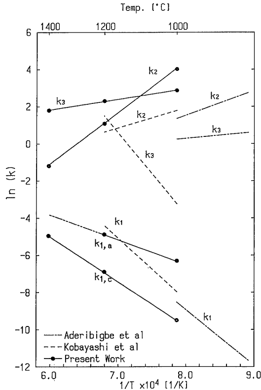
Fig. 13. Arrhenius plot of rate constants.
