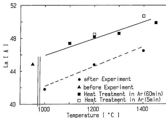
Fig. 6. Relationship between L_a and temperature.
