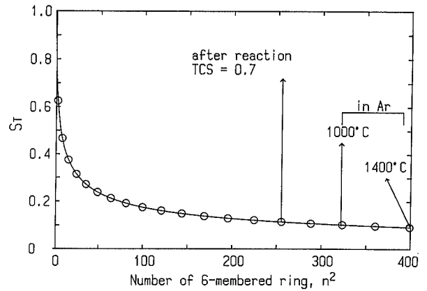
Fig. 9. Relationship between the number of dangling bond per carbon atom ( S_T ) and six-membered ring ( n^2 ).
