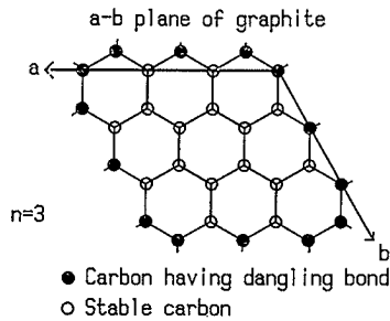
Fig. 8. Model of carbon network having dangling bond ( n=3 ). It is postulated that graphite crystal equiaxially develops on a-b plane of unit cell.
