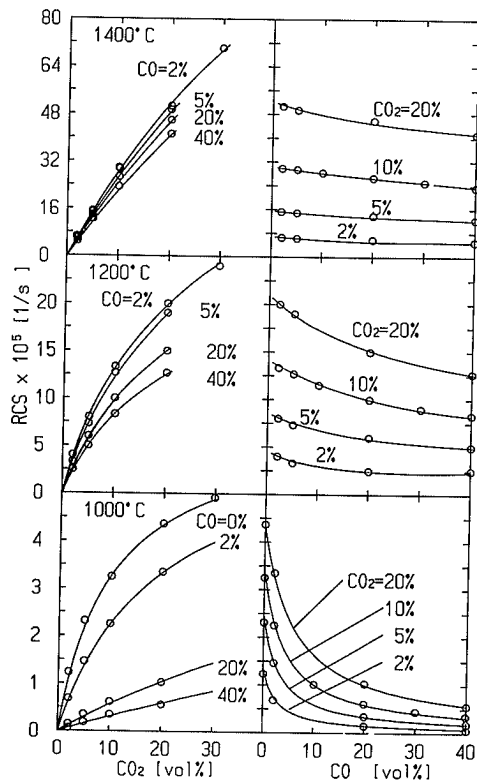
Fig. 12. Variation of RCS with experimental conditions.
