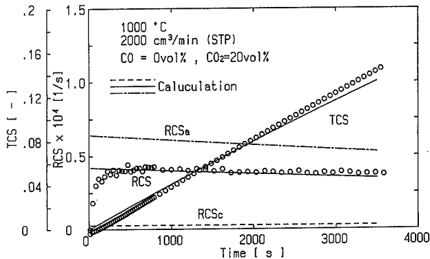
Fig. 14. Comparison between calculated results and observed data (1 000°C).
