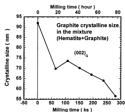
Fig. A3. Variations of crystalline size of graphite in the mixture with milling time.
