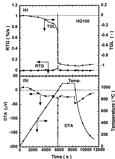
Fig. 1. Typical results of TG-DTA for the mixture of hematite and graphite after milling for 100 hr (HG100). (TGL: weight loss curve, RTG: rate of weight loss, DTA: temperature difference between reference and sample, Temp.: heating profile)
