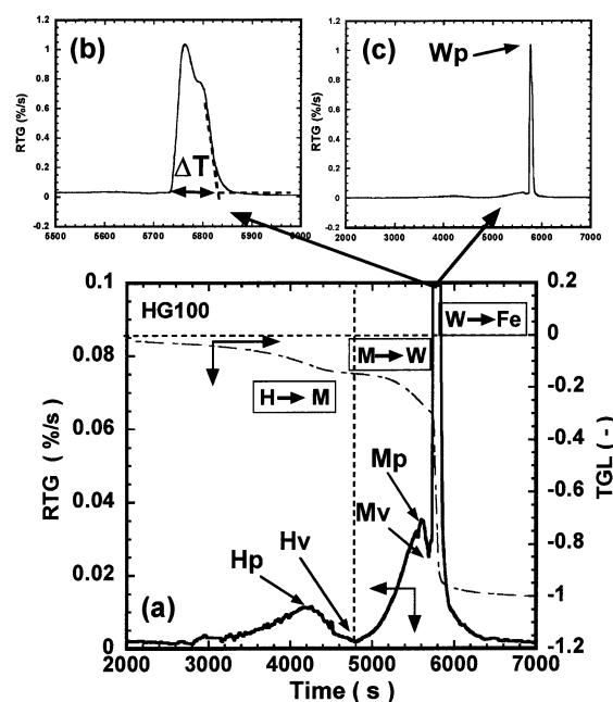
Fig. 2. Details of RTG curve and definitions of characteristic points.
