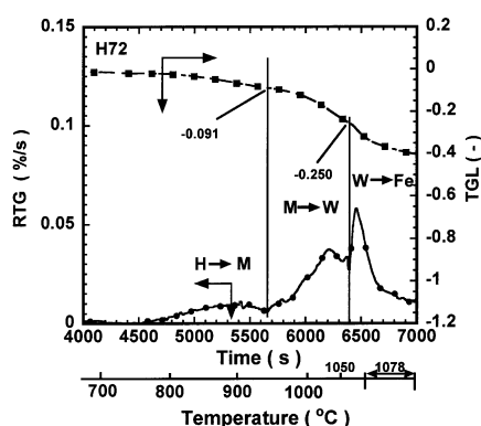
Fig. 7. Variations of TGL and RTG curves for H72.
