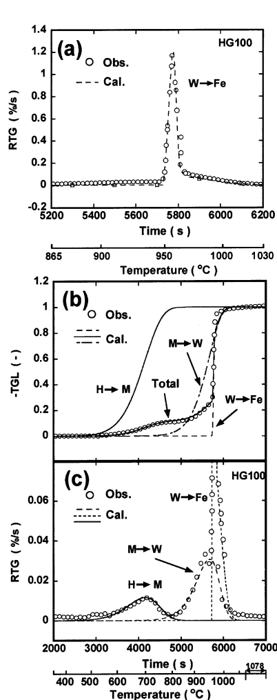
Fig. 11. Calculation results of TGL and RTG curves in HG100 and comparison with the observation.
