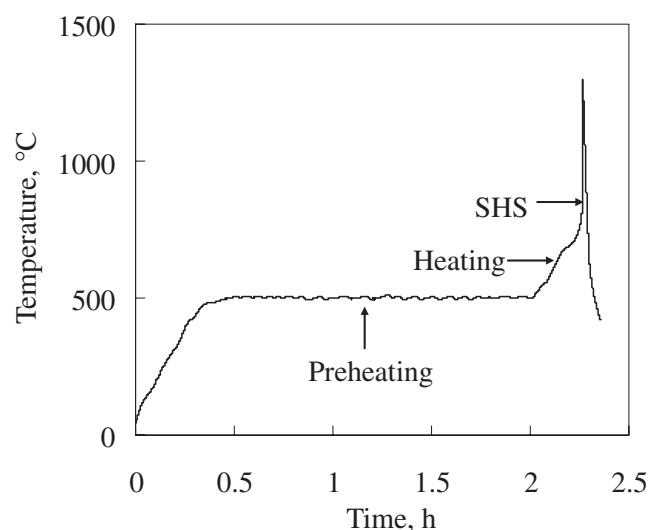
Fig. 8 Temperature change during and after preheating of the compact. f_v = 0.6 .
