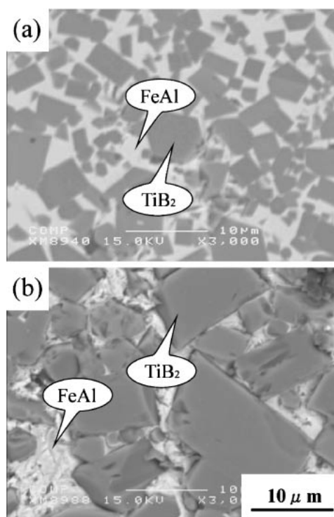
Fig. 2 SEM images of samples. (a) f_v = 0.6 , (b) 0.8.
