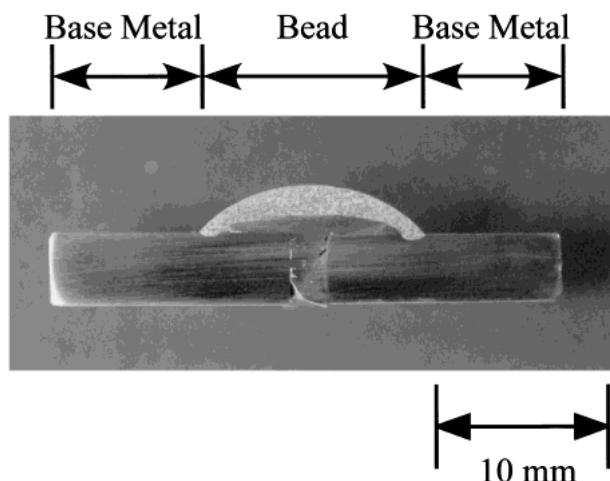
Fig. 9 Photograph of a cross section of a welded sample. The initial temperatures of the Al droplet, Ni powder and base metal were all 1373 K. The root gap was 2 mm.
