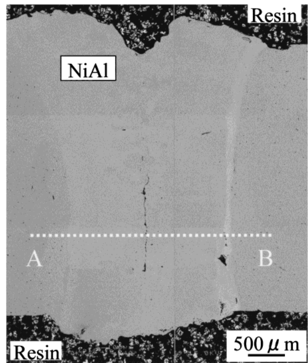
Fig. 14 SEM image of the sample shown in Fig. 13. Line AB indicates the trace of EPMA analysis.
