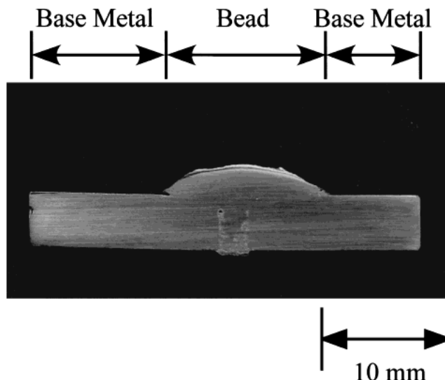
Fig. 11 Photograph of a cross section of a welded sample. The initial temperatures of the Al droplet, Ni powder and base metal were all 1473 K. The root gap was 2 mm.
