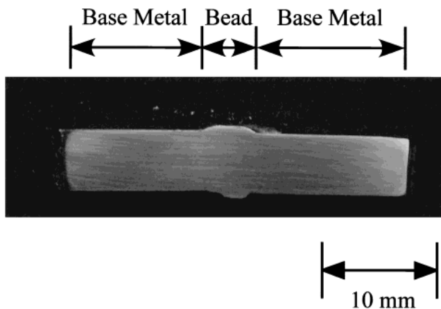
Fig. 13 Photograph of a cross section of a welded sample. The initial temperatures of the Al droplet, Ni powder and base metal were all 1473 K. The root gap was 3 mm.
