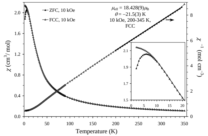
Figure 2. ZFC (filled symbols) and FCC (empty symbols) dc magnetic susceptibility ( \chi = M/H ) curves of \text{Ho}_2\text{MnGaMn}_4\text{O}_{12} at 10 kOe (left-hand axis). The right-hand axis shows the inverse FCC 10 kOe curve with Curie-Weiss fitting results. The inset shows a fragment of the ZFC and FCC \chi versus T curves at H = 10 kOe.
