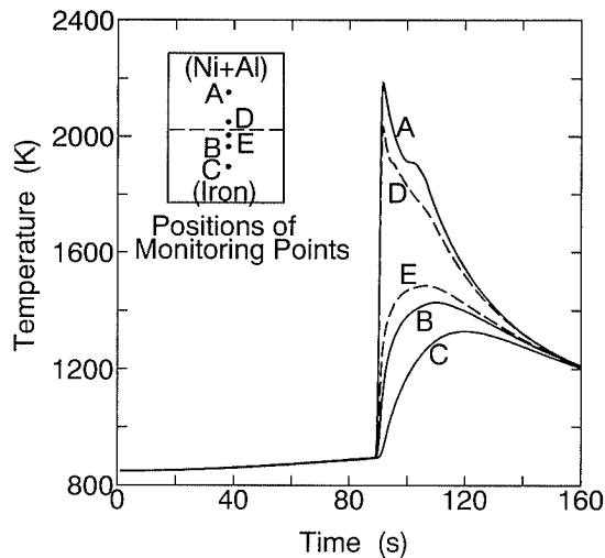
Fig. 2. Simulated time-temperature curves of the joining couple.
