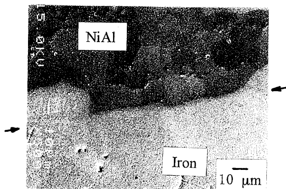
Fig. 5. Microstructure of the joining couple photographed by using a scanning electron microscope. Arrows indicate the joining interface.
