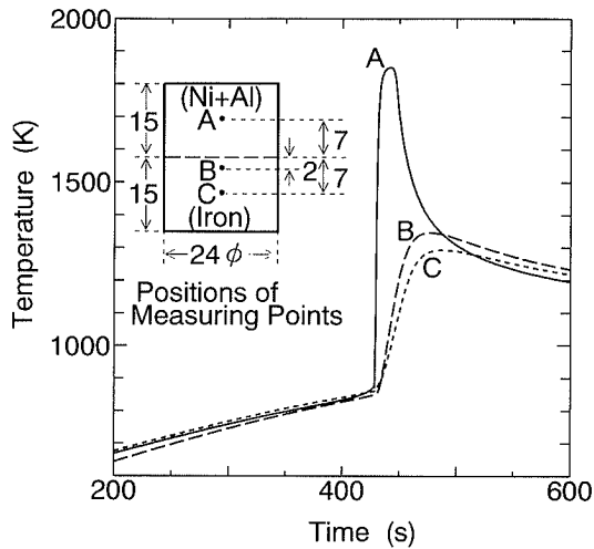
Fig. 1. Measured time-temperature curves of the joining couple.
