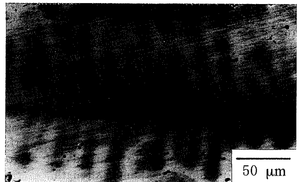
Fig. 4. Microstructure of the synthesized NiAl, showing columnar dendrites. Etchant: Marble's reagent.
