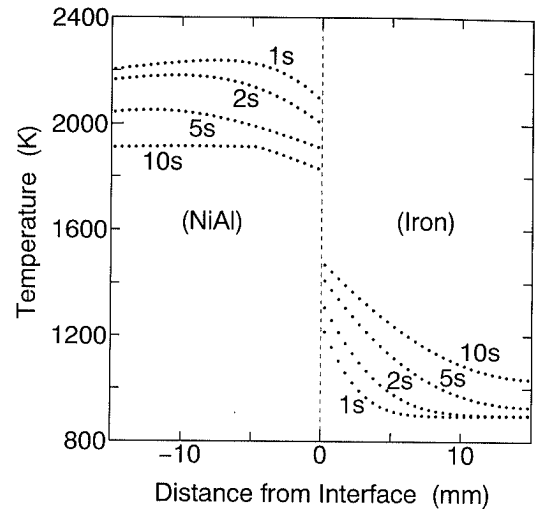
Fig. 3. Simulated temperature distribution curves on the longitudinal axis of the joining couple at several moments from the onset of the synthesis reaction.
