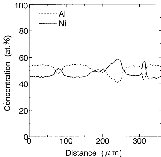
Fig. 8. Concentration distributions of nickel and aluminum in the synthesized NiAl away from the joining interface.
