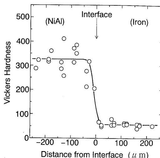
Fig. 7. Hardness distribution across the joining interface.
