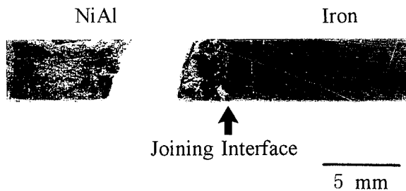
Fig. 9. Fractured specimen of a four-point bending test.
