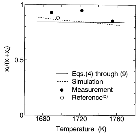
Fig. 7. Temperature dependence of the fraction in the thickness of the \gamma -phase formed by the transformation from the \delta -phase. x_1 represents the \gamma -phase thickness formed by the transformation from the \delta -phase and x_2 by the solidification from the liquid phase.
