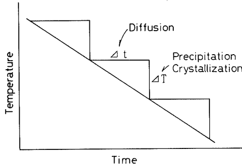
Fig. 1. Continuous cooling process simulated as a sequential combination of isothermal holding and quenching at very small steps in both time and temperature.
