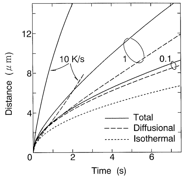
Fig. 6. Relationship between time and the migration distance of \gamma/\text{liquid} interface at various cooling rates.
