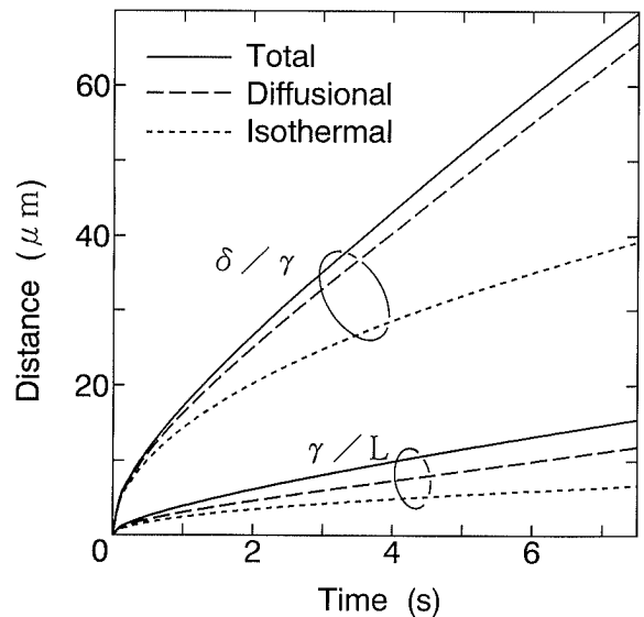
Fig. 4. Relationship between time and the migration distance of the interfaces.
