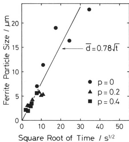
Fig. 7. Relation between the ferrite particle size, \bar{d} , and time from rolling, t . p : rolling reduction
