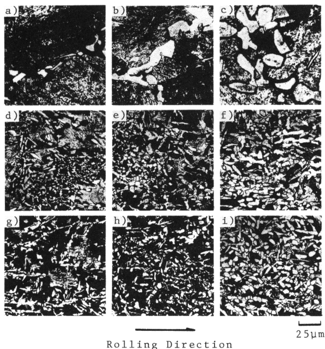
Fig. 6. Change in the ferrite structure during the transformation.
