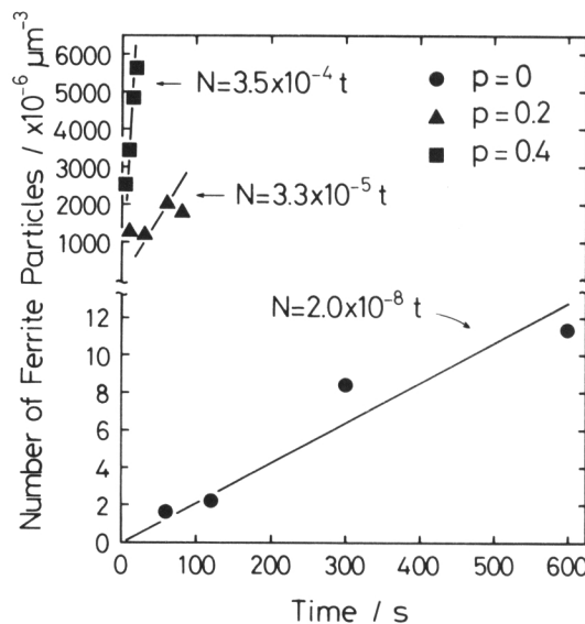
Fig. 8. Relation between the number of ferrite particles, N , and time from rolling, t . p : rolling reduction
