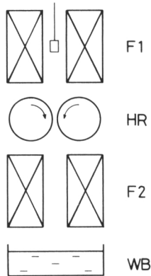
Fig. 3. Schema of the apparatus. F1, F2: furnace HR: roller WB: water bath
