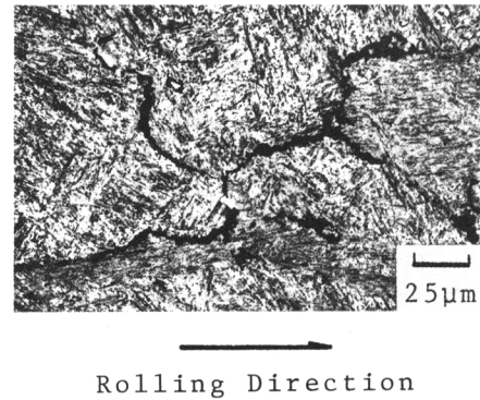
Fig. 4. Structure of the sample quenched soon after rolled at 710°C, showing no evidence of ferrite transformation during rolling. Rolling reduction: p=0.2 .
