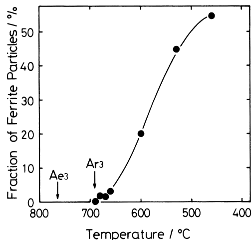
Fig. 1. Increase in the volume fraction of ferrite particles during cooling at 0.3°C/s.
