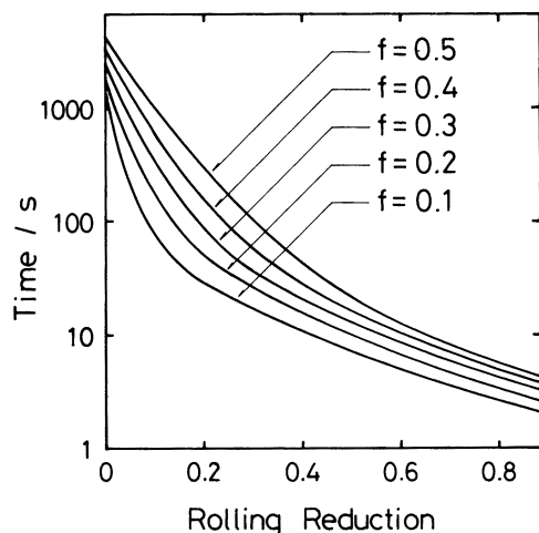
Fig. 10. Effect of rolling reduction on the time required for the transformation. f: volume fraction of ferrite particles
