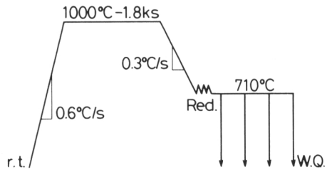
Fig. 2. Thermal history.
