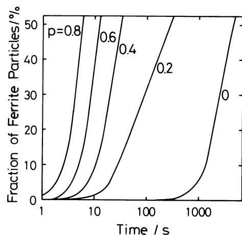
Fig. 9. Calculated transformation behavior for different rolling reduction.
