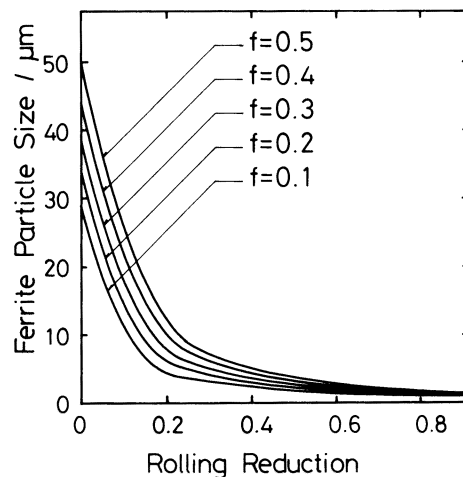
Fig. 11. Relation between the rolling reduction and the average ferrite particle size. f: volume fraction of ferrite particles
