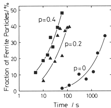
Fig. 5. Transformation behavior for different rolling reduction, p .
