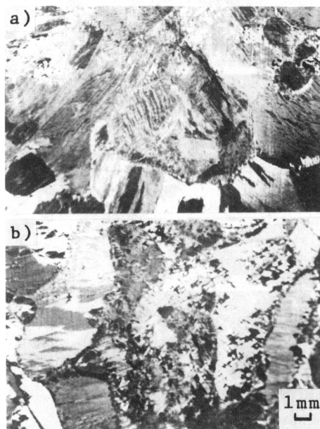
a) Equiaxed grains, G_t = 1.5^{\circ}\text{C/mm} b) Columnar grains G_t = 3.0^{\circ}\text{C/mm} Cooling rate : 0.2^{\circ}\text{C/s} Quenching temperature : 1350^{\circ}\text{C}
