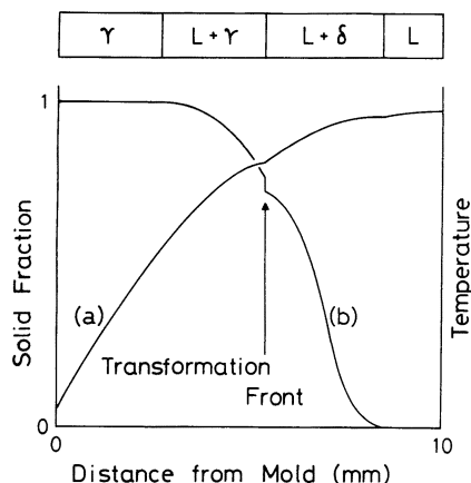
Fig. 5. The illustrated distribution of (a) temperature and (b) solid fraction on the radius of the ingot of hyper-peritectic composition.
