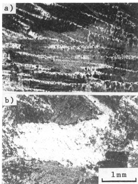
Photo. 3. The comparison between the a)dendritic and b)austenitic structures in 0.2%C steel cooled at 3^{\circ}\text{C/s} and quenched from 1000^{\circ}\text{C} .
