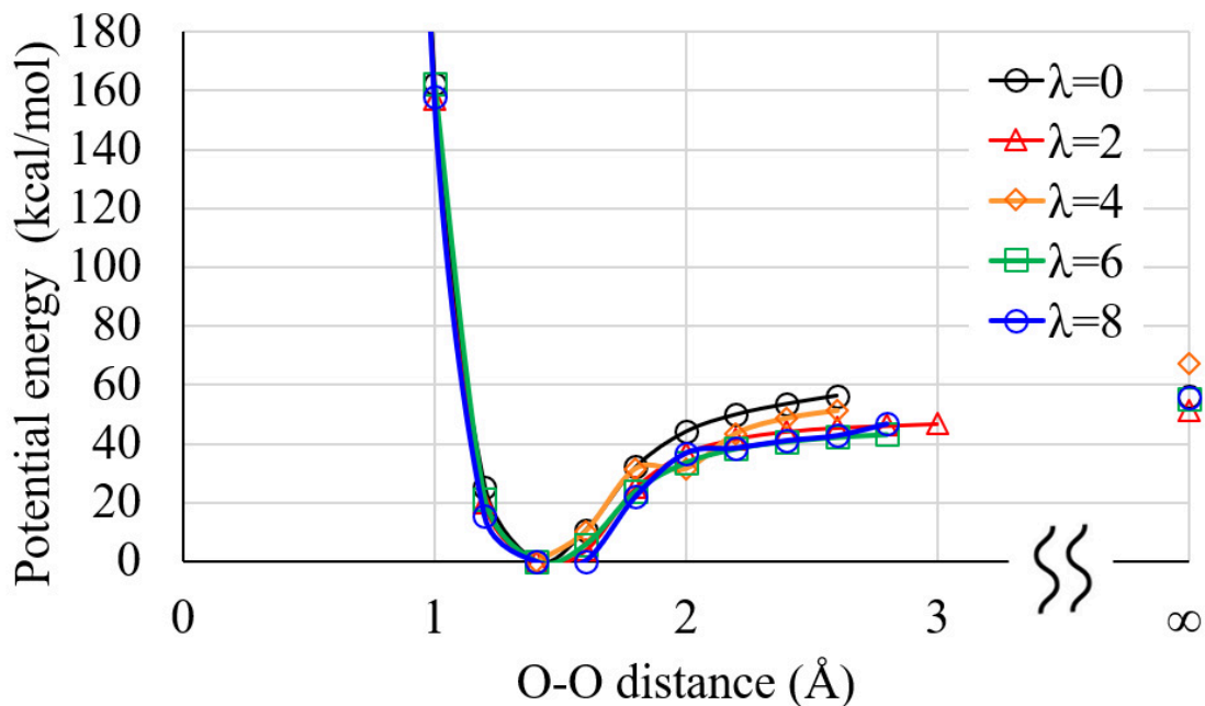
FIG. 2: Potential energy curves of the O-O dissociation of \text{H}_2\text{O}_2 to OH radicals for the explicit hydration numbers \lambda = 0, 2, 4, 6 , and 8 in aqueous solution. The spin-restricted Kohn-Sham calculations are performed under the stability condition for switching to the spin-unrestricted ones. 29,30 LC-BLYP/cc-pVDZ is used with the solvent effect of the polarizable continuum model of water. The minimum potential energies are set to be zero. The dissociation limit energies, which are calculated by equally dividing the hydrated \text{H}_2\text{O}_2 such as \text{H}_2\text{O}_2(\text{H}_2\text{O})_{2\lambda} \rightarrow 2\text{OH}(\text{H}_2\text{O})_\lambda , are also shown at the infinite O-O distance.
