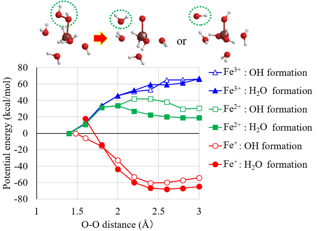
FIG. 4: Potential energy curves of the O-O bond dissociation of \text{H}_2\text{O}_2 , which is coordinated to the iron ion hydration complexes in [\text{Fe}(\text{H}_2\text{O}_2)(\text{H}_2\text{O})_5]^{n+} , for the valence of n = 1, 2 , and 3. LC-BLYP/cc-pVDZ/LanL2DZ is used with the solvent effect of the polarizable continuum model of water. The dotted green circles indicate the \text{H}_2\text{O}_2 molecule and formed \text{H}_2\text{O} molecule and OH radical.
