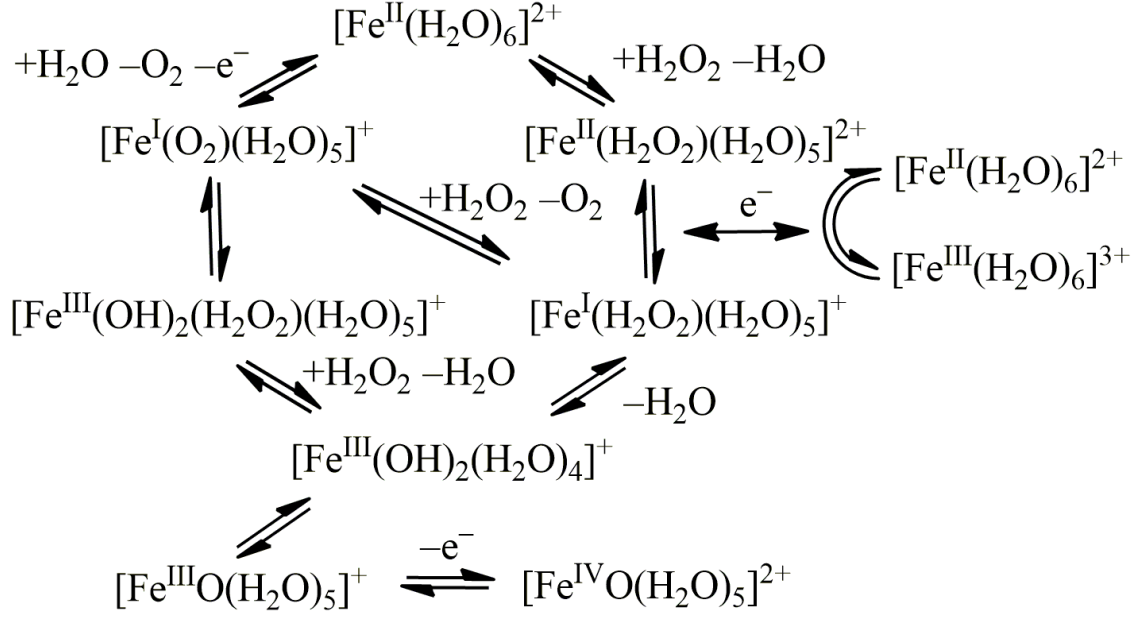
FIG. 7: Schematic overview of \text{H}_2\text{O}_2 decomposition mechanism by iron ion hydration complex.
