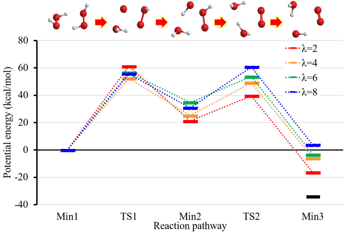
FIG. 3: Reaction diagram of \text{H}_2\text{O}_2 decomposition reaction, i.e., 2\text{H}_2\text{O}_2 \rightarrow \text{O}_2 + 2\text{H}_2\text{O} , under the absence of metal ions in aqueous solution. LC-BLYP/cc-pVDZ is used with the solvent effect of the polarizable continuum model of water. Zero-point vibrational corrections are included. The molecular structures of the reaction processes are also shown for the complex with no water molecule. For Min3, the potential energy of the triplet state for \lambda = 8 is also shown as a black bar.
