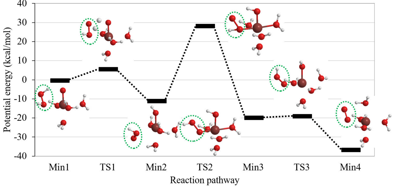
FIG. 5: \text{O}_2 formation mechanism of the \text{H}_2\text{O}_2 -coordinated \text{FeO}^+ ion hydration complex with no additional \text{H}_2\text{O} molecules, i.e., [\text{FeO}(\text{H}_2\text{O}_2)(\text{H}_2\text{O})_4]^+ . LC-BLYP/cc-pVDZ/LanL2DZ is used with the solvent effect of the polarizable continuum model of water. Zero-point vibrational corrections are included. The potential energy of the reactant complex (Min1) is set to be zero. The dotted green circles indicate the \text{H}_2\text{O}_2 molecules and their decomposed fragments.
