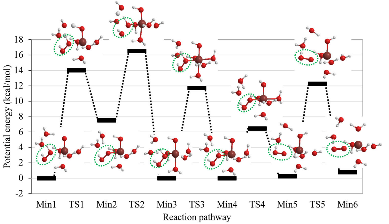
FIG. 6: \text{O}_2 formation mechanism of the \text{H}_2\text{O}_2 -coordinated \text{FeO}^+ ion hydration complex with two \text{H}_2\text{O} molecules, i.e., [\text{FeO}(\text{H}_2\text{O}_2)(\text{H}_2\text{O})_4]^+(\text{H}_2\text{O})_2 . LC-BLYP/cc-pVDZ/LanL2DZ is used with the solvent effect of the polarizable continuum model of water. Zero-point vibrational corrections are included. The potential energy of the reactant complex (Min1) is set to be zero. The dotted green circles indicate the \text{H}_2\text{O}_2 molecules and their decomposed fragments.
