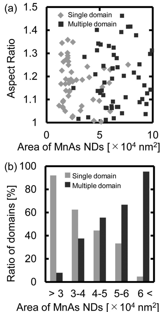
FIG. 2. Size dependence of the magnetic domain structure of MnAs NDs on AlGaAs NP buffers. (a) The two-dimensional distributions of single and multiple magnetic domains as a function of the area and the aspect ratio of the MnAs NDs. The aspect ratio is defined as the ratio of the longest length of the \langle 11-20 \rangle direction divided by the shortest length of the \langle 1-100 \rangle direction of the MnAs NDs. (b) The ratio of the domain structure as a function of area of the MnAs NDs. The number of collected data is 100. Single magnetic domain structures are mainly observed in NDs with an area of 3 \times 10^4 \text{ nm}^2 or less, and multiple magnetic domain structures are observed in NDs with an area of 6 \times 10^4 \text{ nm}^2 or more.
