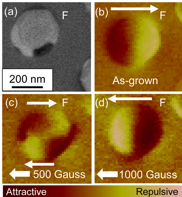
FIG. 5. (a) BSE image of ND-F and the applied magnetic field dependence of the magnetic domain structure of ND-F: (b) as-grown, i.e., B = 0 , (c) 500, and (d) 1000 G. The thick and thin white arrows indicate the directions of the applied magnetic field, B , and the magnetization directions of the MnAs NDs, respectively. At B = 500 G, a change in the domain structure to two magnetic domains from a single domain is observed. At B = 1000 G, the magnetization direction of MnAs ND is completely reversed parallel to the direction of the applied magnetic field, B .
