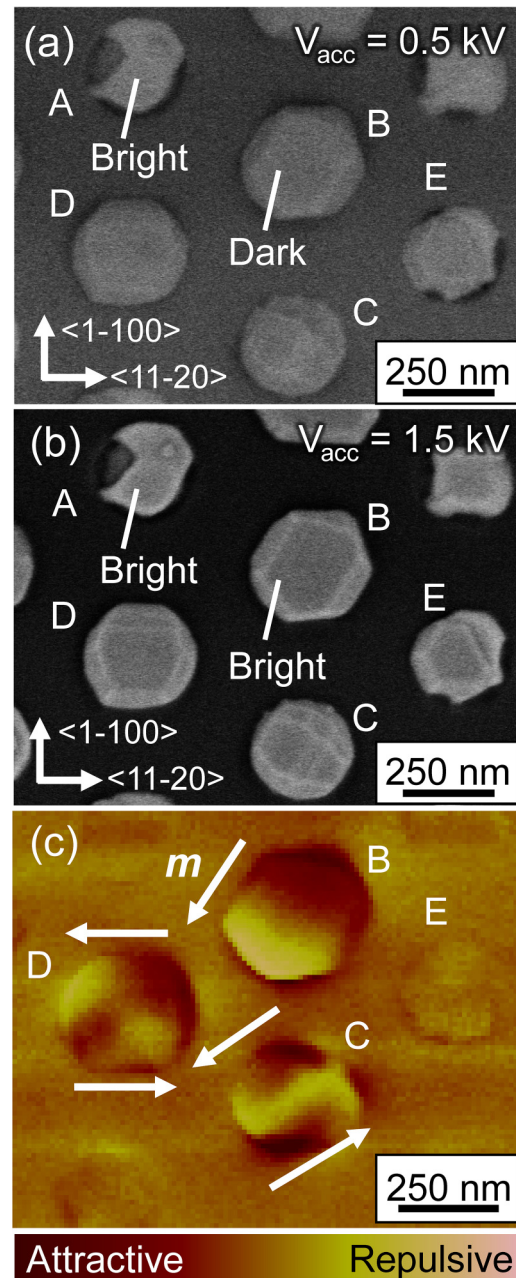
FIG. 1. Acceleration voltage dependence of BSE images of MnAs NDs on AlGaAs NP buffers: (a) 0.5 and (b) 1.5 kV. In (a), a relatively bright image contrast of ND-A and an image contrast of ND-B darker than the one of ND-A are observed. In (b), almost no significant difference in the image contrasts between ND-A and ND-B is observed. (c) MFM image of the corresponding MnAs NDs and AlGaAs NP buffers. The MFM observations were carried out at room temperature without any application of an external magnetic field. Most of the MnAs NDs show a spontaneous magnetization. A single magnetic domain is observed in ND-B, and multiple magnetic domains are observed in ND-C and ND-D. The white arrows in (c) indicate the directions of the magnetic moments ( m ) in the NDs. No well-defined contrast is observed in the MFM image of ND-E.
