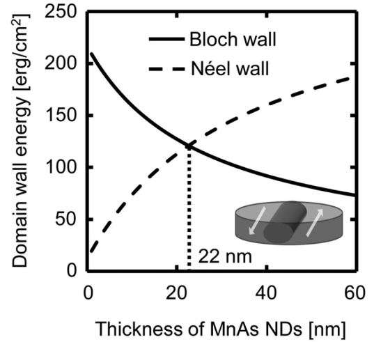
FIG. 4. Calculated wall energy density per unit area of the domain walls as a function of the MnAs thickness. The Bloch wall energy is equal to the Néel wall energy at a ND thickness of approximately 22 nm, which is in good agreement with the thickness of 20 nm roughly estimated from the acceleration voltage dependence of the BSE images of the MnAs NDs.
