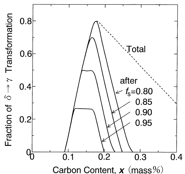
Fig. 10 Relationship between carbon content and the amount of austenite phase transformed after the solid fraction reached high values. Cooling rate is 0.01 K/s.
