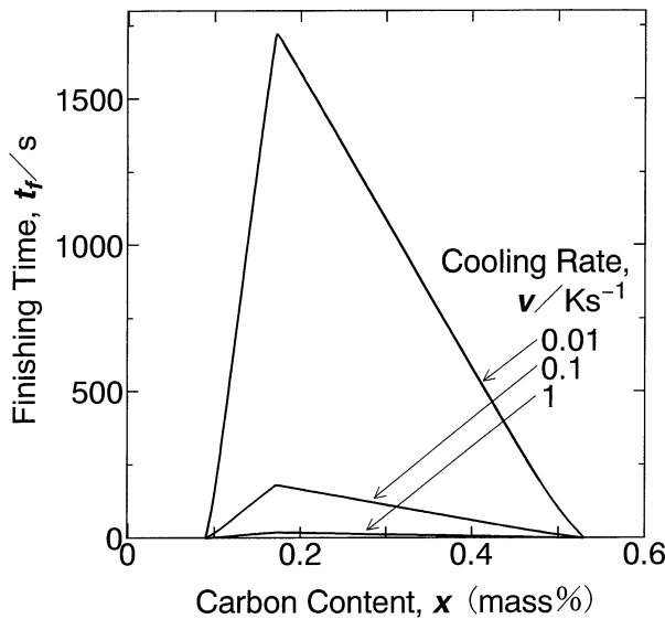
Fig. 11 Effect of carbon content on the finishing time of the peritectic transformation.
