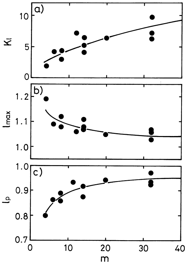
Fig. 3. Relation between m and K_l (a), l_{\text{Max}} (b) and l_p (c). m : number of faces of a polyhedron, K_l : maximum probability density, l_{\text{Max}} : maximum relative diameter, l_p : peak position in the distribution.
