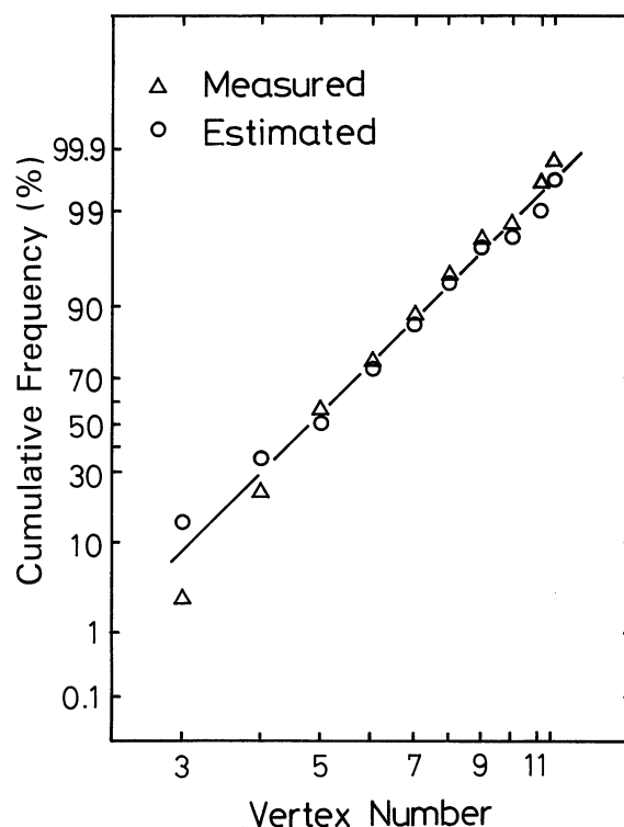
Fig. 8 Cumulative frequency of the vertex number of grains on the cross section.
