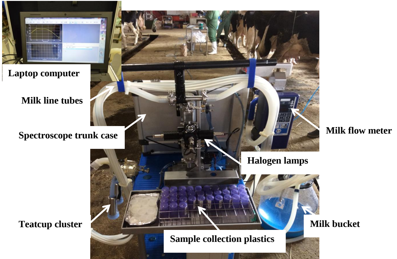
Figure 3.1 Overview of the NIR spectroscopic sensing system
