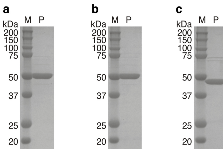
Figure 2.4 Expression and purification of recombinant XOO_1319, XOO_1320, and MurD.
