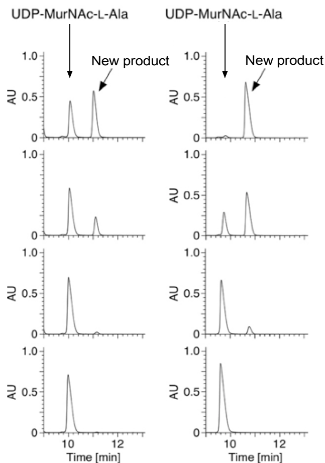
Figure 2.12 Glu ligase assay with recombinant XOO_1320 using L-Glu as a substrate.
