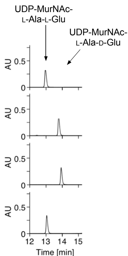
Figure 2.15 UDP-MurNAc-L-Ala-L-Glu epimerase activity of recombinant XOO_1319.
