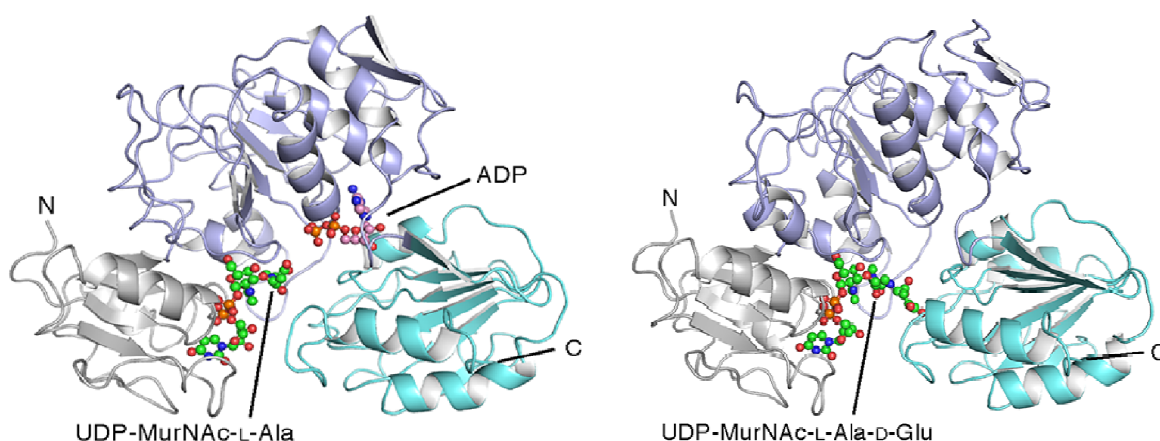
Figure 3.1 Ribbon representations of overall structures of the MurD2 model of the substrate-binding state (left) and its product-binding state (right). The N -terminal, central, and C -terminal domains are colored in gray, blue, and cyan, respectively. UDP-MurNAc-L-Ala and ADP bound to the MurD ec quaternary complex structure and UDP-MurNAc-L-Ala-D-Glu bound to the MurD ec tertiary complex structures are shown with the MurD2 models.
