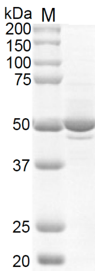
Figure 3.12 SDS-PAGE analysis of recombinant MurD sm _T192E (51.1 kDa). M, marker
