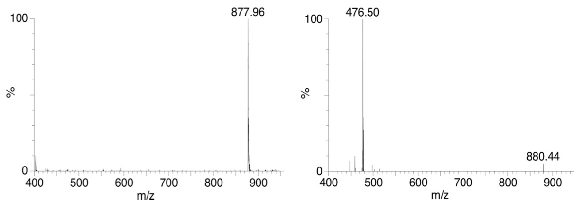
Figure 2.16 MS spectra of the product formed from UDP-MurNAc-L-Ala-L-Glu with recombinant XOO_1319
