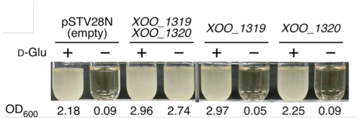
Figure 2.3 Complementation assay of the D-Glu auxotrophic E. coli mutant with subcloned plasmids.
