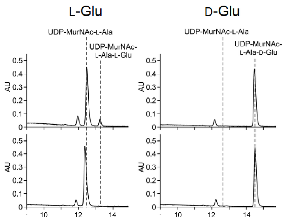
Figure 3.16 UDP-MurNAc-L-Ala-Glu synthetase activities of recombinant MurD ec and MurD sm _K319T mutant with UDP-MurNAc-L-Ala and L-Glu (left column) or D-Glu (right column) as the substrates. HPLC traces (260 nm) of the reaction products formed with K319T mutant (top) and wild type (bottom) are shown.
