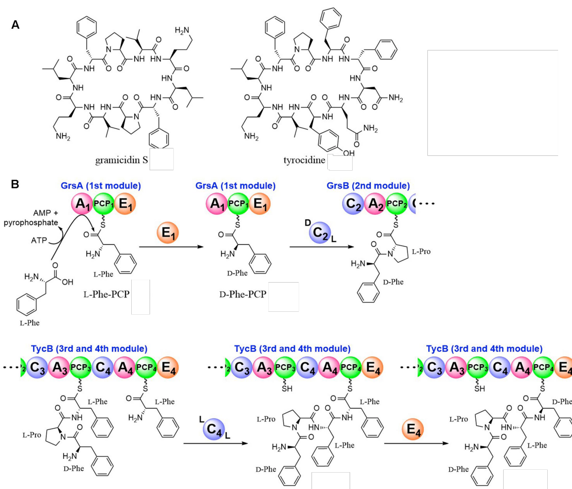
Figure 1.4 Epimerization in NRPS
