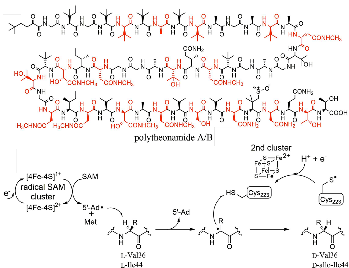
Figure 1.5 Structures of polytheonamide A/B (differing in sulfoxide configuration) and reaction mechanism proposed for rSAM dependent epimerase. Amino acid residues with D-configuration are shown in red.
