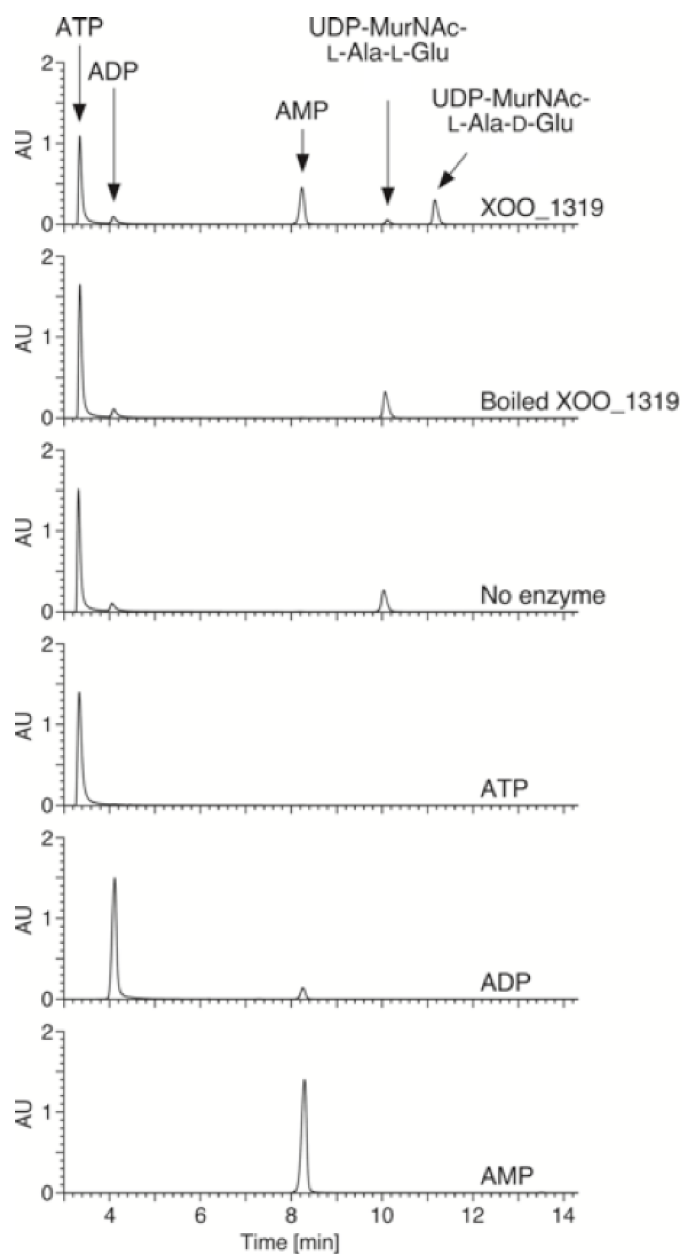
Figure 2.18 Substrate-activation mechanism of XOO_1319.
