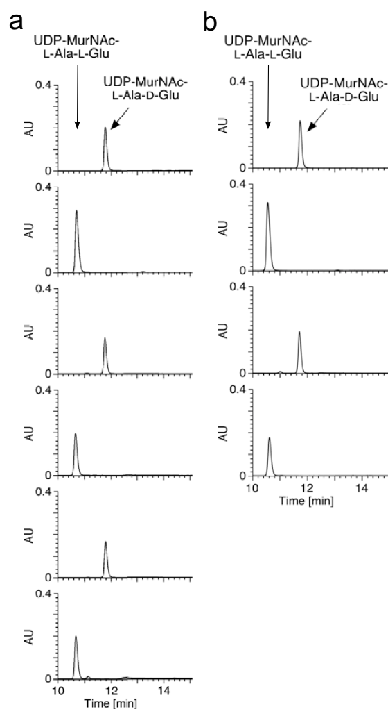
Figure 2.22 Glu epimerase activities of XOO_1319 orthologs.
