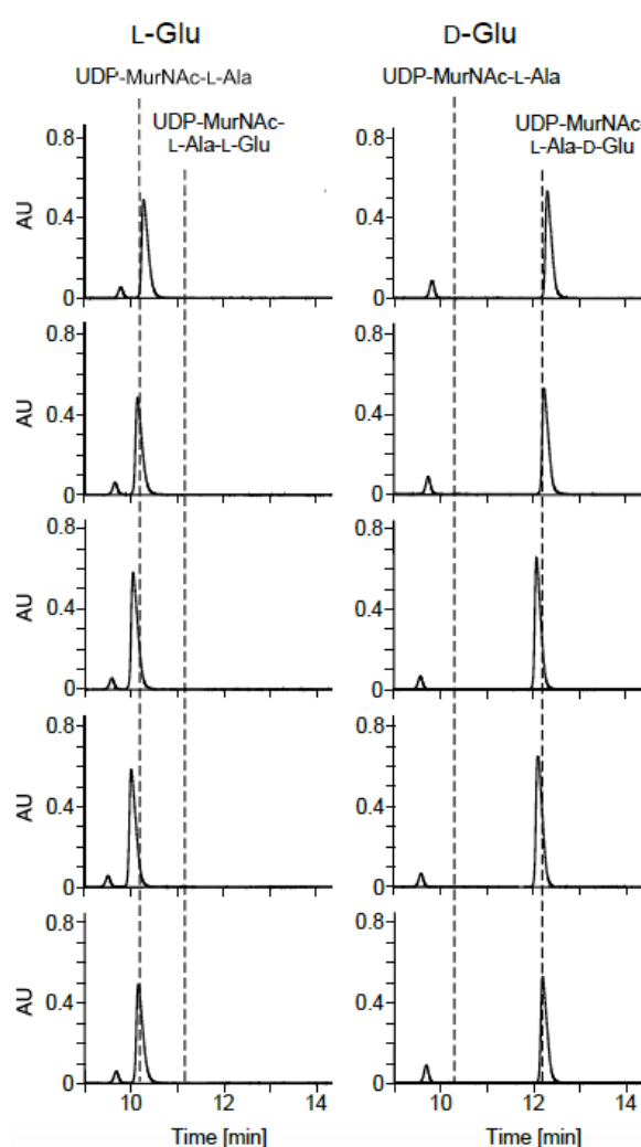
Figure 3.8 UDP-MurNac-L-Ala-Glu synthetase activities of recombinant MurD ec and its mutants with UDP-MurNac-L-Ala and L-Glu (left column) or D-Glu (right column) as the substrates.
