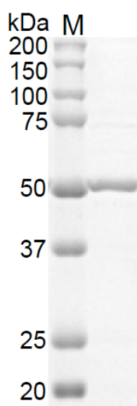
Figure 3.10 SDS-PAGE analysis of purified recombinant MurD sm (51.1 kDa). M, marker
