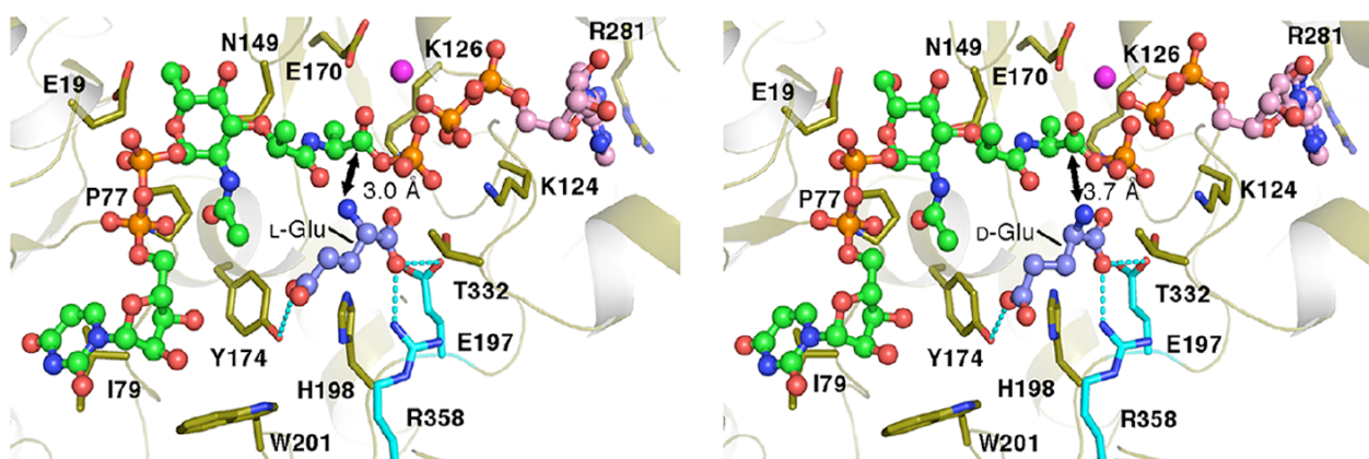
Figure 3.6 Close-up views of the active site cavity of the MurD2 quinary complex models with UDP-MurNAc-L-Ala-phosphate, ADP, Mg 2+ , and L-Glu (left) or D-Glu (right).
