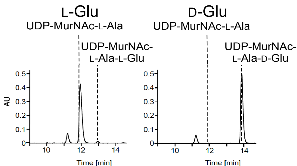
Figure 3.11 UDP-MurNAc-L-Ala-Glu synthetase activities of recombinant MurD sm with UDP-MurNAc-L-Ala and L-Glu (left column) or D-Glu (right column) as the substrates.
