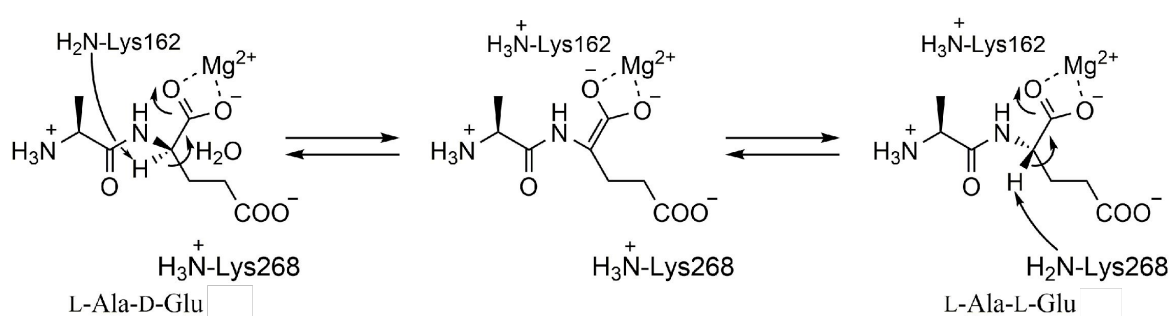
Figure 1.3 Reaction of L-Ala-D/L-Glu epimerases.
