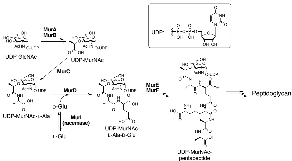
Figure 1.2 Peptidoglycan biosynthetic pathway
