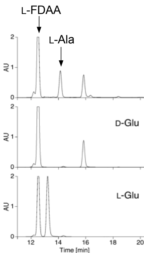
Figure 2.17 Chiral analysis of the terminal Glu residue of the reaction product formed from UDP-MurNAc-L-Ala-L-Glu by recombinant XOO_1319 (upper).
