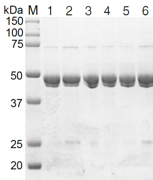
Figure 3.7 SDS-PAGE analysis of purified recombinant MurD ec and its mutants (48.2 kDa).
