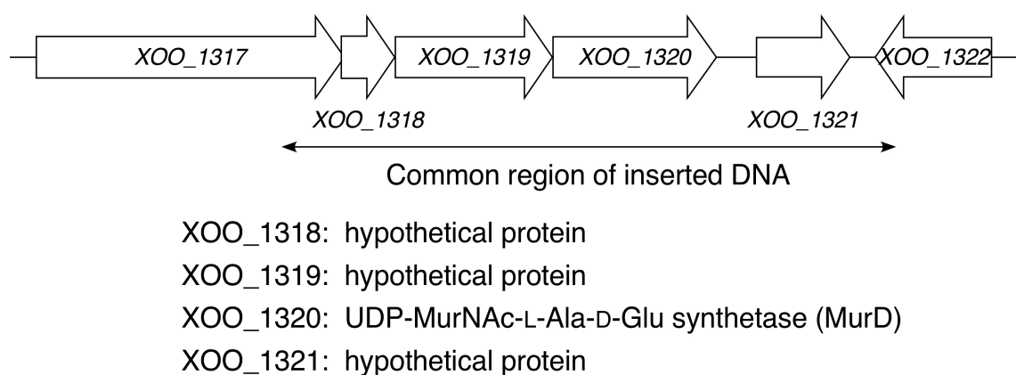
Figure 2.2 DNA regions complementing the D-Glu auxotrophic E. coli mutant.
