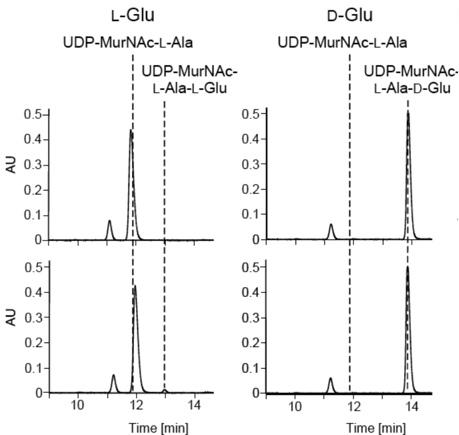
Figure 3.13 UDP-MurNac-L-Ala-Glu synthetase activities of recombinant MurD sm and its mutant with UDP-MurNac-L-Ala and L-Glu (left column) or D-Glu (right column) as the substrates.
