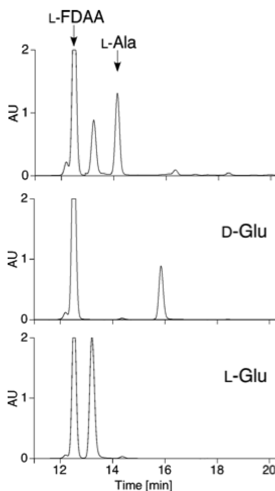
Figure 2.14 Chiral analysis of the terminal Glu residue of the reaction product formed from UDP-MurNAc-L-Ala and L-Glu by recombinant XOO_1320 (upper). L-FDAA derivative of Glu released by acid hydrolysis of the reaction product was analyzed by HPLC with detection at UV 340 nm. The standards, D-Glu (middle) and L-Glu (lower), were also analyzed.
