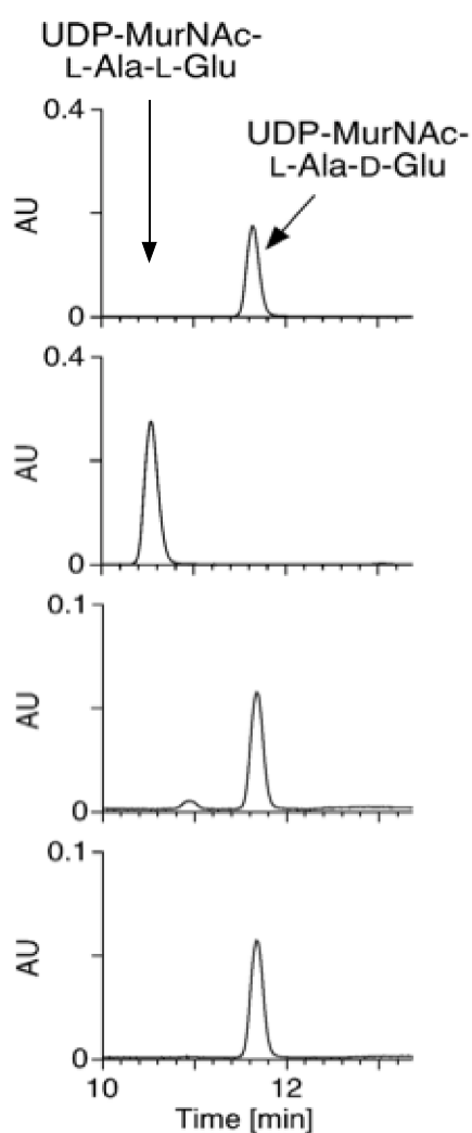
Figure 2.19 UDP-MurNAc-L-Ala-D-Glu epimerase activities with recombinant XOO_1319.
