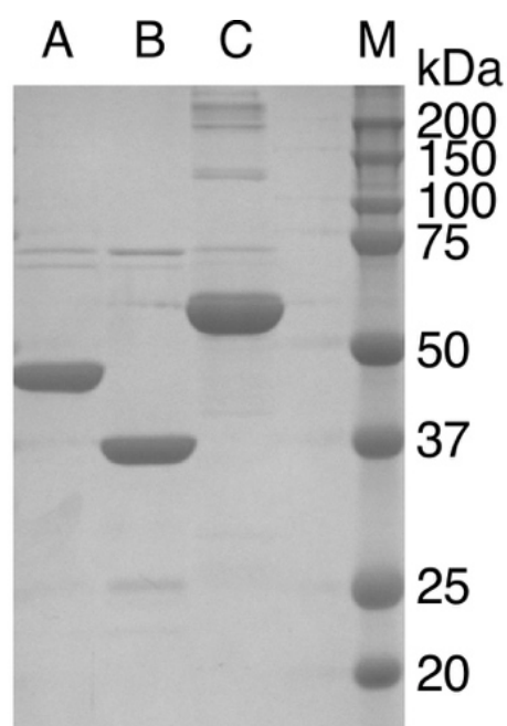
Figure 2.5 Expression and purification of recombinant MurA, MurB, and MurC of E. coli .
