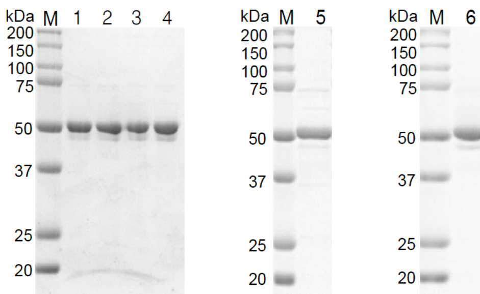
Figure 3.3 SDS-PAGE analysis of purified recombinant MurD2 and its mutants (51.9 kDa).
