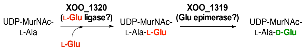
Scheme 2.2 Proposed peptidoglycan biosynthetic pathway by L-Glu ligase and epimerase
