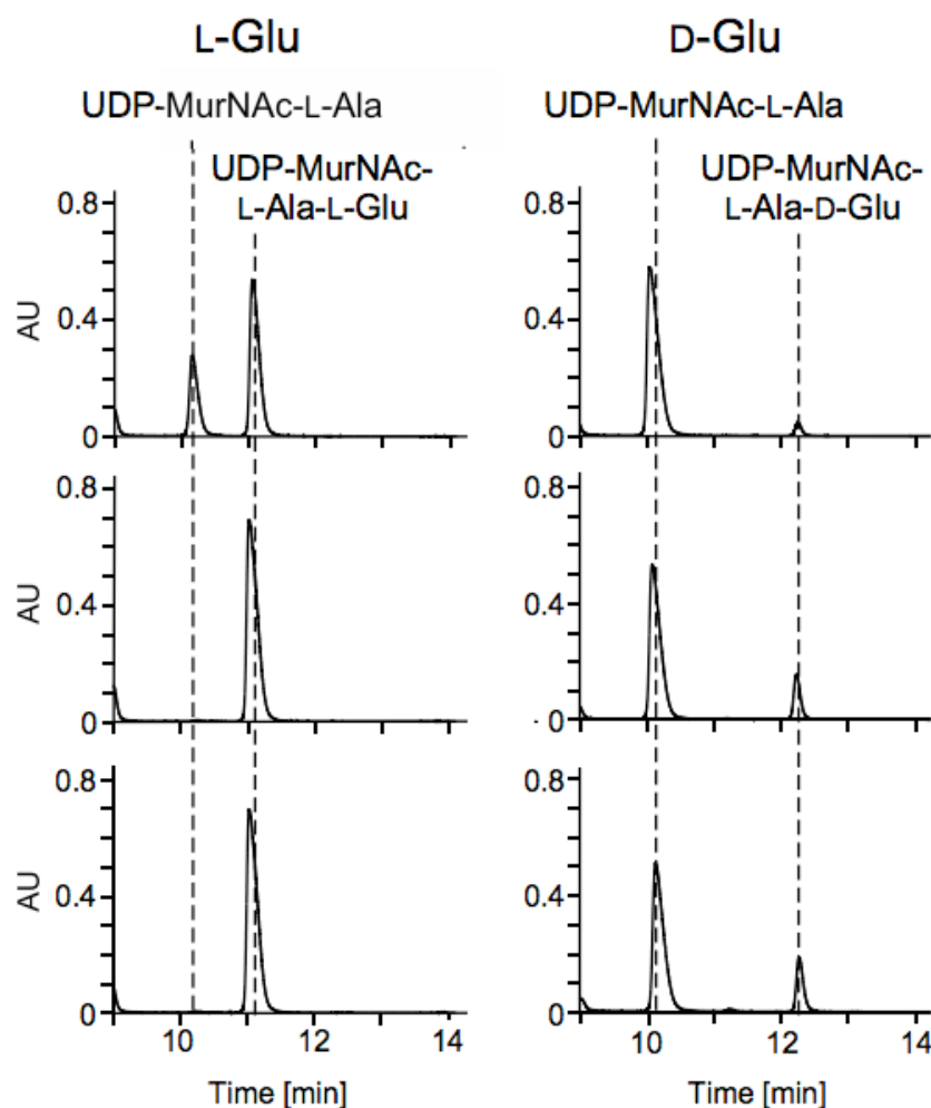
Figure 3.4 UDP-MurNac-L-Ala-Glu synthetase activities of recombinant MurD2 and its mutants with UDP-MurNac-L-Ala and L-Glu (left column) or D-Glu (right column) as the substrates.
