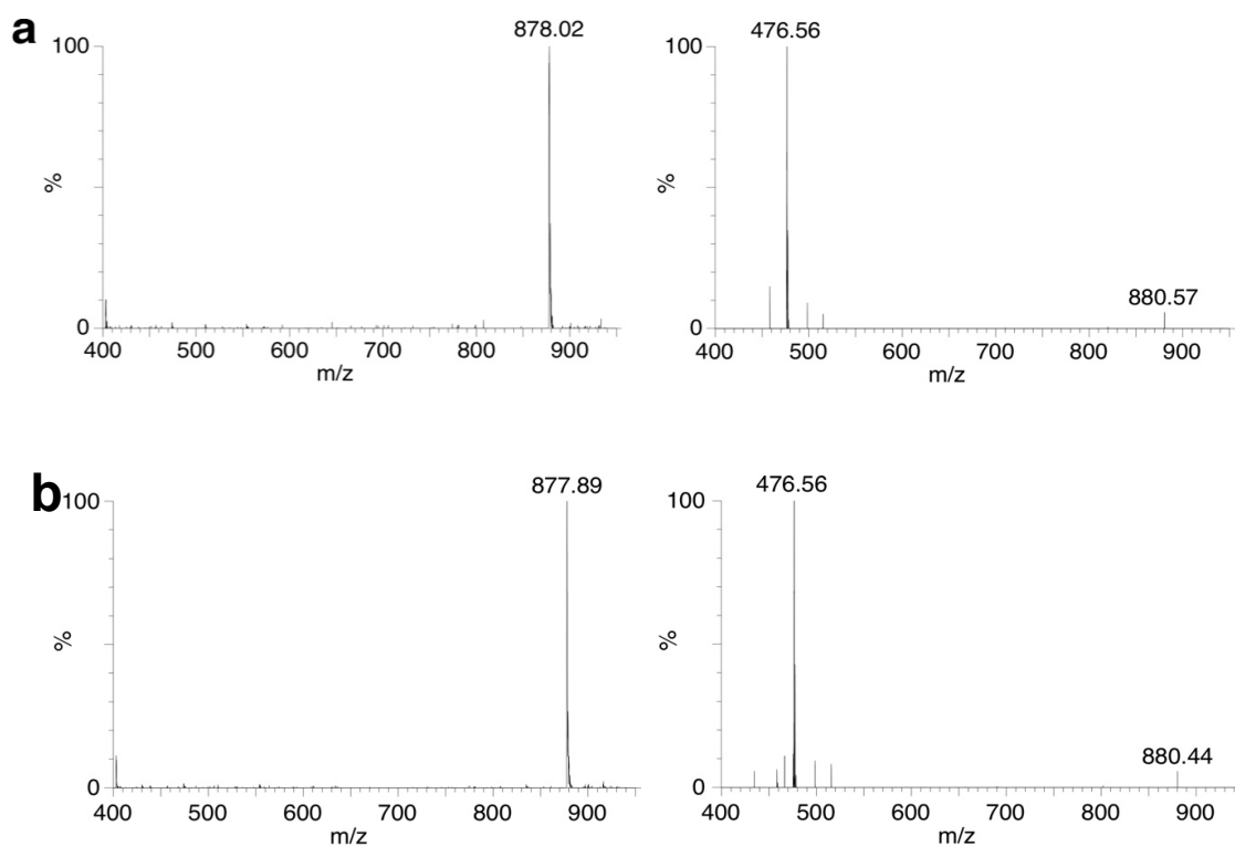
Figure 2.13 MS spectra of UDP-MurNAc-L-Ala-Glu formed by recombinant XOO_1320 and MurD.
