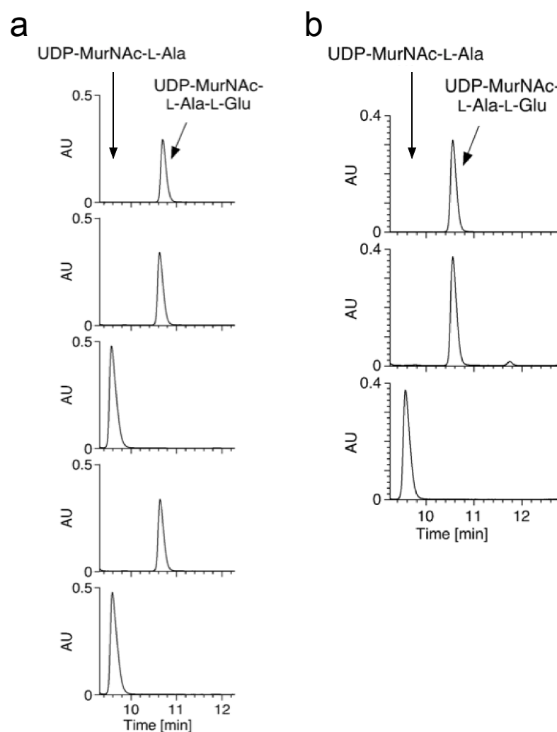
Figure 2.21 UDP-MurNAc-L-Ala-L-Glu ligase activities of XOO_1320 orthologs. (a) HPLC trace of the standard of UDP-MurNAc-L-Ala-L-Glu, reaction products with Strop_3005, boiled Strop_3005, MCAG_01009, or boiled MCAG_01009 are shown (from top to bottom). (b) HPLC trace of the standard UDP-MurNAc-L-Ala-L-Glu, the reaction products with DP16_1119, or boiled DP16_1119 are shown (from top to bottom)
