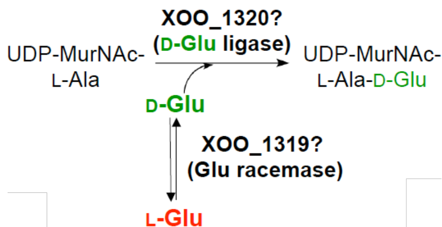
Scheme 2.1 Proposed peptidoglycan biosynthetic pathway by racemase and D-Glu ligase.
