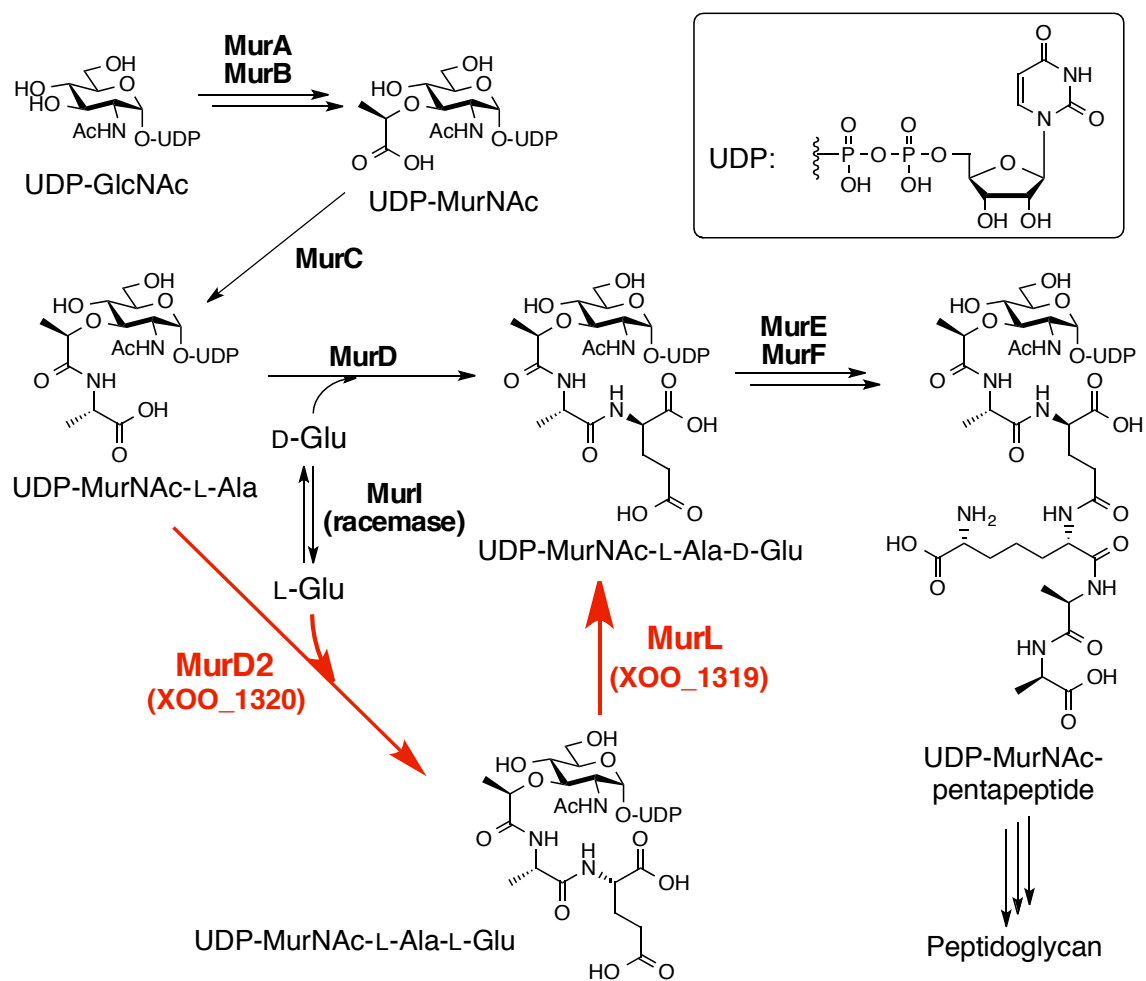
Figure 2.23 Peptidoglycan biosynthetic pathways of MurD/MurI and MurD2/MurL.
