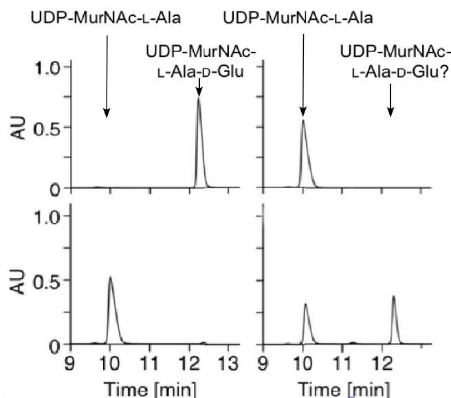
Figure 2.9 UDP-MurNAc-L-Ala-L/D-Glu synthetase activities.
