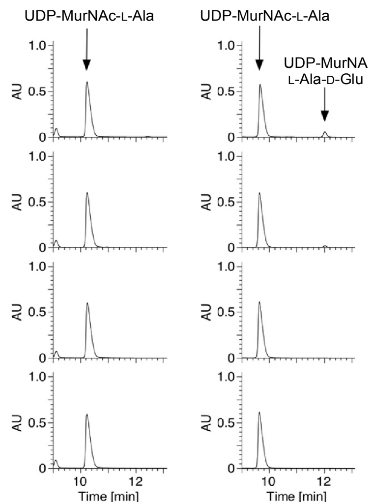
Figure 2.8 Glu ligase assay with recombinant XOO_1320 using D-Glu as substrate. HPLC traces of the reaction products formed with 50, 17, and 5.6 \mu\text{g mL}^{-1} (0.96, 0.32, and 0.11 \mu\text{M} ) of XOO_1320 and boiled XOO_1320 (from top to bottom) after 5 min (left column) and 2 h (right column) reaction times are shown.
