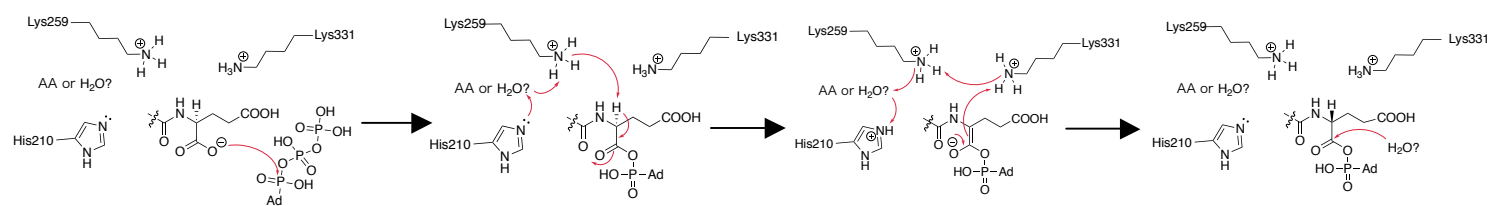
Figure 2.24 Proposed reaction mechanism of MurL
