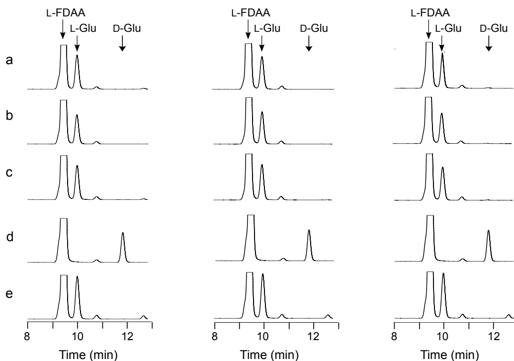
Figure 2.7 Racemase assay with recombinant XOO_1319.
