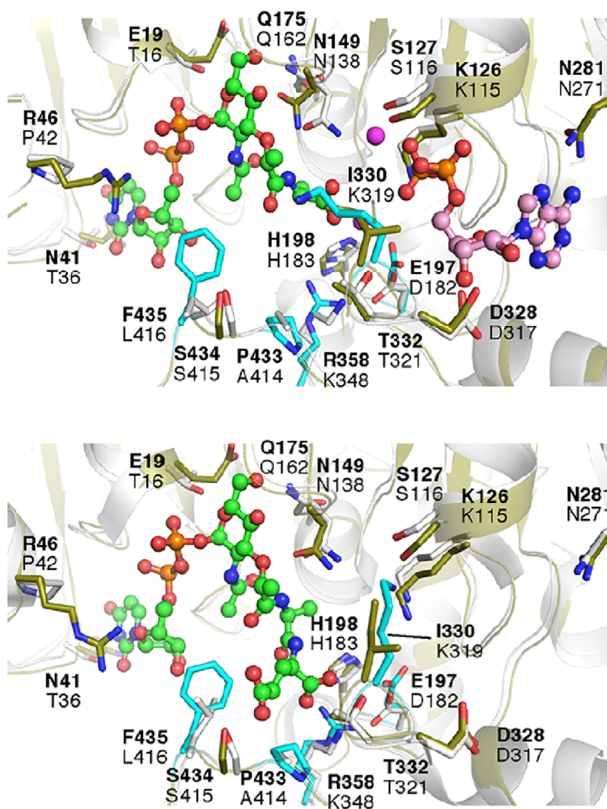
Figure 3.2 Comparisons of the active site cavities of the MurD2 models of the substrate-binding state (top) and its product-binding state (bottom) with those of the MurD ec quaternary and tertiary complex structures, respectively.
