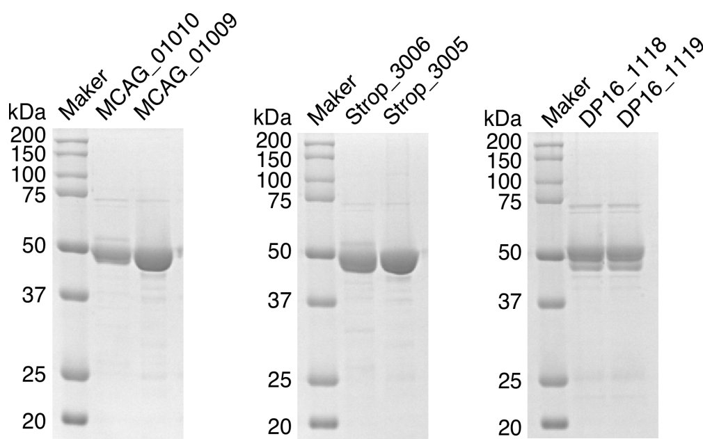
Figure 2.20 Expression and purification of recombinant MCAG_01009, MCAG_01010, Strop_3005, Strop_3006, DP16_1118, and DP16_1119. SDS-PAGE analysis of purified MCAG_01009 (49.8 kDa), MCAG_01010 (50.4 kDa), Strop_3005 (49.1 kDa), Strop_3006 (51.2 kDa), DP16_1118 (51.9 kDa), and DP16_1119 (52.0 kDa).
