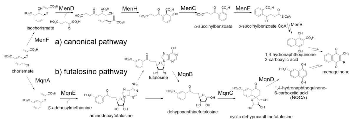
Figure 1.1 Two distinct biosynthetic pathways of menaquinone. (a) The canonical pathway (b) The futalosine pathway
