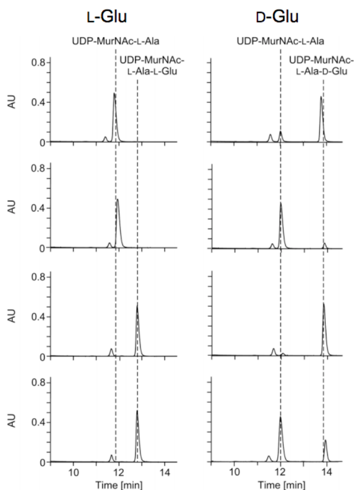
Figure 3.5 UDP-MurNac-L-Ala-Glu synthetase activities of recombinant MurD2 and its mutants with UDP-MurNac-L-Ala and L-Glu (left column) or D-Glu (right column) as the substrates.
