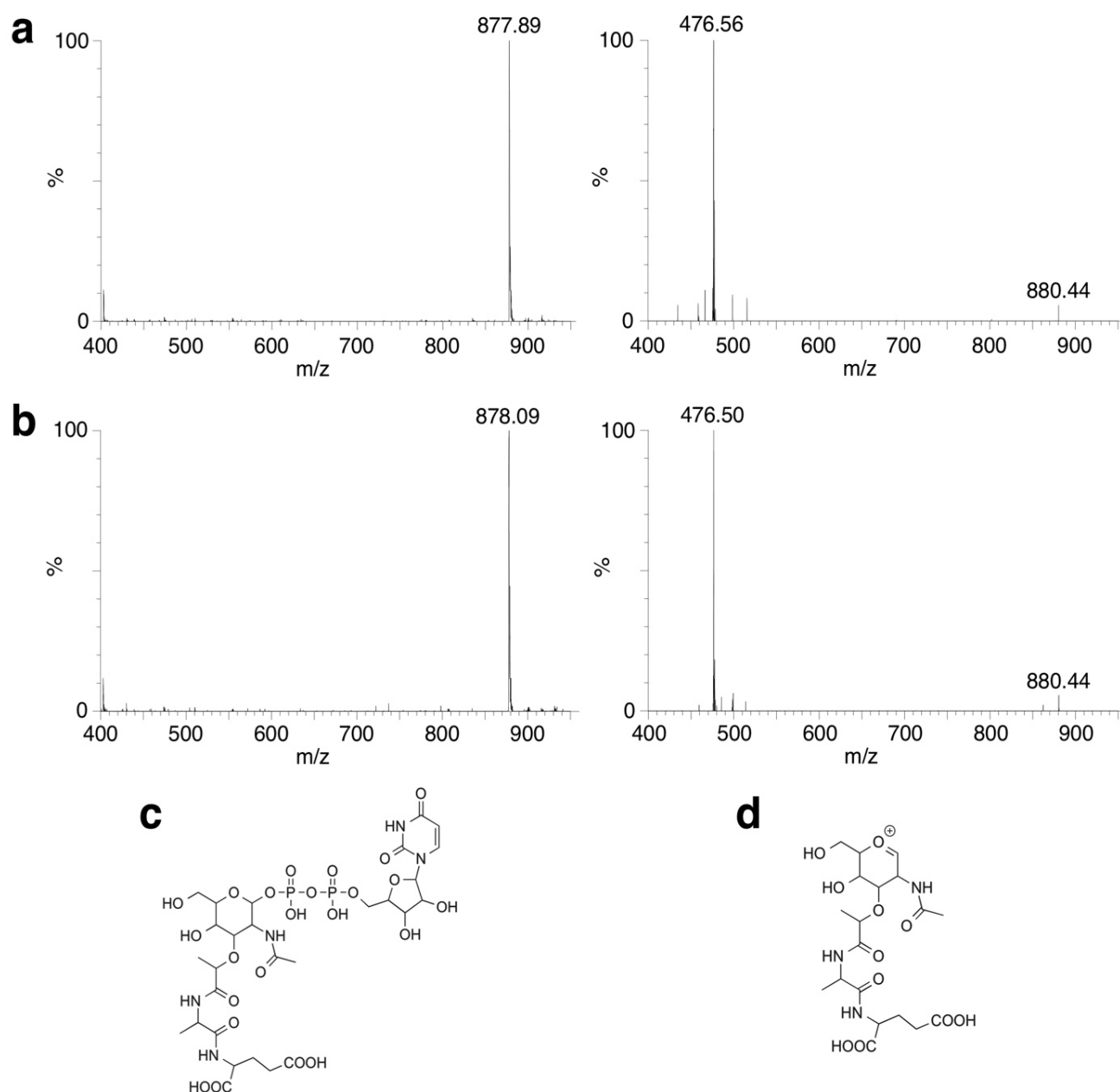
Figure 2.10 Mass spectra of the reaction products of MurD and a mixture of XOO_1319 and XOO_1320.
