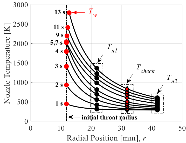
Figure 44. Check thermocouple supports TTRT results of MSS-5.
