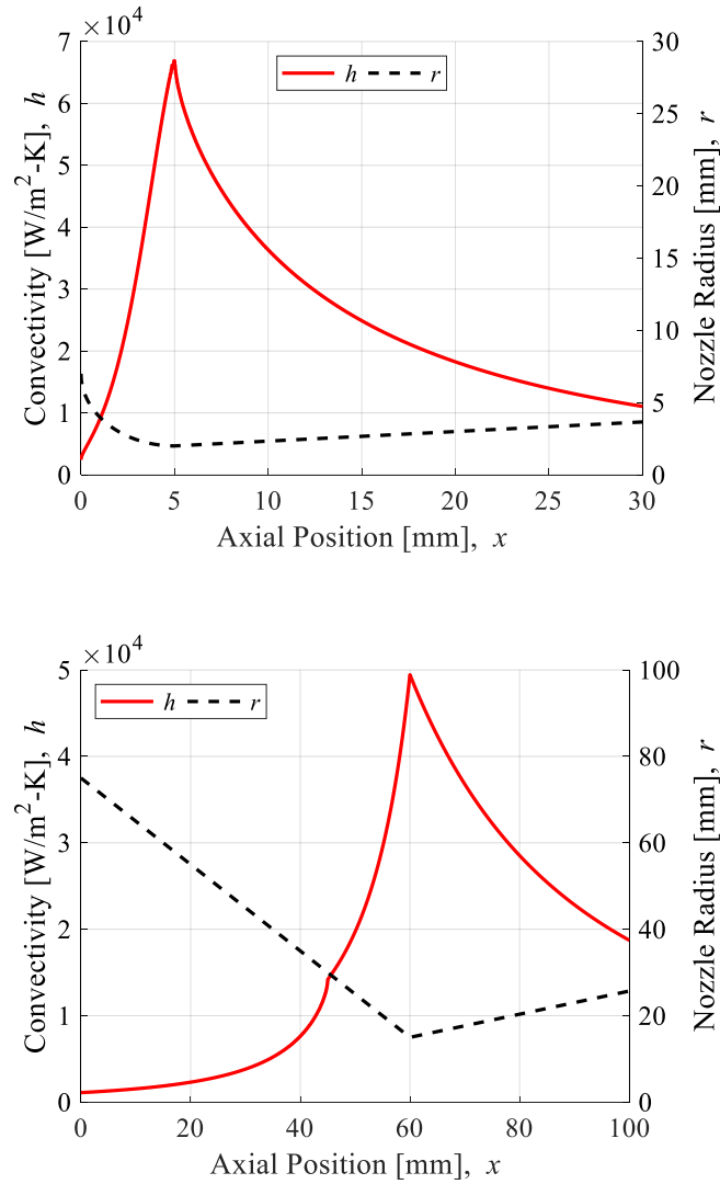
Figure 43. Sharp increase in heat transfer coefficient at the nozzle throat in: (upper) sharp circular inlet ; (lower) gradual conical inlet . P_c = 3 MPa; \Phi = 1 ; LOX/HDPE.
