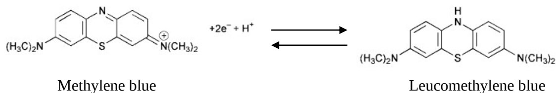
Figure 2-1. Reduction-oxidation reaction of methylene blue
