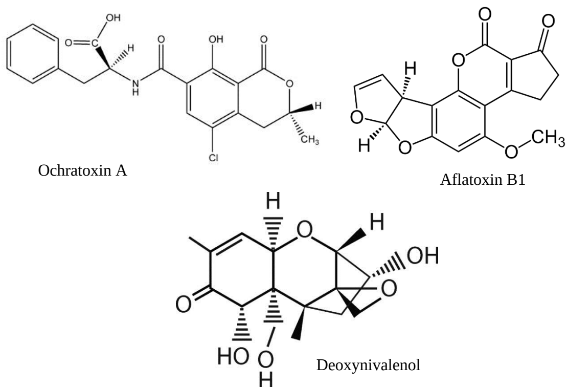
Figure 3-11. Chemical structure of OTA, AFB1 and DON
