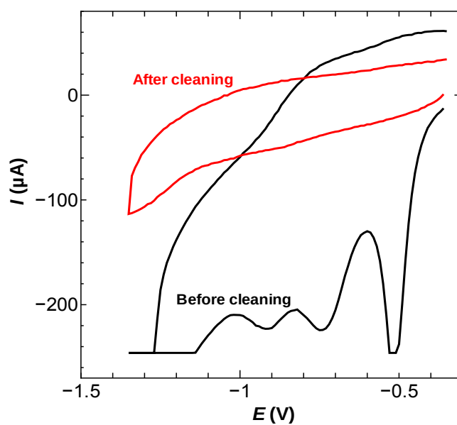
Figure 2-7. Potential scanning under basic condition (0.5 M NaOH) to clean the electrode before sensor fabrication. Voltammogram before cleaning (black) and after 200 times scanning completion (red) is shown.
