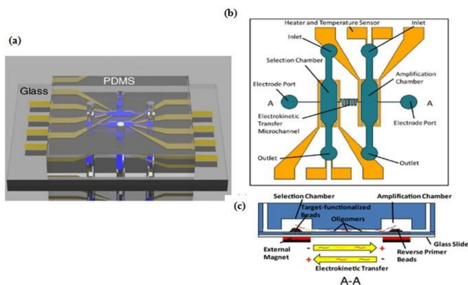
Figure 1-2. Schematic of microfluidic SELEX device which integrates selection and amplification steps. (a) Polydimethylsiloxane (PDMS) channel on glass substrate; (b) Top view with detailed features; (c) Selection and amplification microchamber connected by a single serpentine shaped microchannel. Reproduced with permission from reference [17]. Copyright 2017 Electrochemical Society
