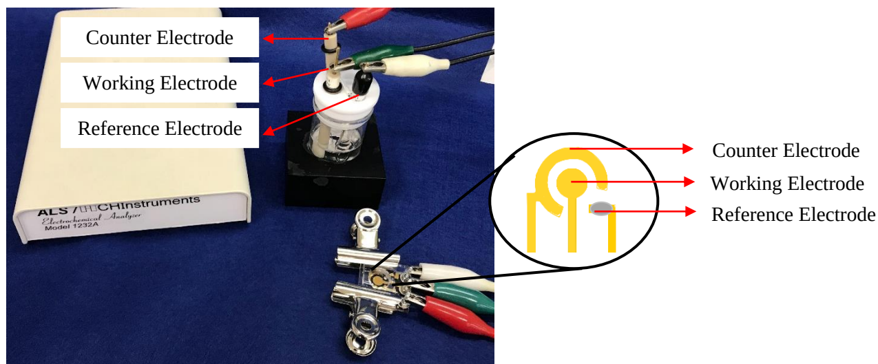
Figure 3-2. The electrochemical system used in this study contains an ALS 1232a electrochemical analyzer, conventional electrodes, and the microfabricated electrodes.
