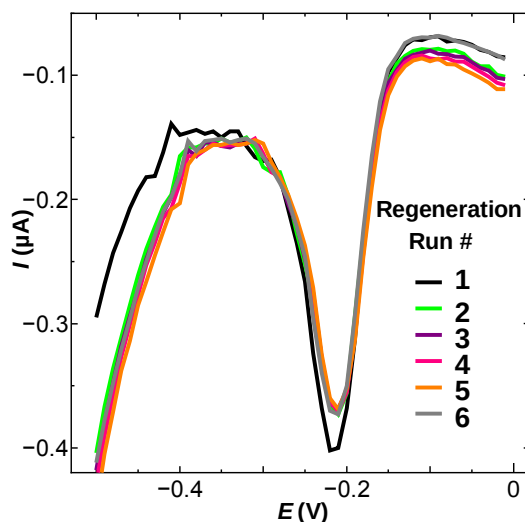
Figure 2-15. Signal responses for six times regeneration of sensor.
