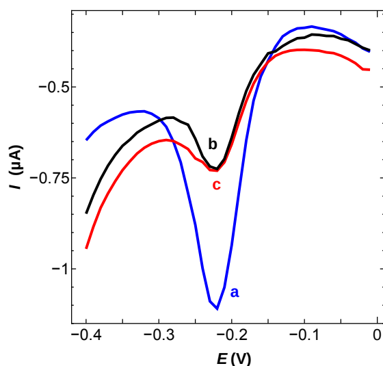
Figure 2-14. Selectivity of the sensor to (a) 0 \text{ng mL}^{-1} OTA and 0 \text{ng mL}^{-1} AFB1, (b) 50 \text{ng mL}^{-1} OTA and 50 \text{ng mL}^{-1} AFB1, and (c) 50 \text{ng mL}^{-1} OTA.
