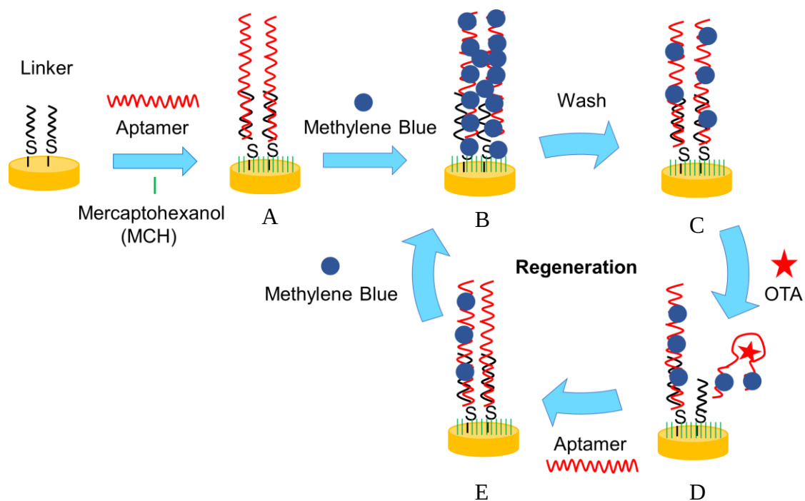
Figure 2-5. Schematic illustration of the modification of the electrode, detection of OTA, and regeneration of the sensor.
