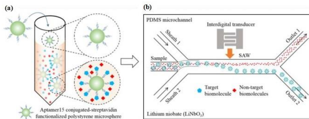
Figure 1-10. (a) Specific aptamer to form a microparticle–aptamer–target complex; the unbound particles remained in a free condition; (b) Separation process of the mixture solution through an acoustofluidic device. Reproduced with permission from reference [100]. Copyright 2017 American Chemical Society.
