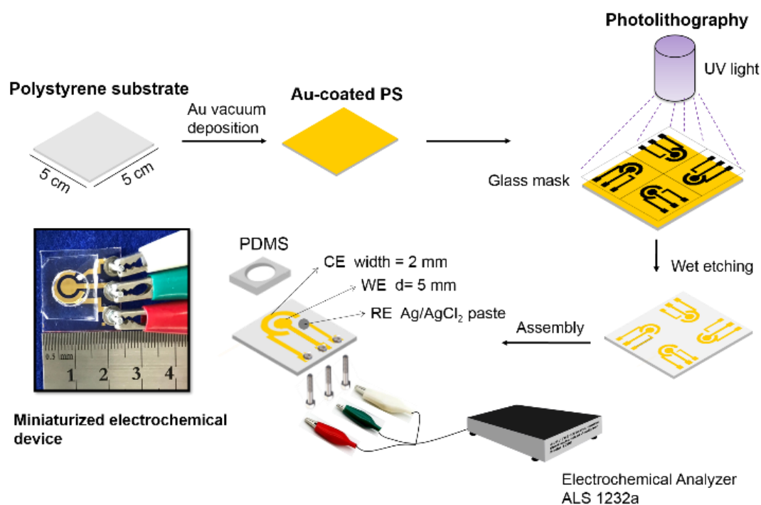
Figure 2-2. Schematic diagram for the fabrication of a miniaturized electrode for the present sensor and its experimental setup.
