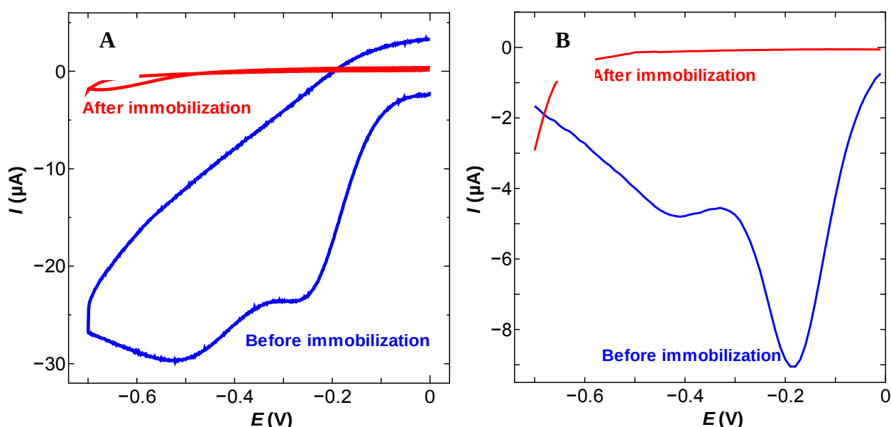
Figure 2-8. Background currents measured with electrodes before and after modification without MB by (A) cyclic voltammetry (CV) and (B) differential pulse voltammetry (DPV). The voltammograms were obtained in PBS buffer containing 1 mM MgCl.
