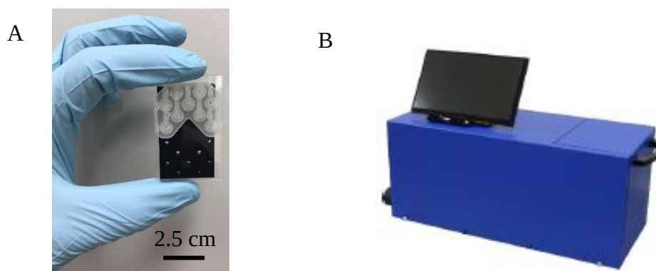
Figure 4-2. (A) Microdevice chip enable to detect up to nine samples simultaneously. (B) Miniaturized fluorescence polarization analyzer
