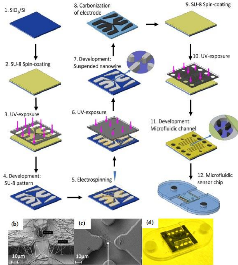
Figure 1-7. Fabrication steps of the carbon nanowire aptasensor. (a) The device was fabricated by integrating electrospinning and photolithography with carbon-microelectromechanical system (C-MEMS) technique; (b) Electrospun SU-8 nanowire; (c) Single SU-8 nanowire after photolithography and development; (d) Microfluidic platform containing the nanowire sensor. Reproduced with permission from reference [72]. Copyright 2018 Elsevier.
