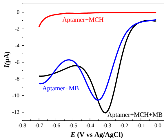
Figure 3-5. The effect of MCH to the dithiol modified aptamer on the electrode surface
