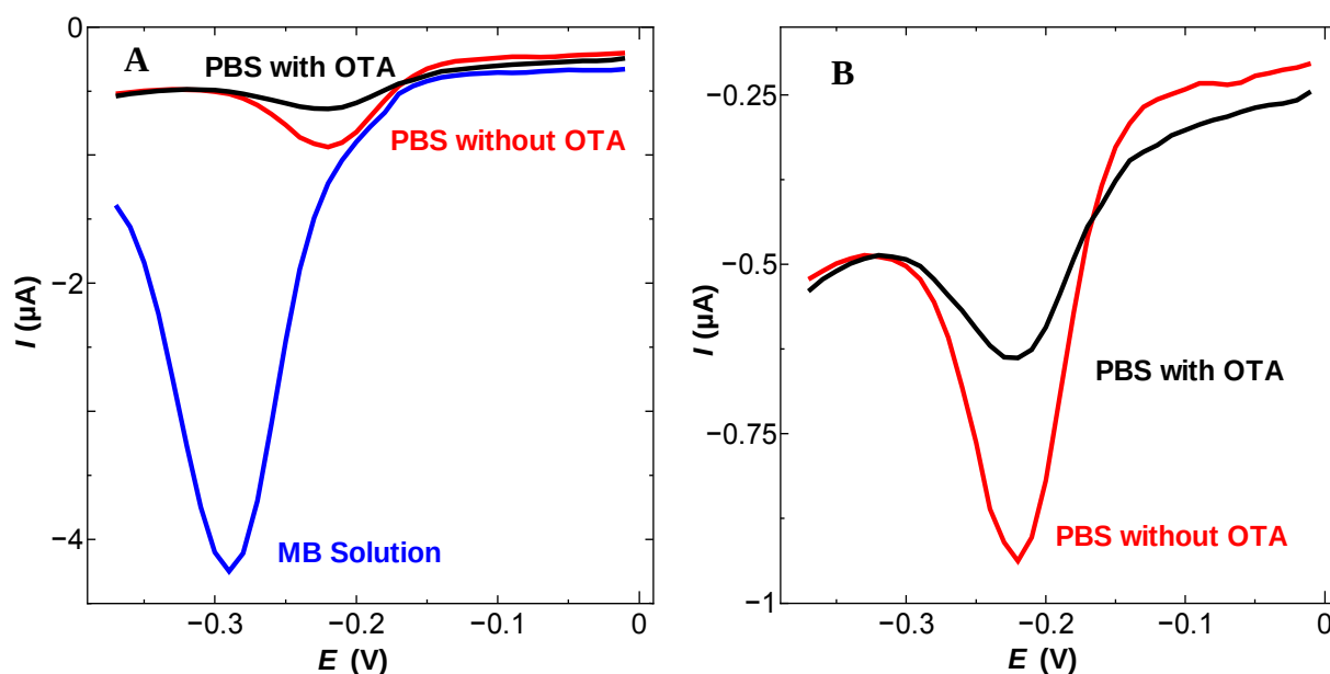
Figure 2-9. DPV curves of the sensor obtained with MB solution (blue curve), PBS buffer without OTA (red curve), and PBS buffer containing 100 \text{ ng mL}^{-1} OTA (black curve). (B) Enlarged view of the curve for PBS with and without OTA in (A). Specific peak potential ( -0.22 \text{ V} vs Ag/AgCl) and the gap of currents indicates the presence of OTA.
