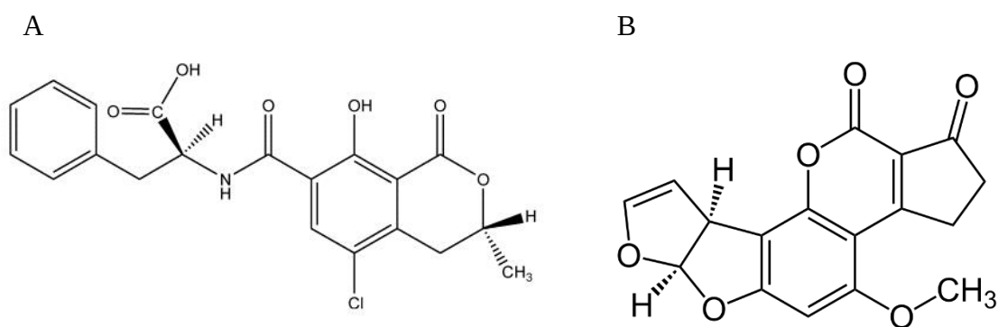
Figure 2-13. Chemical structure of (A) ochratoxin A and (B) aflatoxin B1
