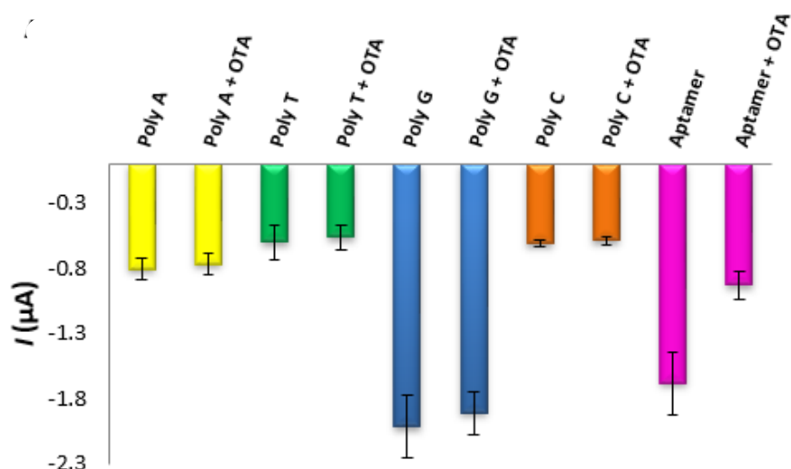
Figure 2-12. Selectivity test with Poly-C, Poly-G Poly-T, and Poly-A. All these oligonucleotides were treated under the same conditions as the aptamer.
