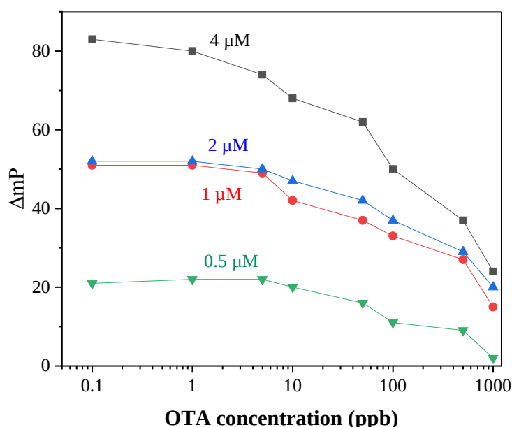
Figure 4-4. FP intensity dependencies of aptamer concentration from 0.5 \mu\text{M} to 4 \mu\text{M} . The higher intensity was reached with aptamer concentration 4 \mu\text{M} .
