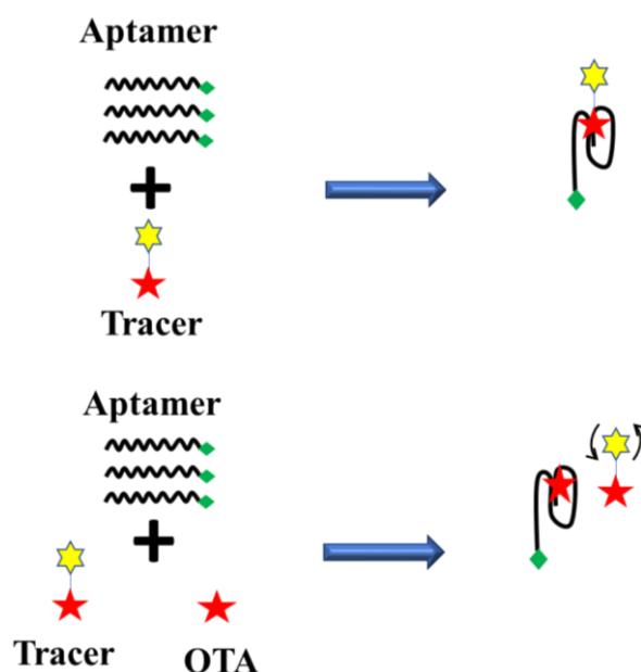
Figure 4-1. Working principle of competitive FPAA method for OTA detection. In the absent of OTA, all the aptamer will bind with tracer resulting high P value (above). However, when the target was present, the tracer and OTA competitively bind to the aptamer (below) and the P value depends on the OTA concentration.
