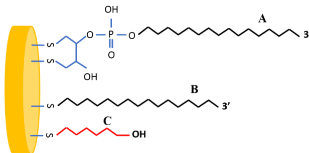
Figure 3-4. Modification of the gold surface with (A) dithiol based-aptamer, (B) monothiol based-aptamer, and (C) 6-mercaptohexanol.
