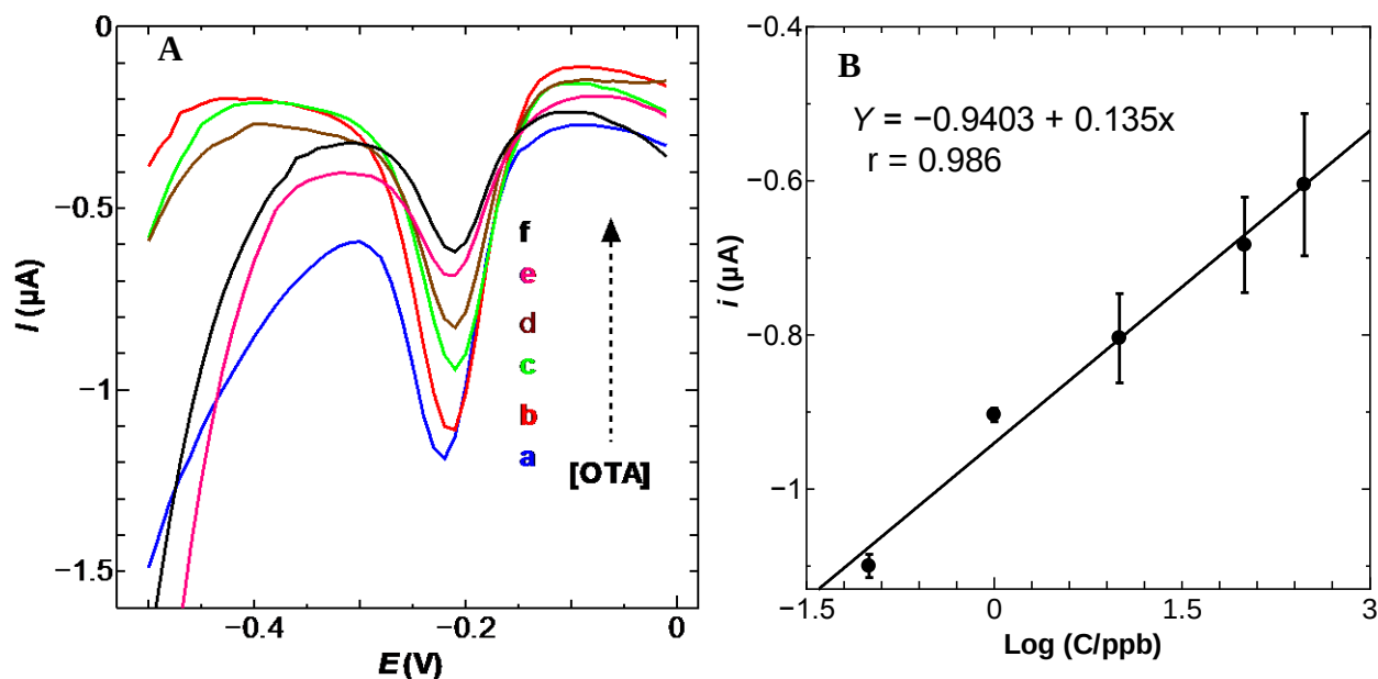
Figure 2-10. (A) Current responses measured by DPV at various concentrations of OTA: (a) 0, (b) 0.1, (c) 1, (d) 10, (e) 100, (f) 300 \text{ng mL}^{-1} . (B) Plot of current vs logarithmic concentration of OTA. Error bars represent \pm standard deviations of means ( n = 3 ).
