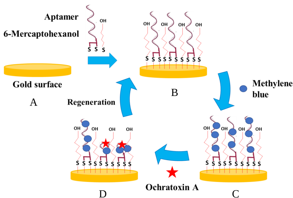
Figure 3-3. Schematic illustration of the modified electrode based on structure switching signal-on aptasensor and sensor regeneration.
