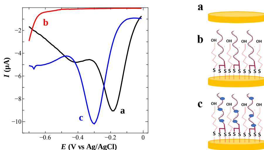
Figure 3-9. The current responses obtained before and after electrode modification: a) bare electrode; b) aptamer-and MCH modified electrode; c) MB-modified electrode. These responses were obtained in PBS containing 1 mM \text{MgCl}_2 .
