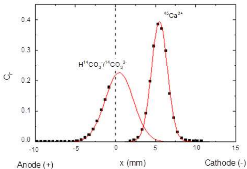
Figure 3-3. Spatial distribution of relative concentration of ^{45}Ca^{2+} and H^{14}CO_3^- / ^{14}CO_3^{2-} ions after 6 hours of electromigration experiment with constant electrical current of 15 mA. The initial positions of radiotracers are at x = 0 . The solid lines are the least square fit of the concentration profile of each ion.
