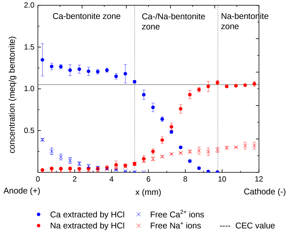
Figure 2-2. Spatial distribution of \text{Ca}^{2+} and \text{Na}^{+} ions in compacted montmorillonite after 16 hours of electromigration experiment. The free \text{Ca}^{2+} and \text{Na}^{+} ions are their respective concentration from extraction with saturated \text{CaCO}_3 solution. The figure has the plotting concentrations (meq/g-dry bentonite) per sliced bentonite sample versus the position of the distance of the center of each slice from the anode side. The acid extractable \text{Ca}^{2+} and \text{Na}^{+} from sequential extraction are the concentration of \text{Ca}^{2+} and \text{Na}^{+} ions as exchangeable cations and solid phases. The horizontal straight line is the CEC value of bentonite sample which equals 1.05 meq/g-dry bentonite. The error bars are calculated from the standard deviation of average value in triplicate experiments.
