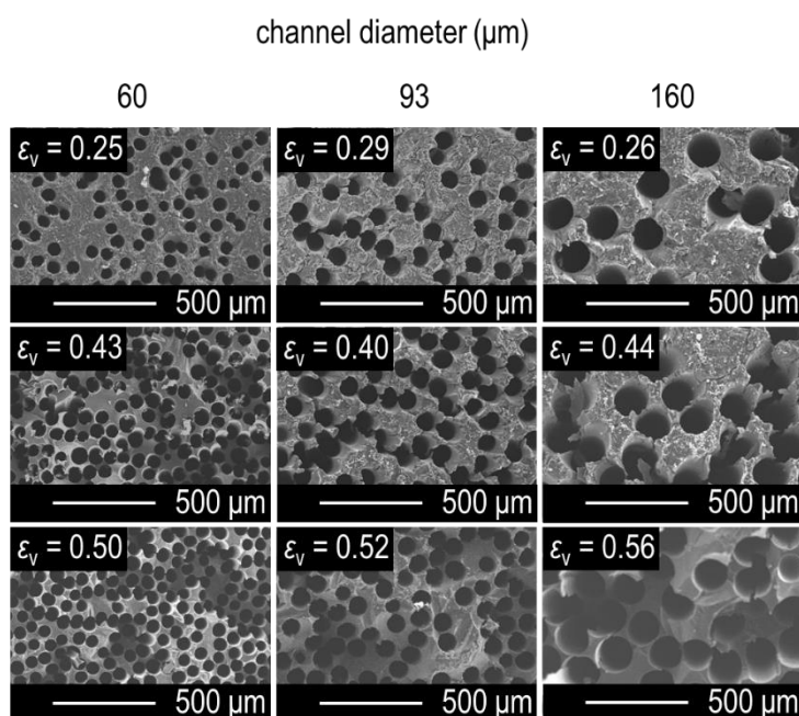
Fig. 3 Cross-sectional SEM images of FCGMs before activation, with channel sizes of 60–160 \mu\text{m} and channel densities (in the form of void fraction \epsilon_v ) of 0.25–0.56
