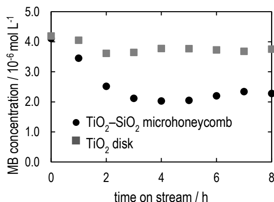
Fig. 1 Photocatalytic activity of an uncalcined TiO 2 -SiO 2 microhoneycombs and TiO 2 disk having the same total amount of TiO 2 in the decolorization of MB in continuous flow systems (feed concentration: 4 \mu\text{mol L}^{-1} , light intensity: 10 \text{W m}^{-2} , superficial velocity: 0.23 \text{cm min}^{-1} ). Conversions of MB were 0.44 and 0.10 for TiO 2 -SiO 2 microhoneycombs and TiO 2 disk, respectively.
