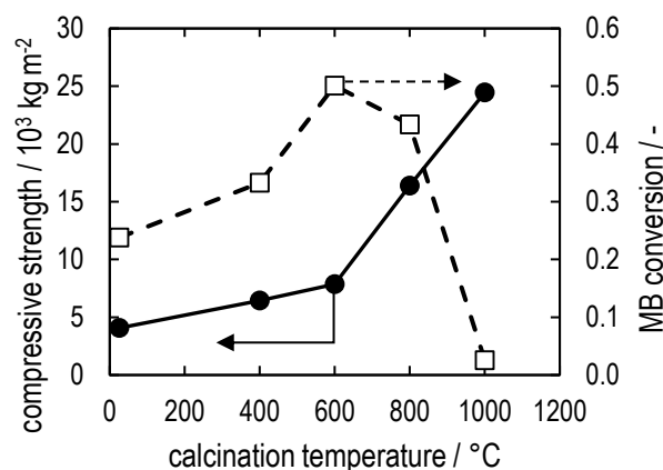
Fig. 2 Compressive strength and conversion of MB, tested using TiO 2 -SiO 2 microhoneycombs calcined at various temperatures (feed concentration: 4 \mu\text{mol L}^{-1} , light intensity: 10 \text{W m}^{-2} , superficial velocity: 0.76 \text{cm min}^{-1} , data points for uncalcined sample are shown at 25 °C).
